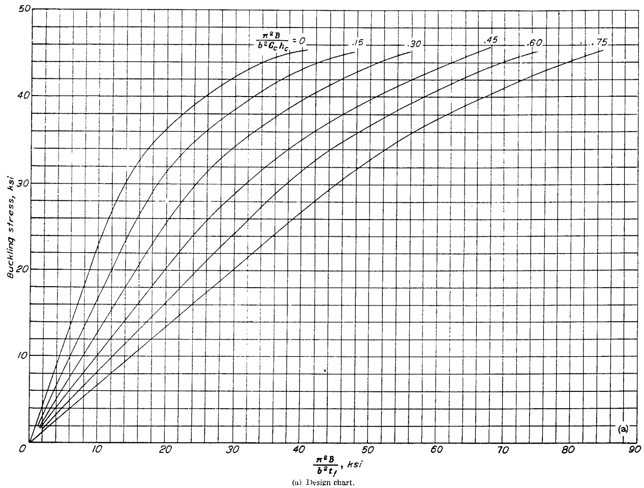
FIGURE 4.—Charts for long solid-core sandwich plates with 24S-T3 aluminum-alloy faces. \mu_f = \frac{1}{3} .
