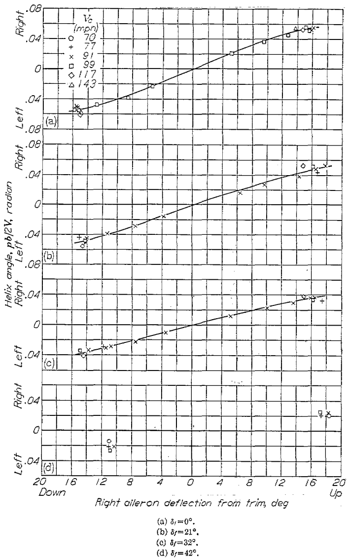
FIGURE 8.—Variation of effectiveness of flap-trailing-edge ailerons with aileron deflection at several values of flap deflection \delta_f and several values of calibrated airspeed V . Level-flight power. F2A-2 airplane.
