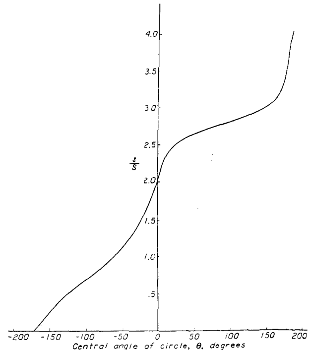
FIGURE 11.—Correspondence between points on airfoil and points on unit circle by conformal transformation.
