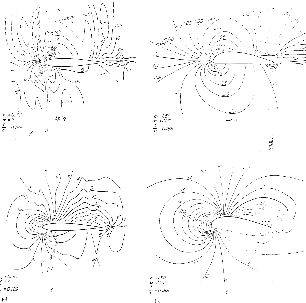
(a) RAF 30 symmetrical airfoil (reference 27). (b) Nonsymmetrical airfoil (reference 26). FIGURE 6.—Contours of equal static-pressure defect \Delta p/q and angle of flow relative to airfoil chord \xi from measurements.
