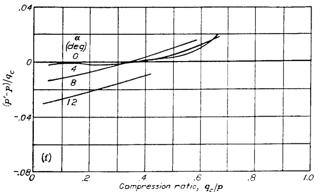
(a) Static orifices at distance x_N behind orignal nose. (c) Mounting stem at distance x_S behind static orifices. x_N=3.4D ; stem thickness D_S=0.9D . (e) Reynolds number. Reference 17. (b) Collar at distance x_C behind static orifices. D_C=1.43D ; x_N=13.8D . (d) Angle of attack for hemispherical nose. Prandtl-type tube. x_N=3D ; x_S=10D_S ; reference 22. (f) Angle of attack for semiellipsoidal nose. x_N=3.5D ; D_S=0.25D ; x_S=20D_S ; reference 23.
