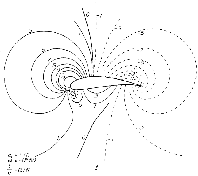
(a) Contours of equal static-pressure defect \Delta p/q and equal angle of flow relative to airfoil chord \xi . Data from reference 28. FIGURE 5.—The field of flow about a Joukowski airfoil from calculations. Variation with c_l .
