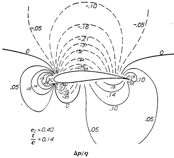
(b) Contours of equal static-pressure defect \Delta p/q . FIGURE 5.—Concluded.
