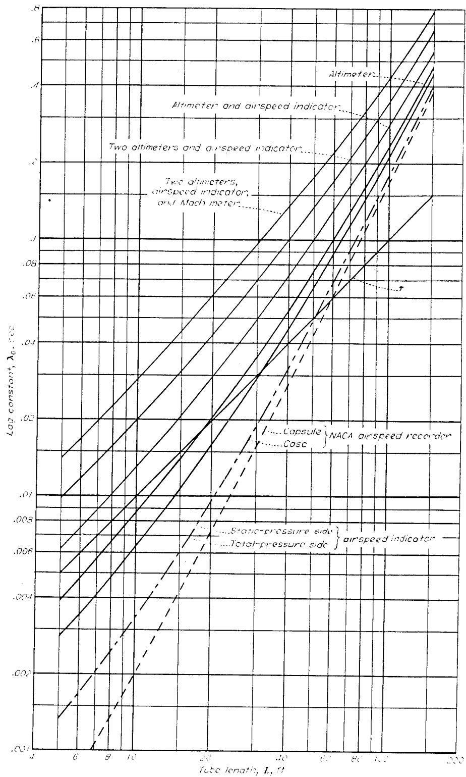
FIGURE 8.—Lag-constant variation with length of 3/16-inch inside-diameter tubing. Sea-level conditions.
