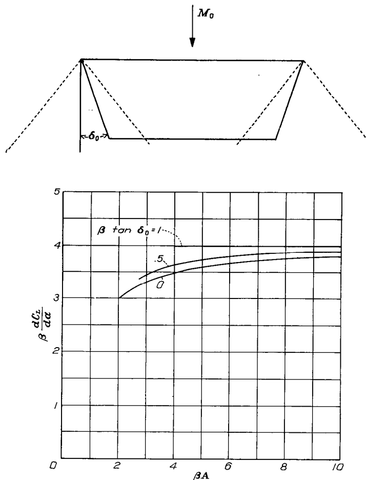
FIGURE 11. Variation of reduced lift-curve slope \beta \frac{dC_L}{d\alpha} with reduced aspect ratio \beta A for various trapezoidal plan forms.
