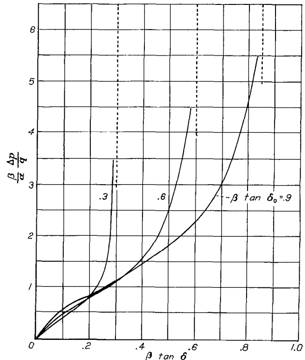
FIGURE 15.—Load distribution over triangular plan forms of type 1.
