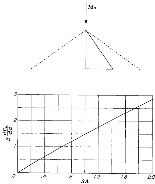
FIGURE 16.—Variation of reduced lift-curve slope \beta \frac{dC_L}{d\alpha} with reduced aspect ratio \beta A for plan forms of type 1.
