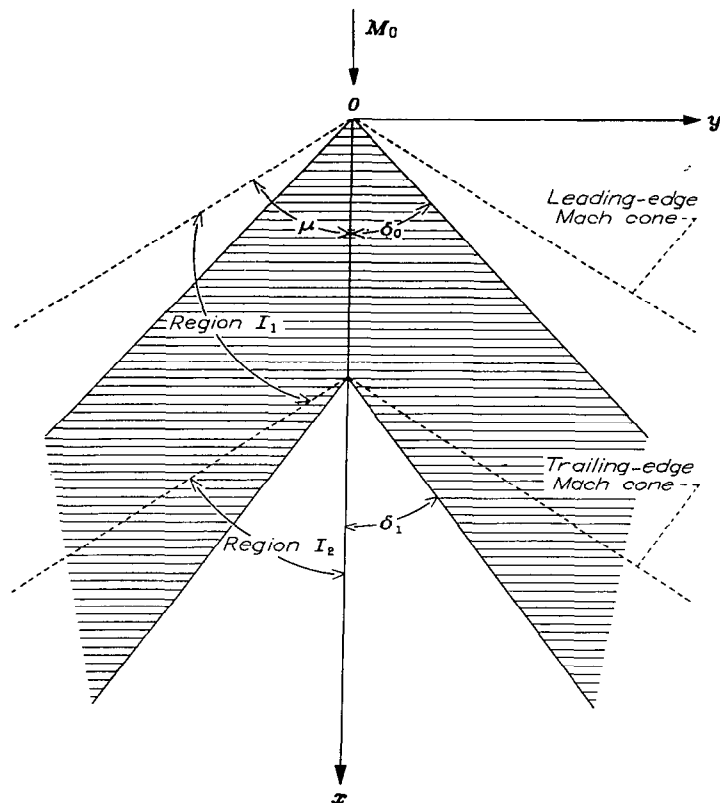
FIGURE 7.—Swept-back lifting surface with traces of Mach cones, coordinate system, and regions defined for equations (36) and (37).
