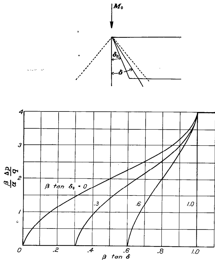
FIGURE 10.—Load distribution over tip for various trapezoidal plan forms.
