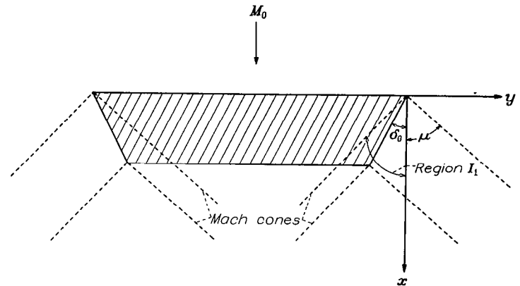
FIGURE 6.—Trapezoidal lifting surface with traces of Mach cones, coordinate system, and regions defined for equation (35).
