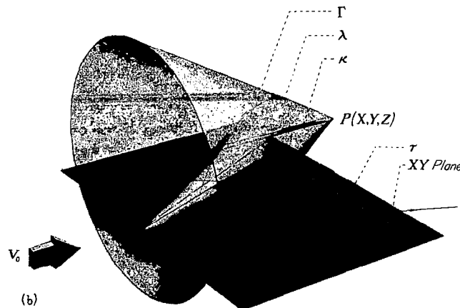
FIGURE 2.—Concluded. (b) Triangular plan form.
