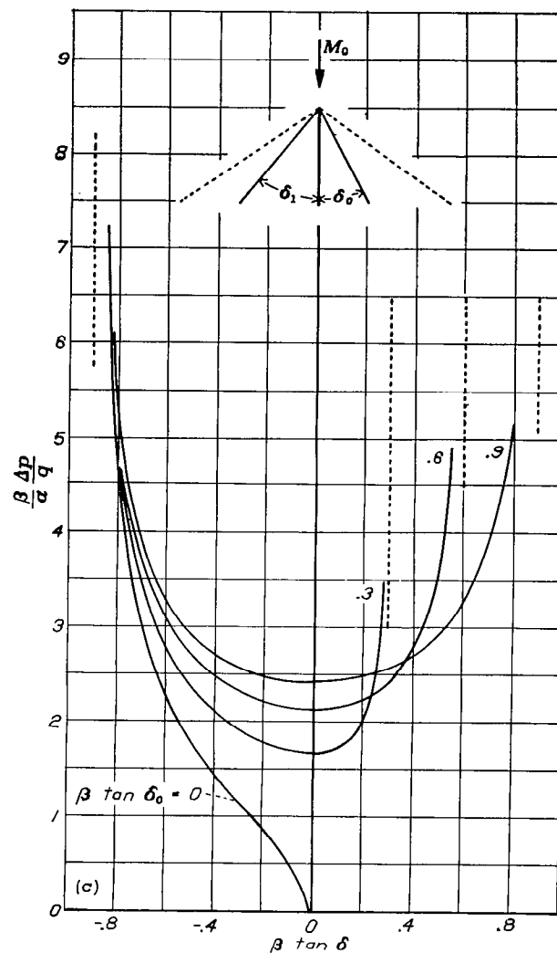
FIGURE 19.—Concluded. (c) \beta \tan \delta_1 = 0.9 .
