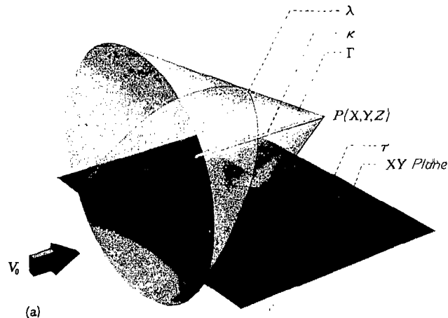
FIGURE 2.—Mach forecone from point P(X, Y, Z) intersecting surface \tau . (a) Rectangular plan form.
