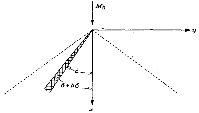
FIGURE 13.—Elemental lifting surface of constant load.
