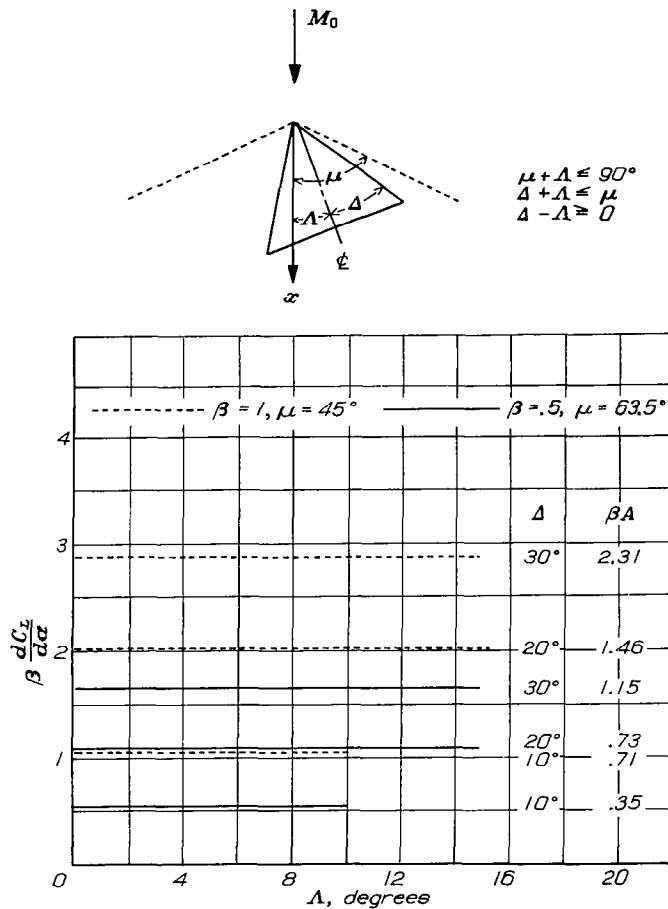
FIGURE 20.—Variation of reduced lift-curve slope \beta \frac{dC_L}{d\alpha} with angle of sideslip A for some plan forms of type 3.
