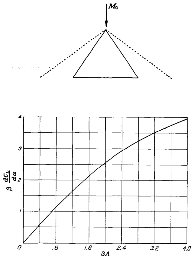
FIGURE 18.—Variation of reduced lift-curve slope \beta \frac{dC_L}{d\alpha} with reduced aspect ratio \beta A for plan forms of type 2.
