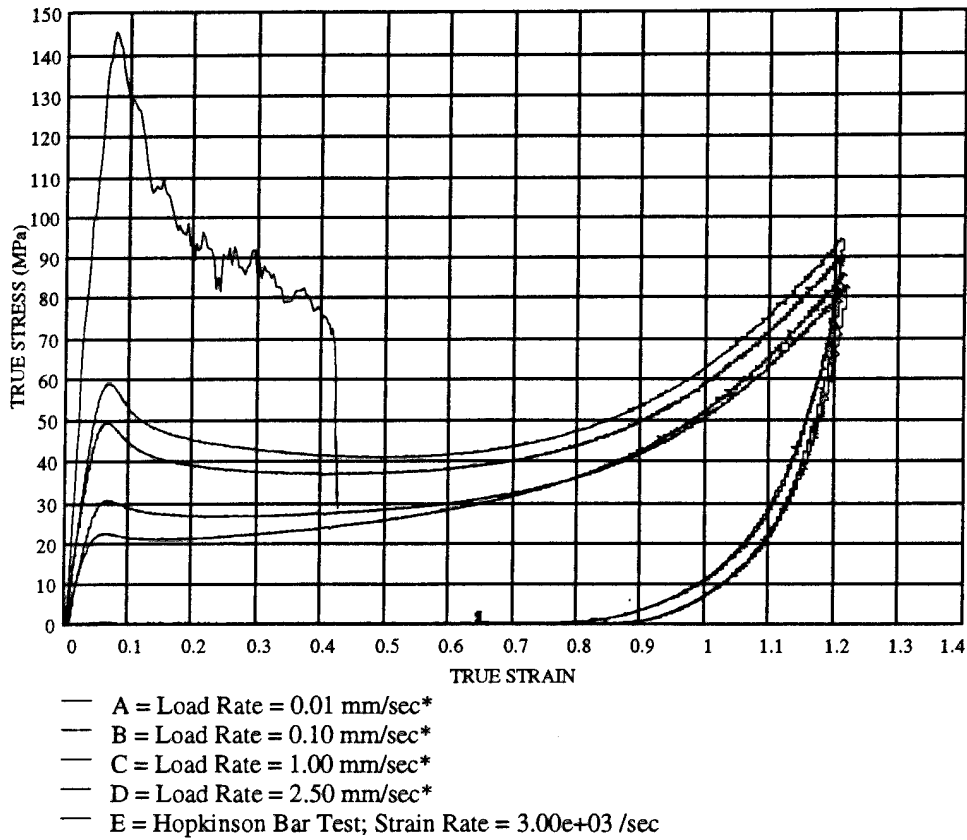
FIGURE 10-5 25% 8084 / 75% 1080 at various load rates
