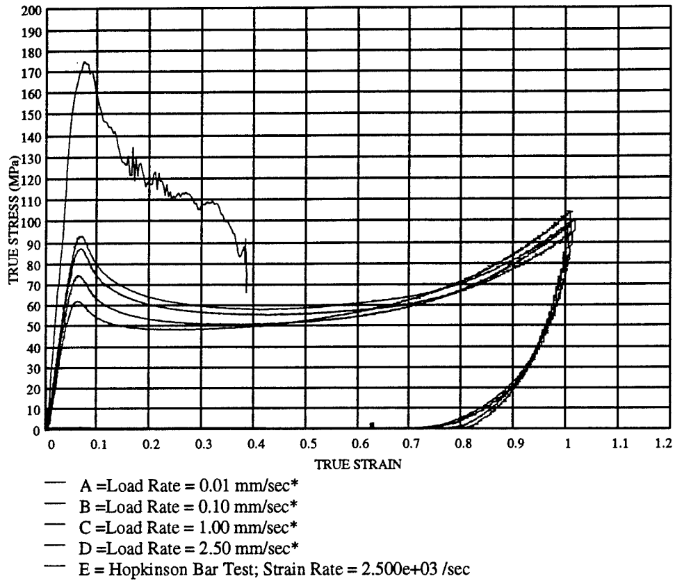
FIGURE 10-4 50% 8084 / 50% 1080 at various load rates:
