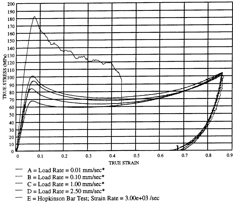
FIGURE 10-3 75% 8084 / 25% 1080 at various load rates
