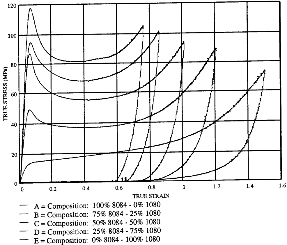
FIGURE 9-9 Plot of true stress (MPa) versus true strain for a loading rate of 1.00 mm/sec for various compositions
