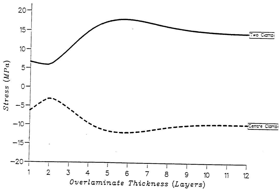
Effect of overlamine thickness on through-thickness stress in overlamine.
