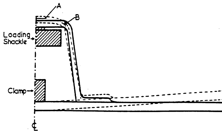
Schematic loading arrangement, centre clamped.
