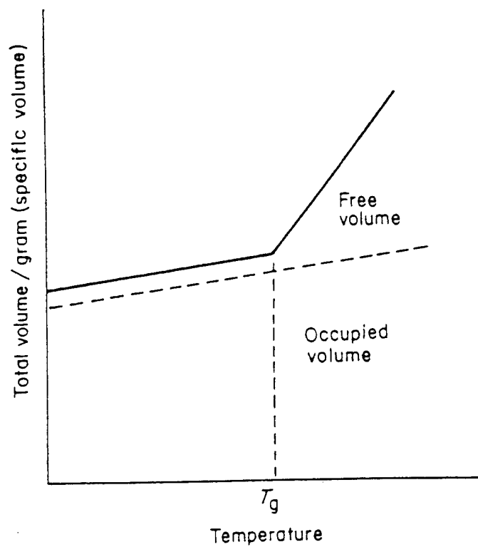
The volume-temperature relationship for a typical amorphous polymer.
