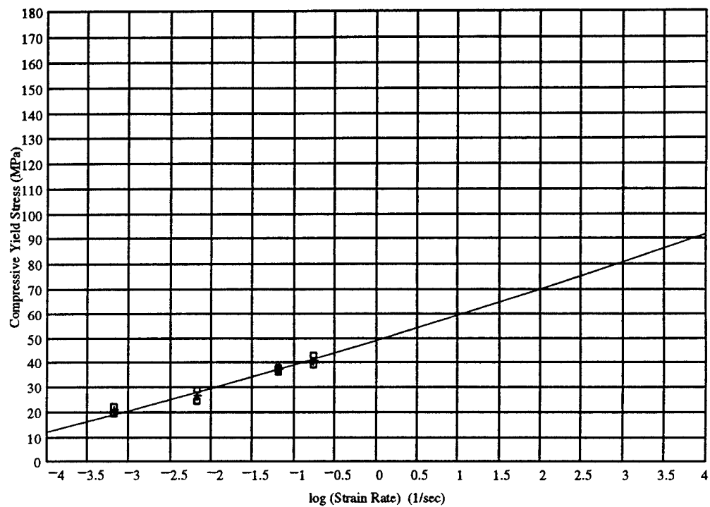
Compressive Flow Stress (MPa) versus Log(Strain Rate)(1/sec) Composition: 25% 8084, 75% 1080
