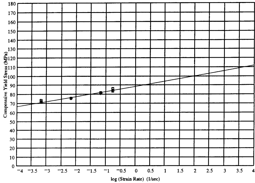
Compressive Flow Stress (MPa) versus Log(Strain Rate)(1/sec) Composition: 100% 8084, 0% 1080
