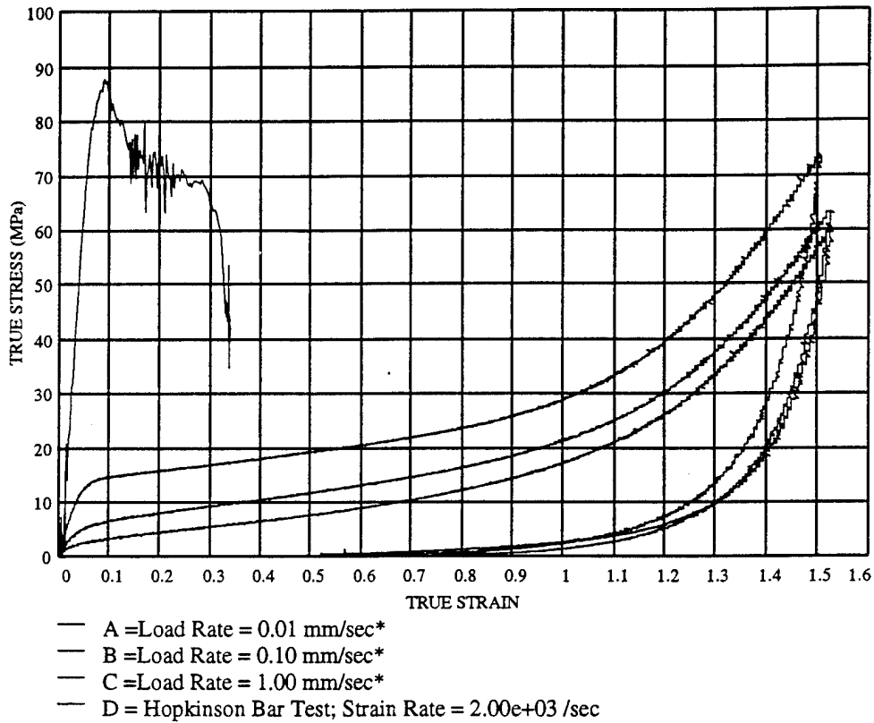
FIGURE 10-6 0% 8084 / 100% 1080 at various load rates:
