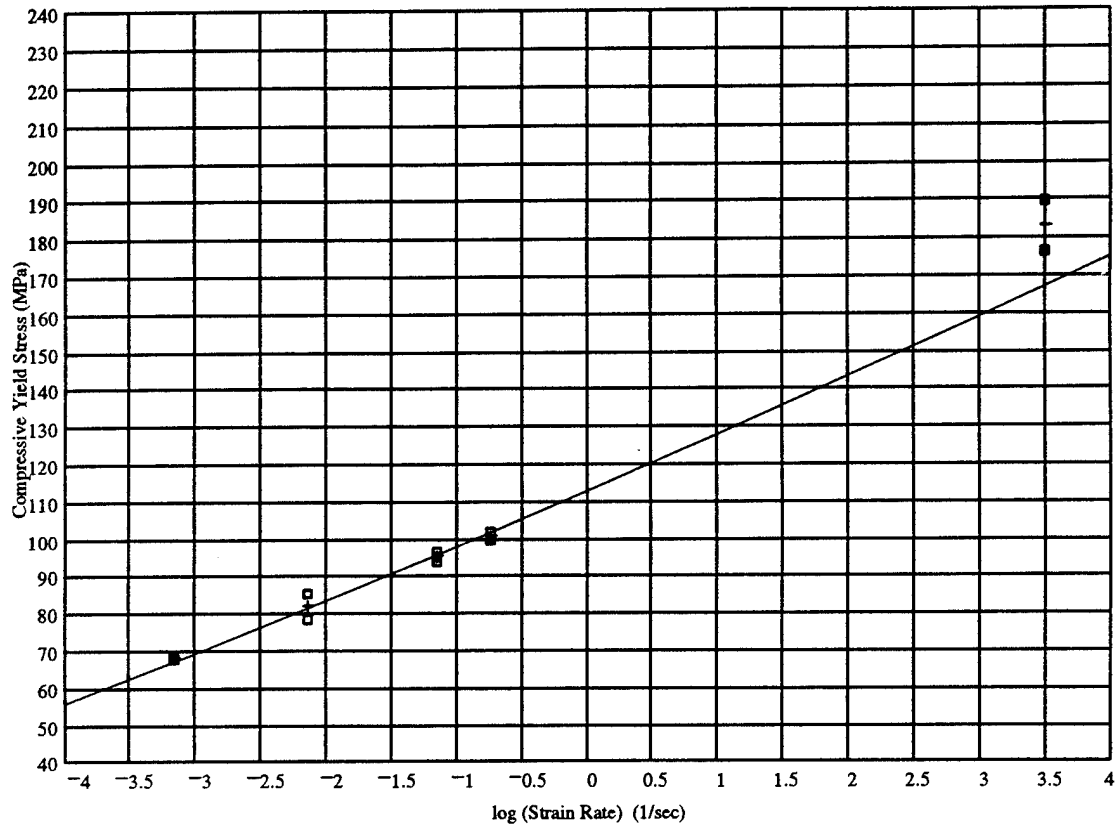
Compressive Flow Stress (MPa) versus Log(Strain Rate)(1/sec) Composition: 75% 8084, 25% 1080
