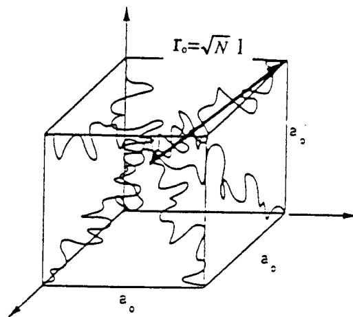
The unstretched network for the proposed eight chain model.
