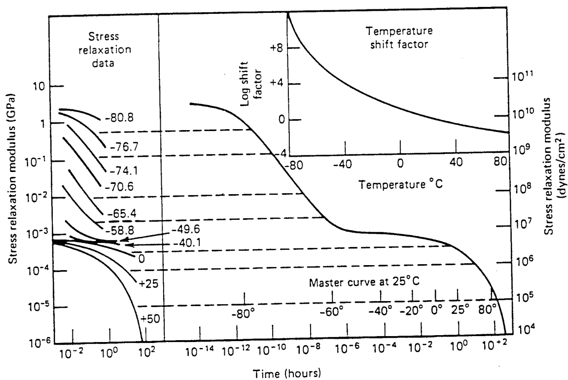
Modulus-time master plot for polyisobutylene based on time-temperature superposition of data to a reference temperature of 25°C.
