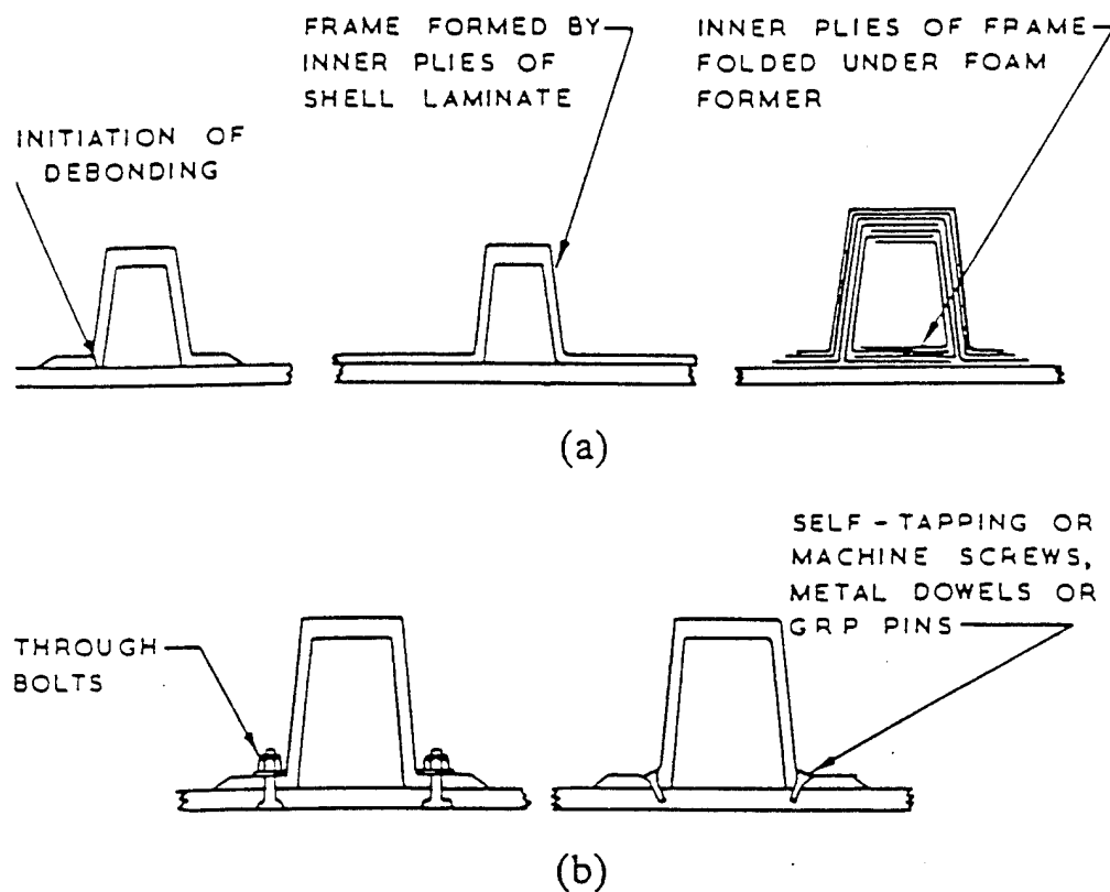
Frame/shell joints: (a) types of frame/shell attachment; (b) reinforcement of frame/shell joint.
