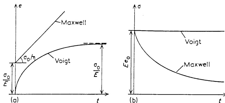
The behaviour of the Maxwell and Voigt models during different types of loading. (a) Creep (constant stress \sigma_0 ), (b) Relaxation (constant strain e_0 ) (after Williams).
