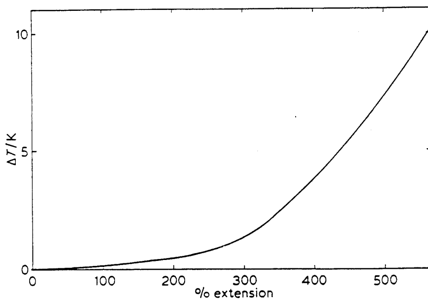
Increase in temperature, \Delta T , upon the adiabatic extension of an elastomer (vulcanized natural rubber) (data of Dart, Anthony and Guth reported by Treloar).
