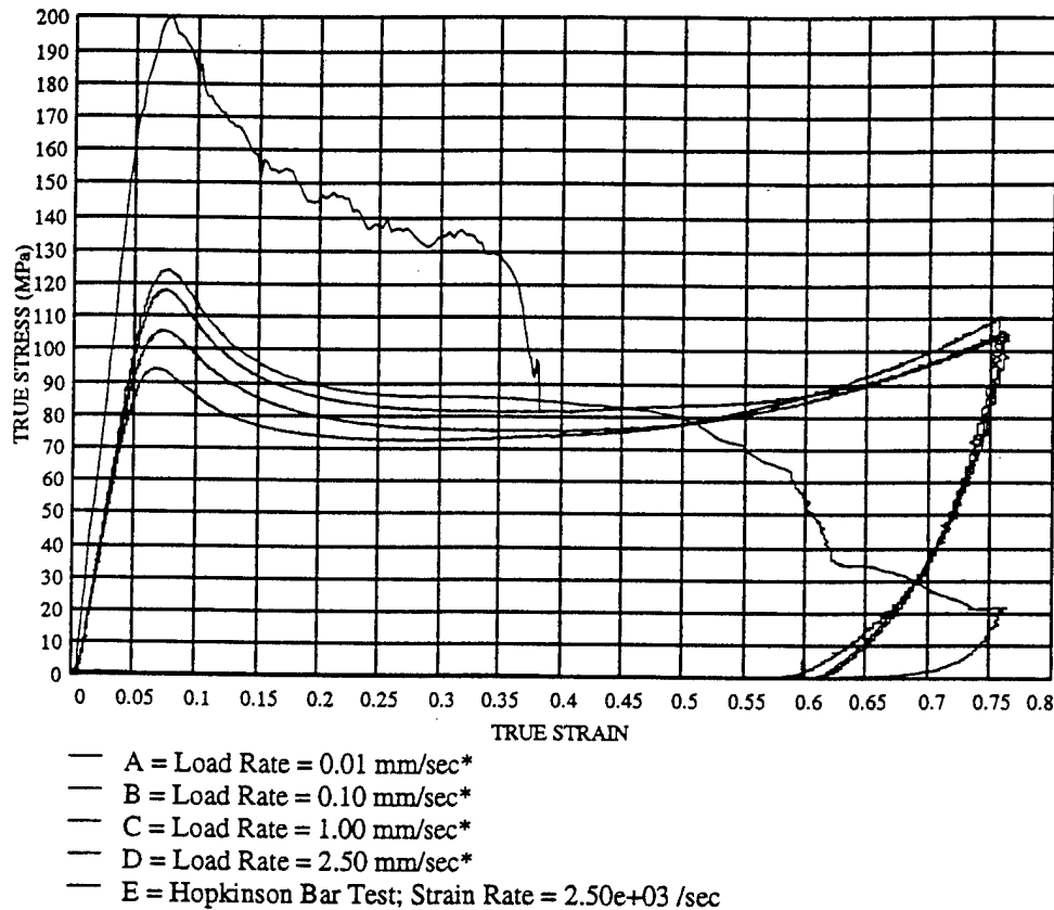
FIGURE 10-2 100% 8084 / 0% 1080 at various loads
