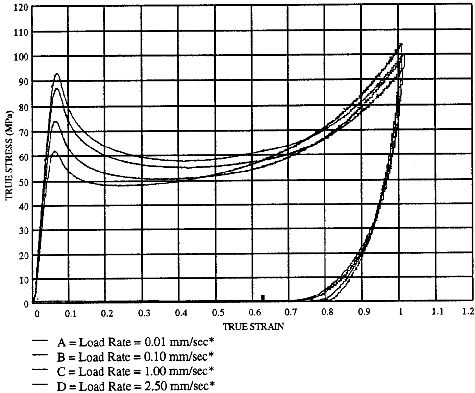
Figure 9-4 50% 8084 / 50% 1080 at various load rates
