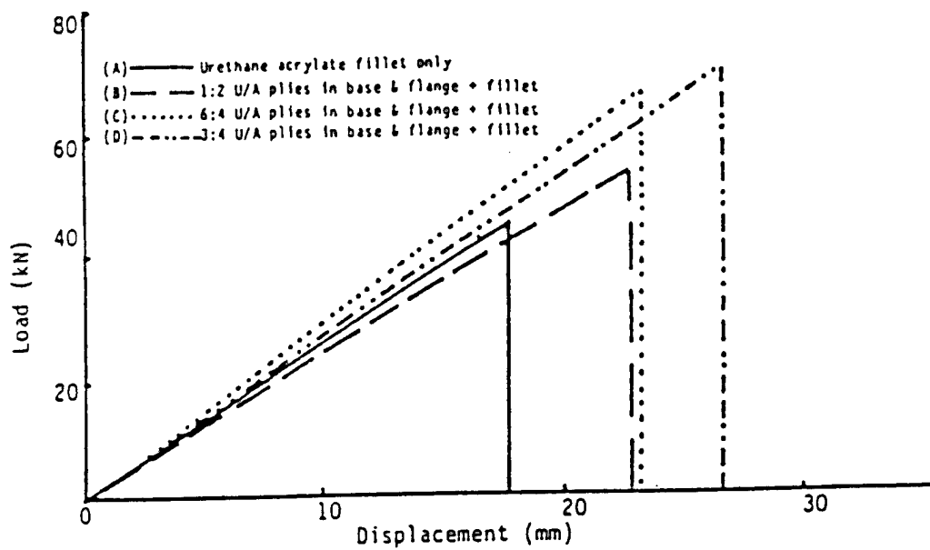
Centre clamp top hat pull off tests with different bondline conditions.
