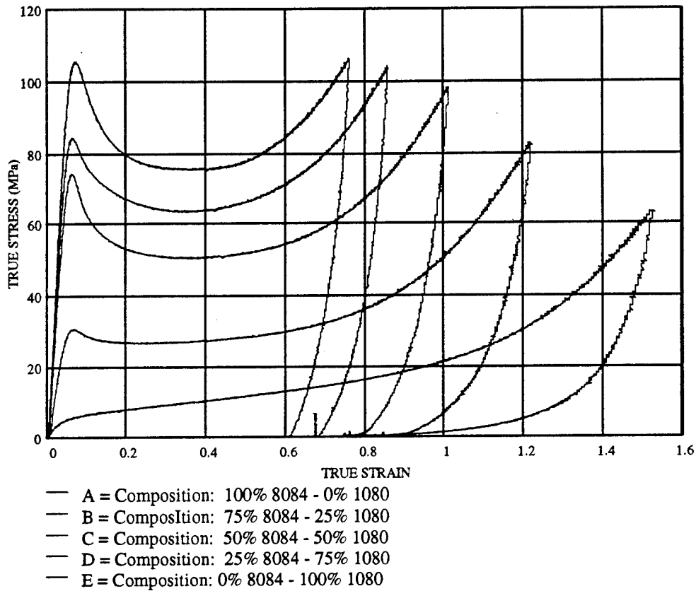
FIGURE 9-8 Plot of true stress (MPa) versus true strain for a loading rate of 0.10 mm/sec for various compositions
