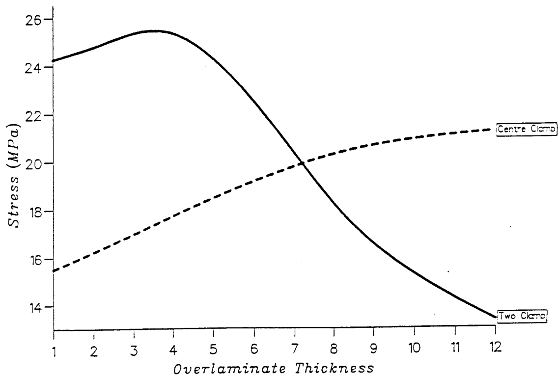
Effect of overlamine thickness on stress in fillet.
