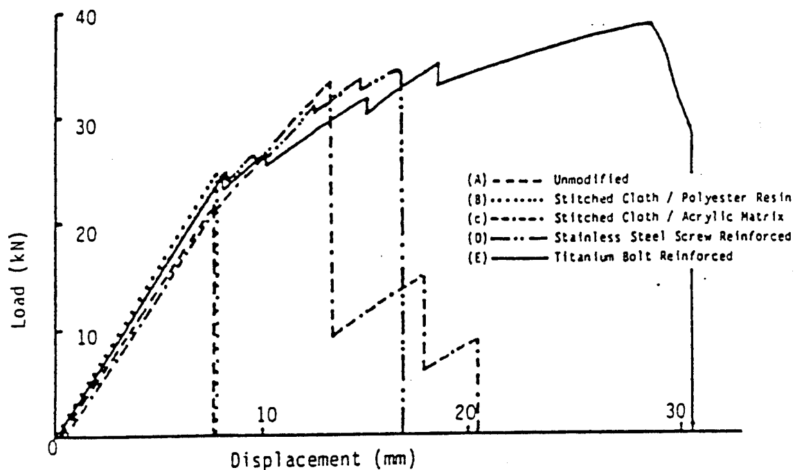
Centre clamp top hat pull off tests.
