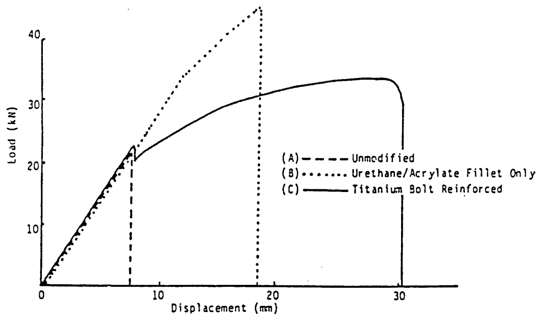
Centre clamp top hat pull off tests, comparing standard bondlines with the adopted urethane acrylate system.
