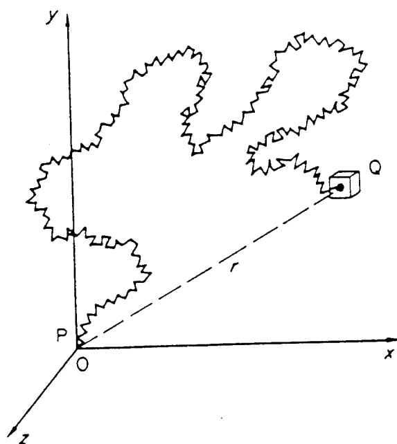
Freely jointed chain made of (N) identical links, each of length (l) .
