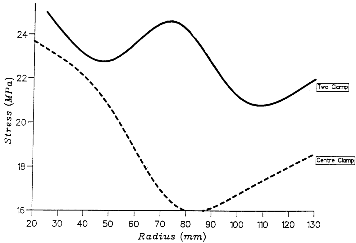
Effect of radius on stress in fillet.
