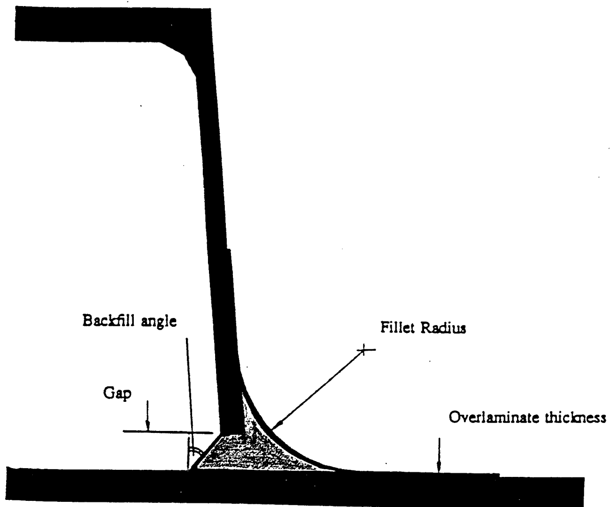
Design variations considered for top-hat stiffeners.
