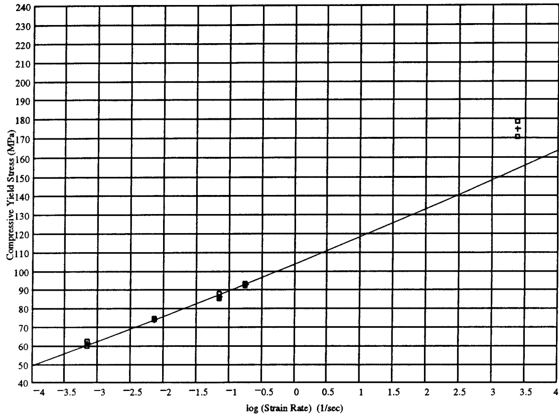
Compressive Flow Stress (MPa) versus Log(Strain Rate)(1/sec) Composition: 50% 8084, 50% 1080
