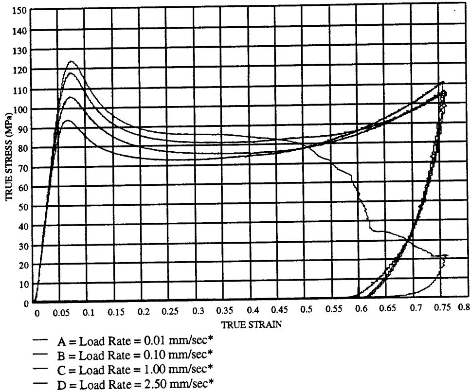
Figure 9-2 100% 8084 / 0% 1080 at various load rates
