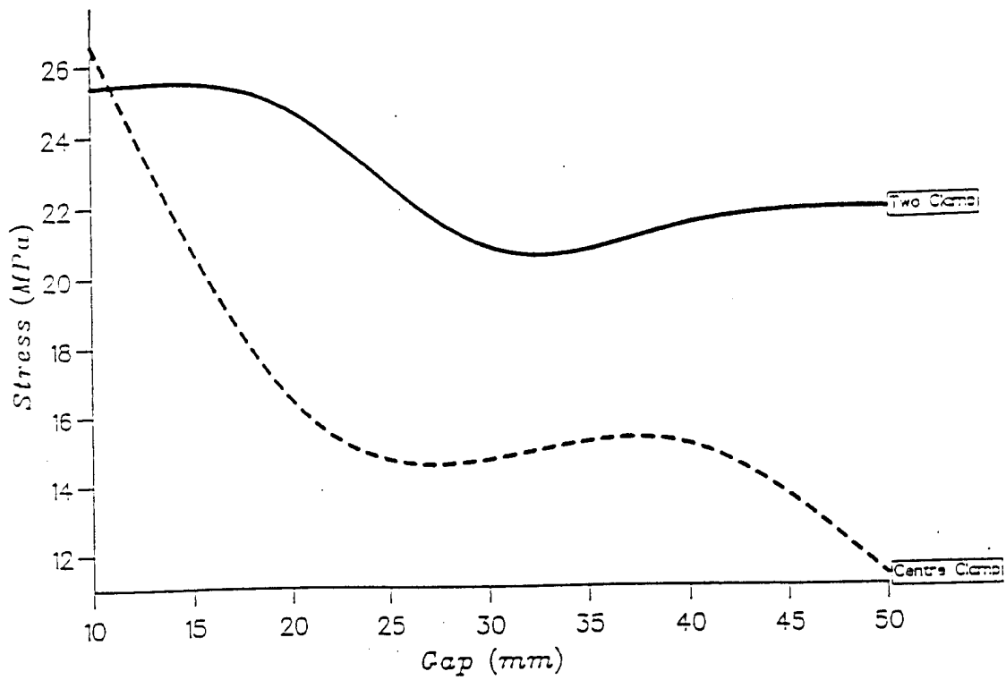
Effect of gap on stress in fillet.
