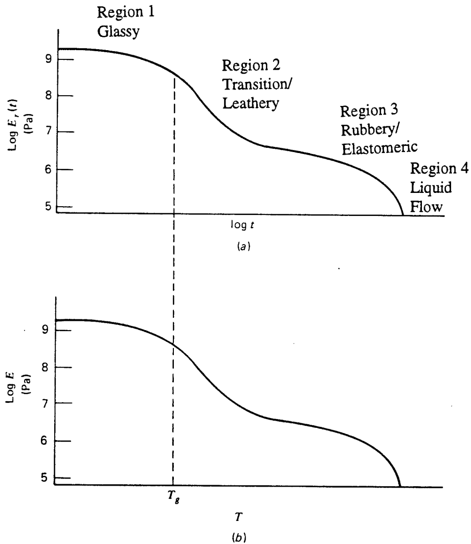
Time-temperature dependence of elastic modulus in thermoplastic polymeric solids: (a) change in relaxation modulus E_r(t) as function of time; (b) change in tensile modulus as function of temperature.
