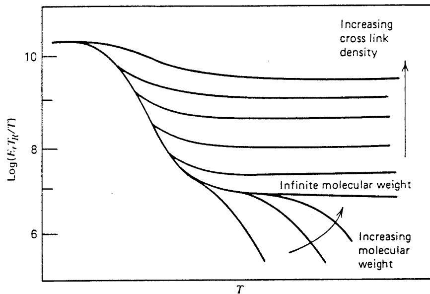
Effect of molecular weight and degree of cross-linking on relaxation modulus.
