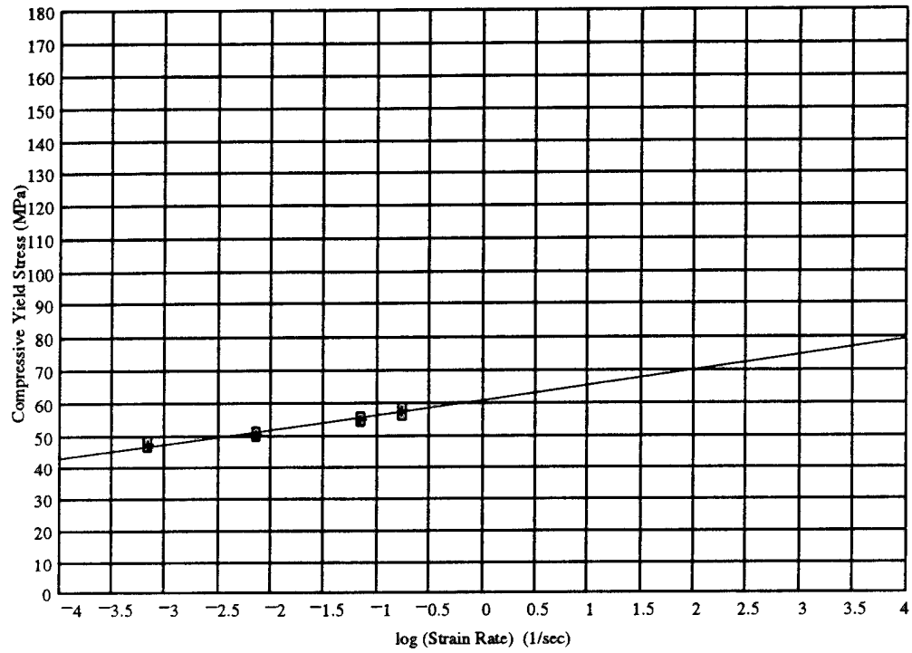
Compressive Flow Stress (MPa) versus Log(Strain Rate)(1/sec) Composition: 50% 8084, 50% 1080
