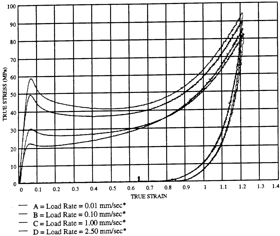
Figure 9-5 25% 8084 / 75% 1080 at various load rates
