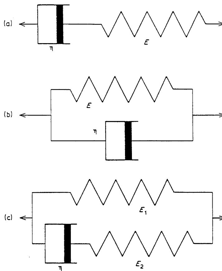
Mechanical models used to represent the viscoelastic behaviour of polymers. (a) Maxwell model, (b) Voigt model, (c) Standard linear solid.
