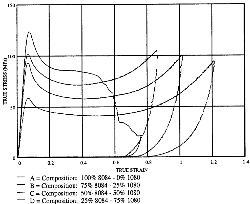
FIGURE 9-10 Plot of true stress (MPa) versus true strain for a loading rate of 2.50 mm/sec for various compositions
