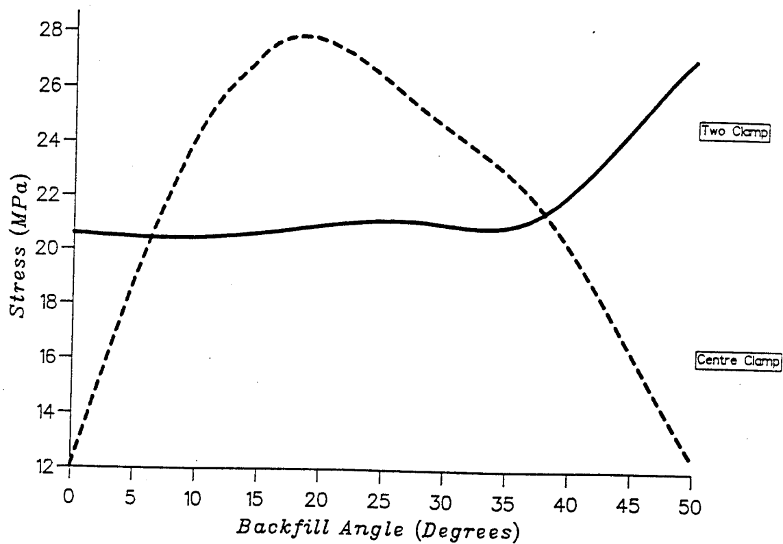
Effect of backfill angle on stress in fillet.
