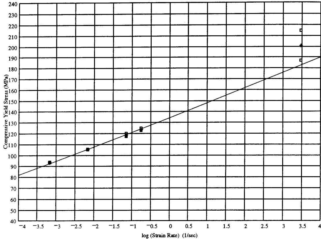
Compressive Flow Stress (MPa) versus Log(Strain Rate)(1/sec) Composition: 100% 8084, 0% 1080
