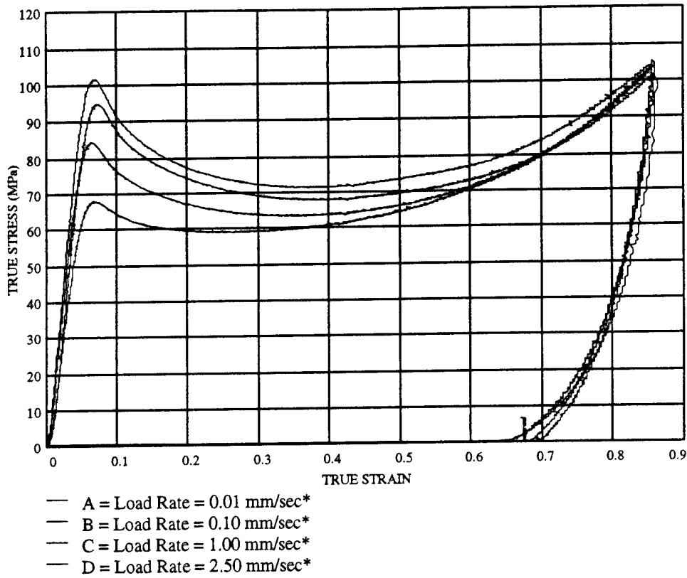
Figure 9-3 75% 8084 / 25% 1080 at various load rates
