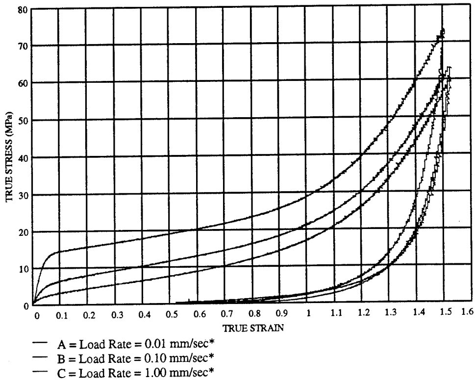
Figure 9-6 0% 8084 / 100% 1080 at various load rates
