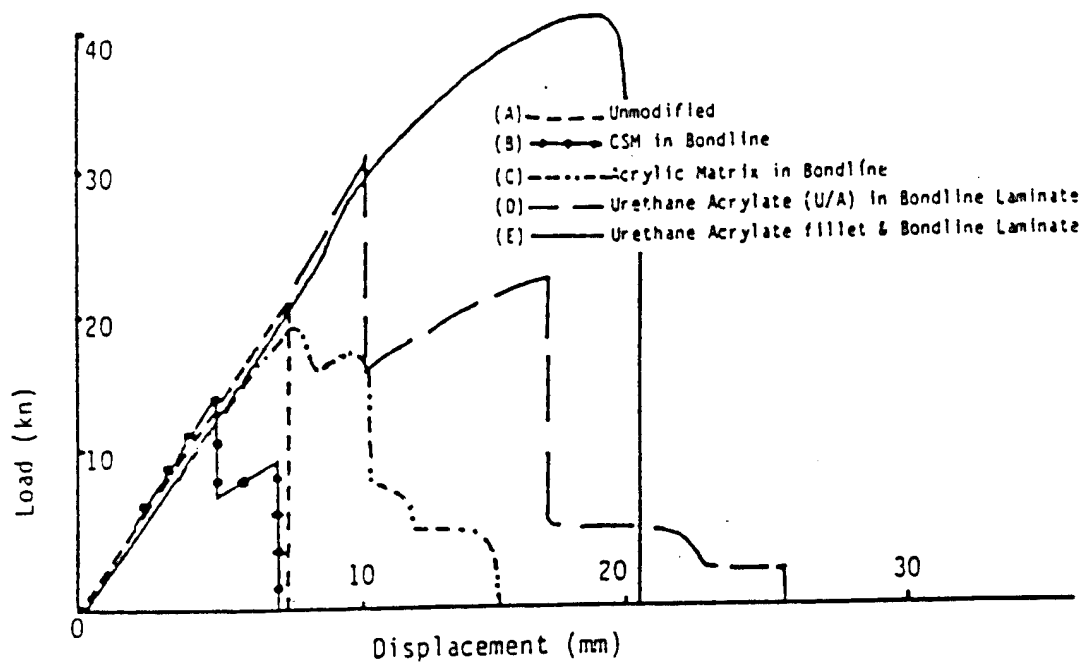
Centre clamp top hat pull off tests.
