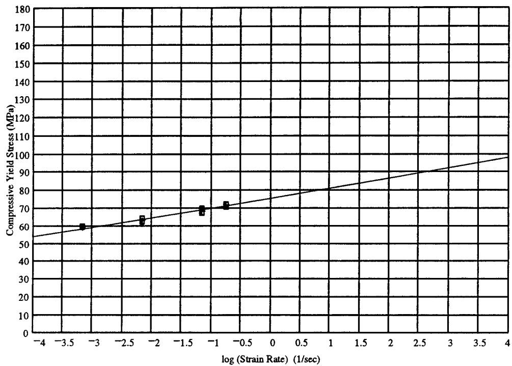
Compressive Flow Stress (MPa) versus Log(Strain Rate)(1/sec) Composition: 75% 8084, 25% 1080
