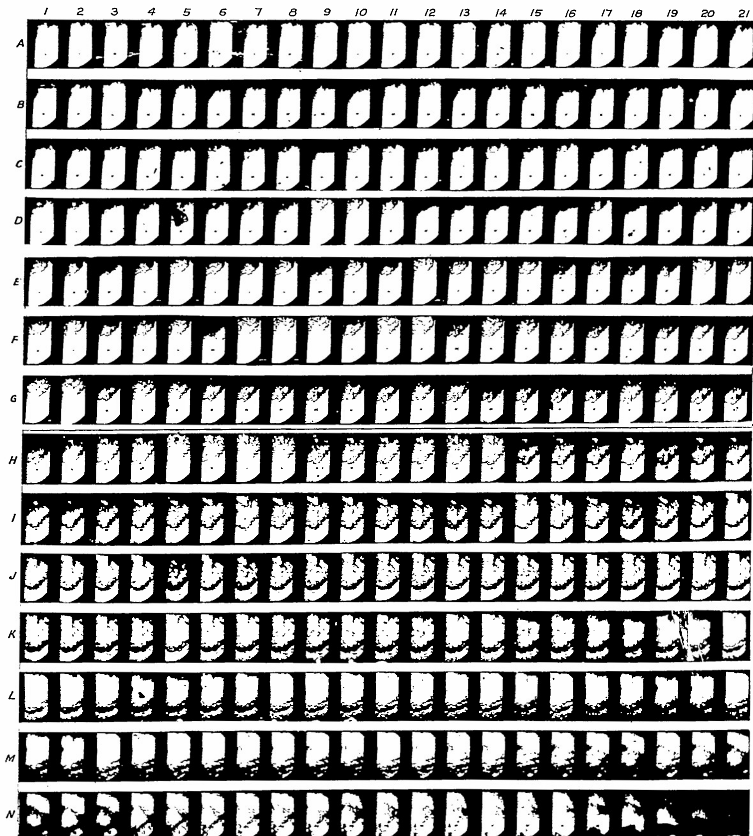
FIGURE 13.—High-speed motion pictures of combustion cycle in an engine cylinder showing antokignition before knock. S-2 fuel plus 400 ml amyl nitrate per gallon.
