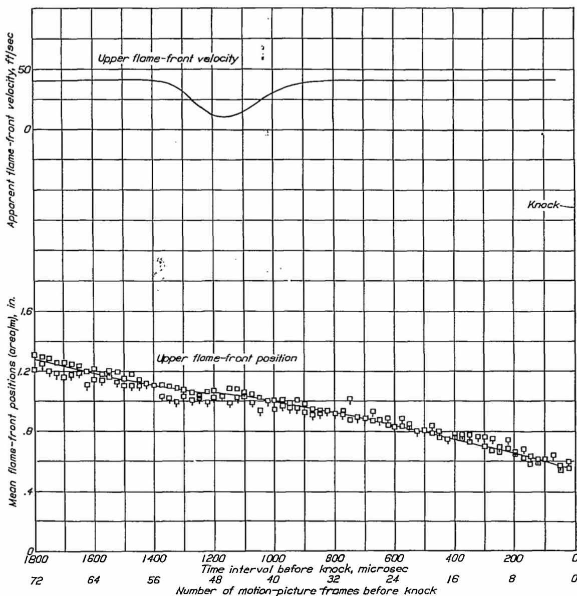
FIGURE 12.—Flame travel in an engine cylinder during knocking combustion as affected by the addition of 200 ml amyl nitrate per gallon of S-1 fuel (from fig. 11). (Tailed symbols represent check points.)
