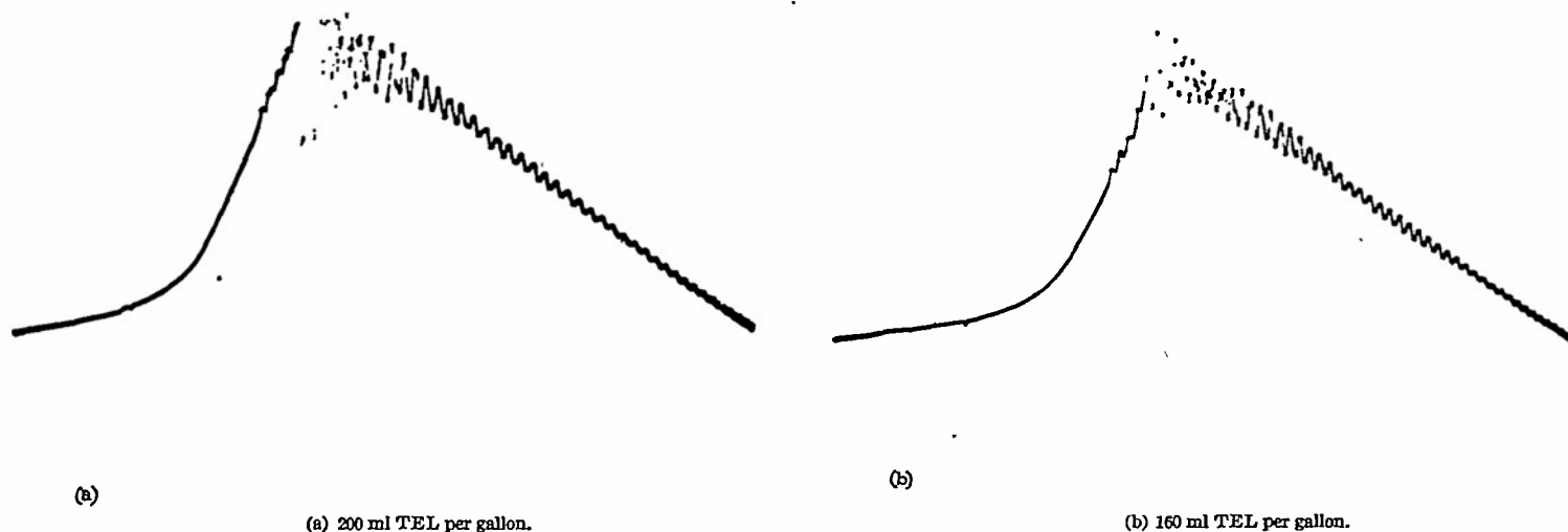
FIGURE 10.—Pressure-time records of combustion cycles showing irregular preknock vibrations. Fuel, M-3.
