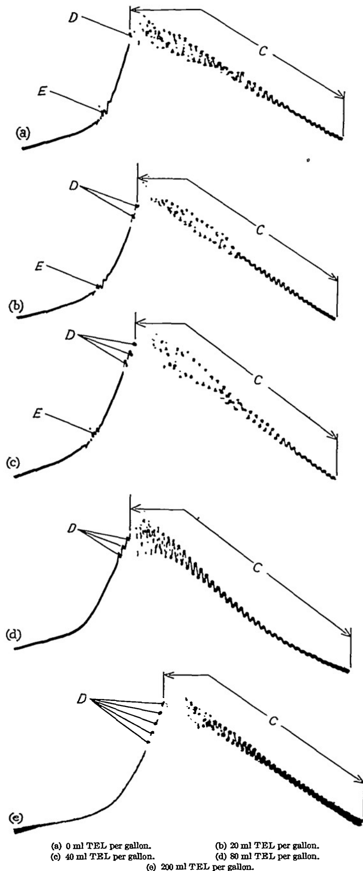
FIGURE 8.—Effect of tetraethyl-lead concentration on preknock vibrations in combustion cycles using M-3 fuel. C, knocking vibrations; D, preknock vibrations; E, timing impulses.
