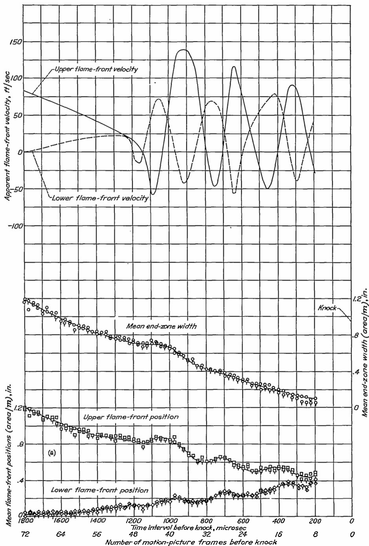
FIGURE 4.—Effect of explosive preknock reaction on travel of flame fronts in an engine cylinder. Fuel, M-2. (Tailed symbols represent check points.)
