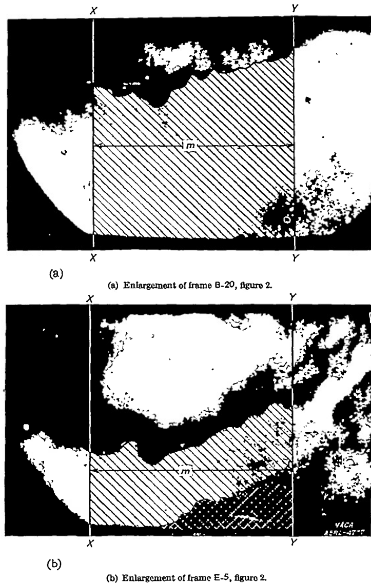
FIGURE 3.—Diagram showing areas to be measured in computing mean flame-front velocities for combustion cycle shown in figure 2.
