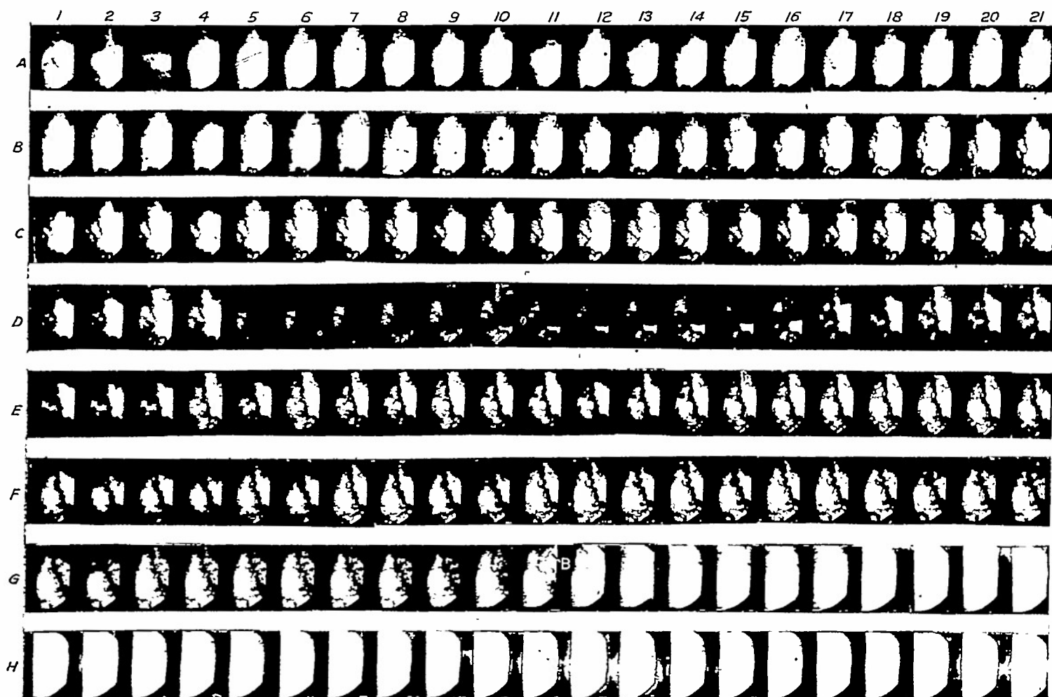
FIGURE 11.—High-speed motion pictures of combustion cycle in an engine cylinder showing autoignition before knock. S-1 fuel plus 200 ml amyl nitrate per gallon. B, blurring caused by knock. (See fig. 12.)
