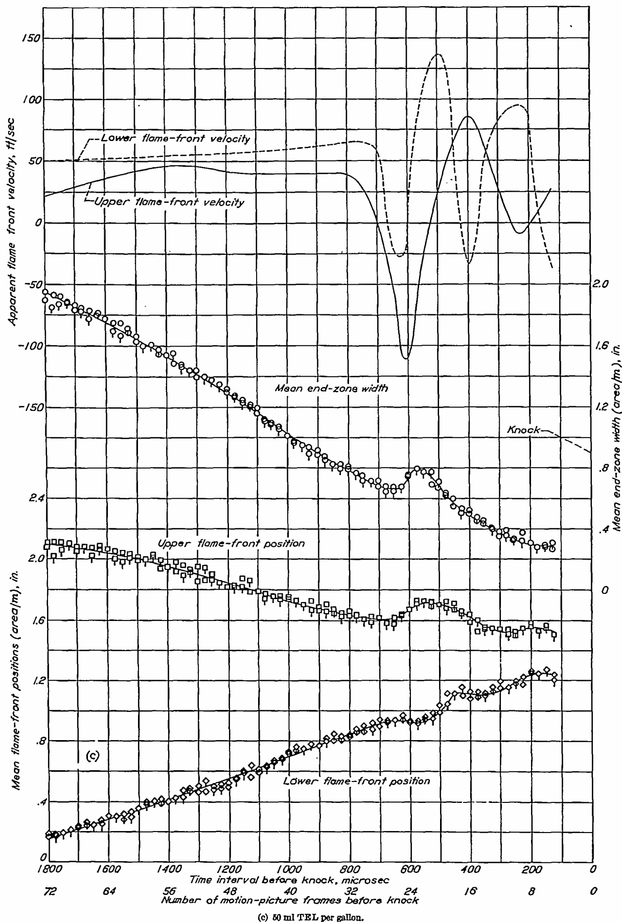
FIGURE 4.—Continued. Effect of explosive preknock reaction on travel of flame fronts in an engine cylinder. Fuel, M-2. (Tailed symbols represent check points.)
