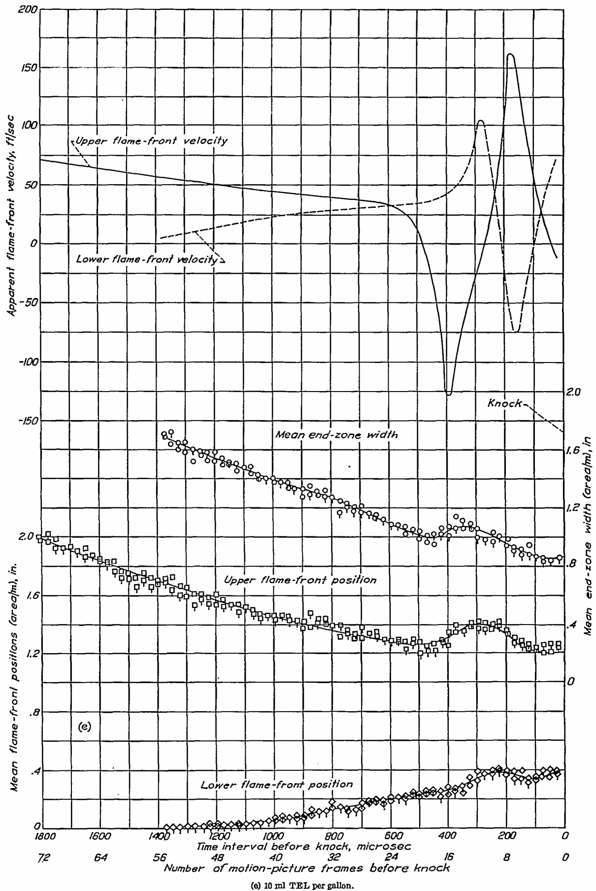
FIGURE 4.—Concluded. Effect of explosive preknock reaction on travel of flame fronts in an engine cylinder. Fuel, M-2. (Tailed symbols represent check points.)
