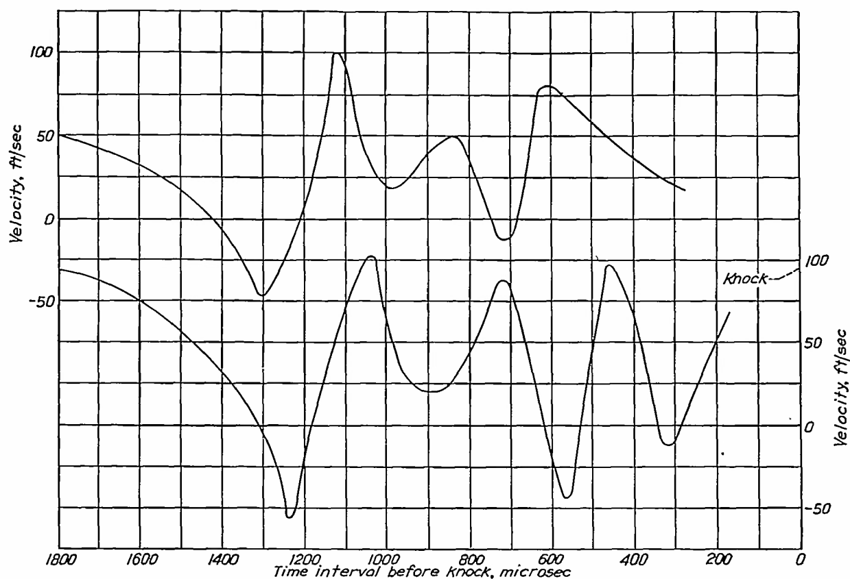
FIGURE 9.—Apparent upper-flame-front velocities in an engine cylinder showing measured irregularities in flame-front progression. M-2 fuel plus 200 ml TEL per gallon.
