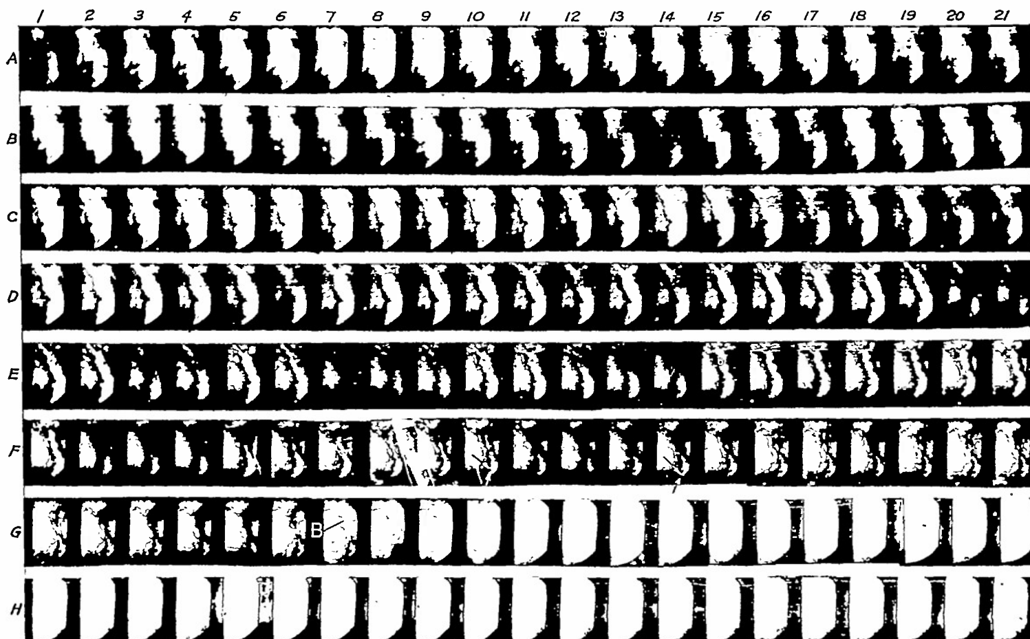
FIGURE 2.—High-speed motion pictures of vibratory combustion cycle in an engine cylinder. M-2 fuel plus 200 ml TEL per gallon. B, blurring caused by knock. (See fig. 4 (a).)
