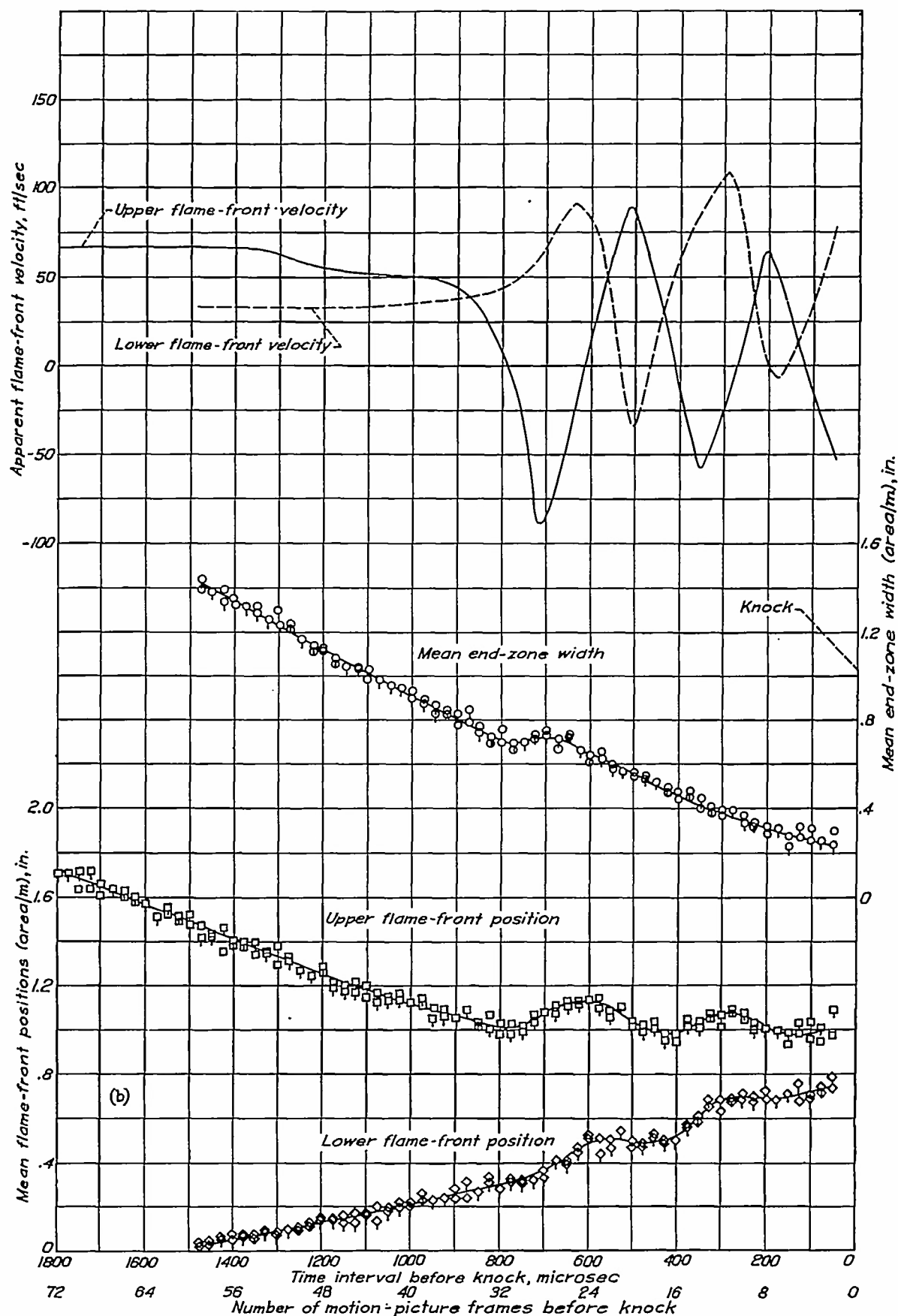
FIGURE 4.—Continued. Effect of explosive preknock reaction on travel of flame fronts in an engine cylinder. Fuel, M-2. (Tallied symbols represent check points.)
