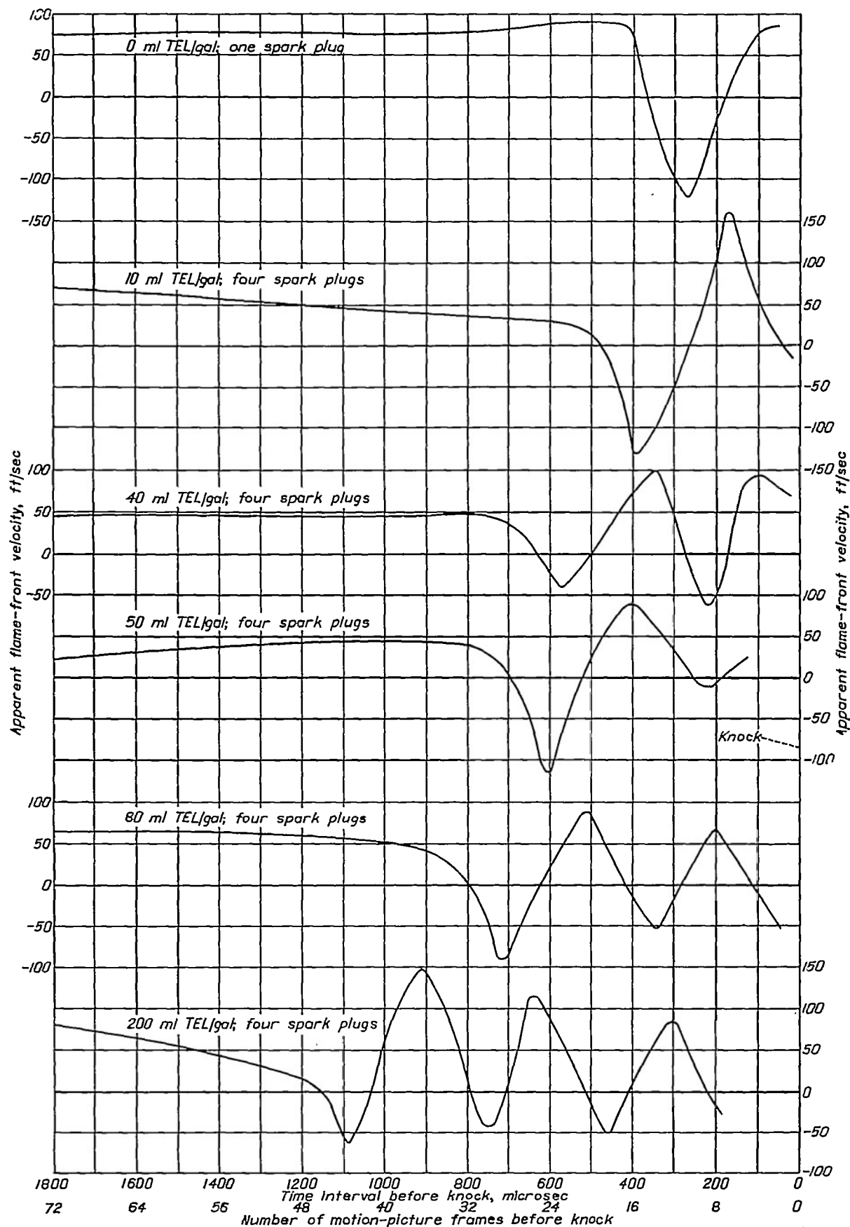
FIGURE 6.—Apparent upper-flame-front velocities in an engine cylinder as affected by preknock explosive reaction. Fuel, M-2.
