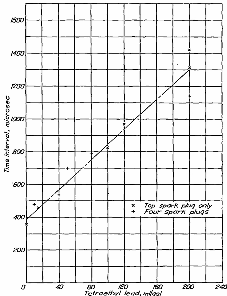
FIGURE 7.—Effect of tetraethyl-lead concentration in M-2 fuel on time interval between preknock explosive reaction and knock in an engine cylinder.
