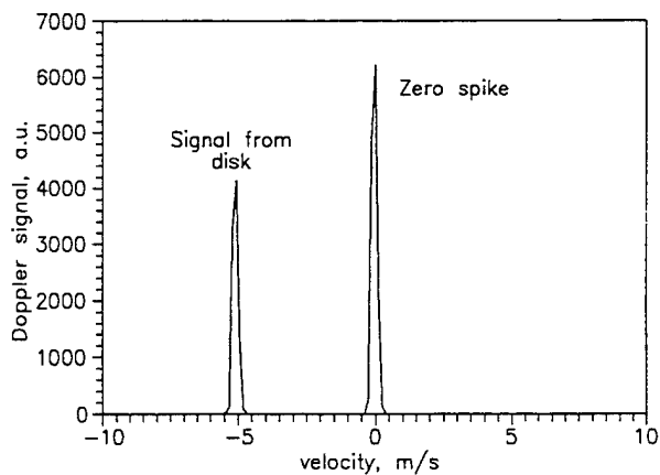
Fig 2. Doppler spectrum for rotating disk.
