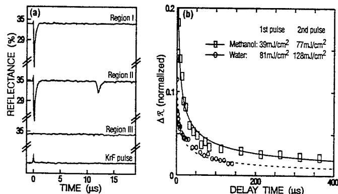
Fig. 3. (a) The optical reflectance signal for the three regions shown Fig 2(a) confirming the existence of a memory effect at the laser-irradiated area. (b) The echo signal peak amplitude as a function of delay time between the laser pulse and the acoustic pulse (temporal decay of the memory effect) for liquid-chromium interface. The lines represent the fit of the experimental data with the diffusion model.
