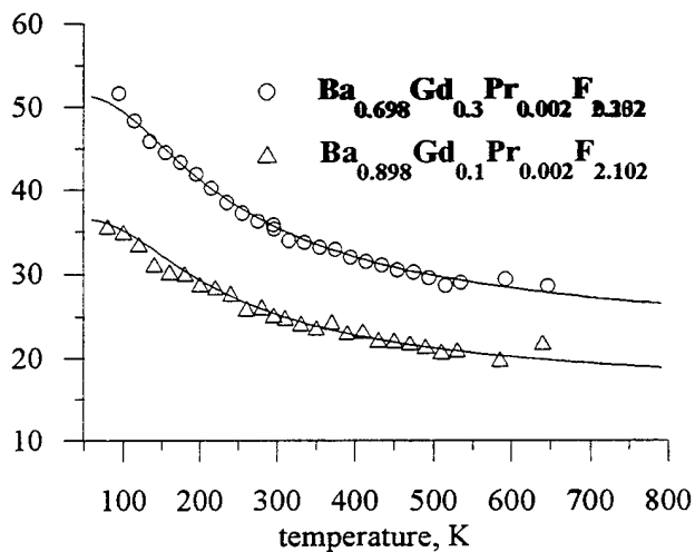
Fig. 8. Temperature dependence of integral abs. coefficient of 3P_2-3P_0 group of lines
