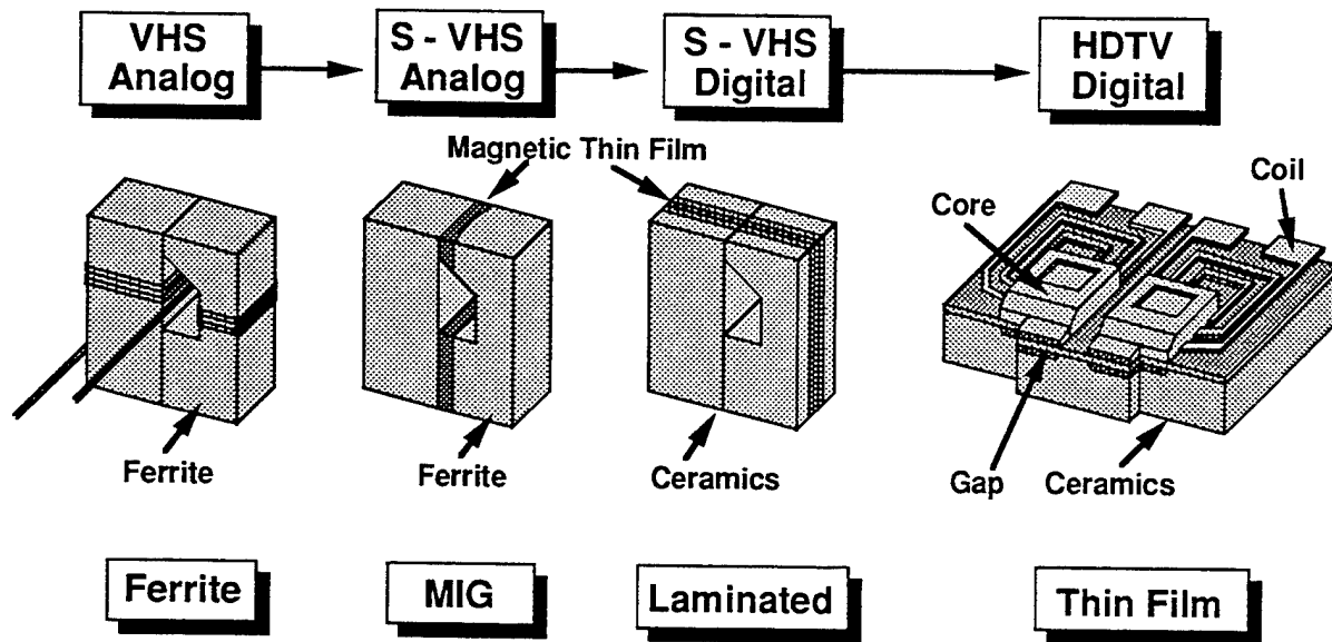
Fig. 1 A trend of video tape recorder (VTR) recording heads.
