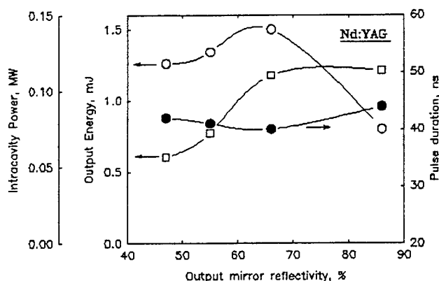
Fig. 11. Single pulse output energy \circ , pulse duration \bullet and intracavity power \square versus output mirror reflectivity of Nd:YAG laser with V^{3+} :YAG.
