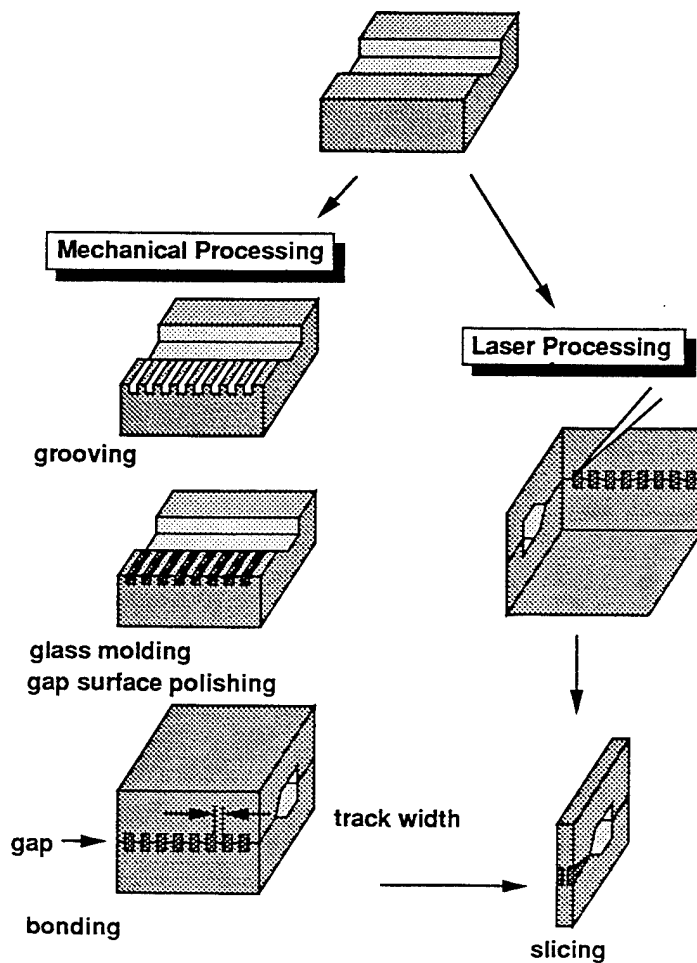
Fig. 2 A comparison of magnetic head fabrication processes between a conventional mechanical and laser processing.
