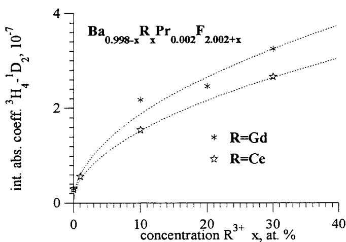
Fig. 7. Integral absorption coefficient of 1D_2 bands versus R^{3+} concentration
