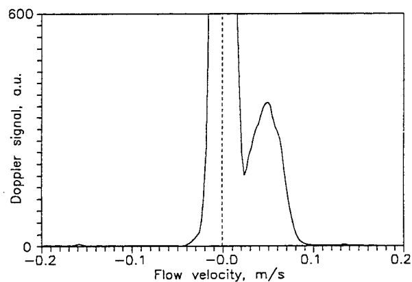
Fig 3a. Doppler spectrum for water target. Thermocapillary convection.
