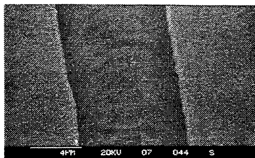
Fig. 9 A top SEM view of a laser etched groove in ITO on a glass substrate. A frequency doubled Nd:YLF laser with a pulse duration of 6 ns at an energy density of 7.7\text{ J/cm}^2 was scanned at 2.4\text{ mm/s} with a pulse repetition rate of 3 kHz.
