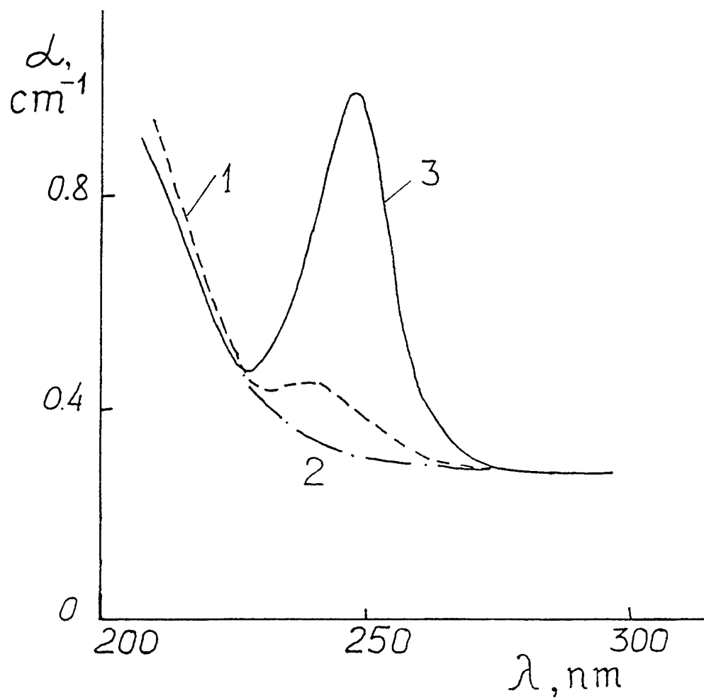
Fig.2. Absorption spectra of initial electrofused silica glass KI ( 1 ) and of samples synthesized by LAD in air ( 2 ) and in \text{N}_2 ( 3 ).
