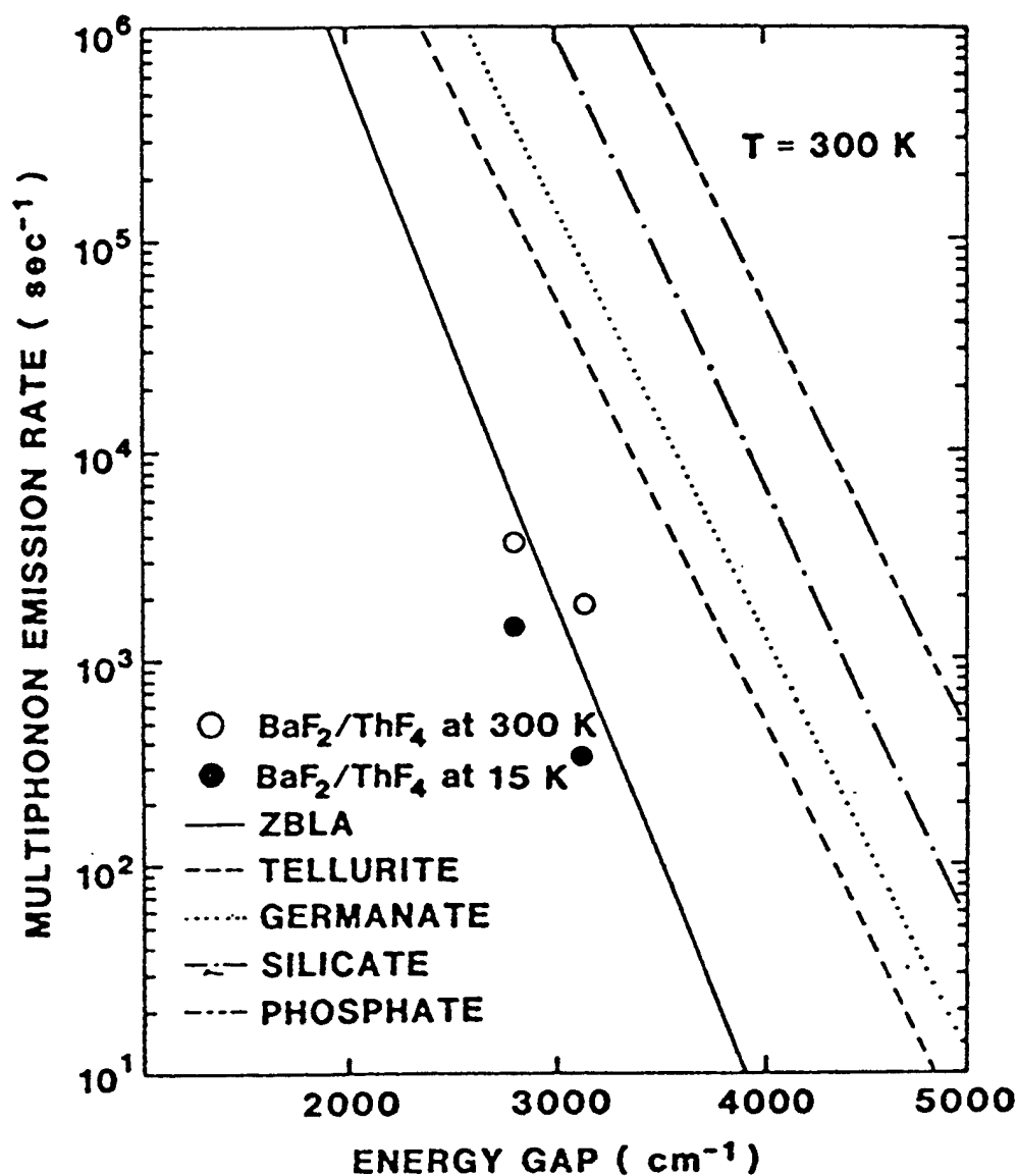
Fig. 1. Multiphonon emission rates of \text{Er}^{3+} in various materials at 300K as a function of the energy gap to the next lower level. 8
