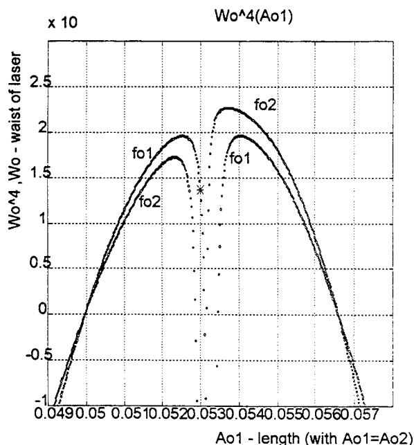
Fig. 7. Region of laser stable operation for lens with fo1 = 10 m and with fo2 = 0.02 m.
