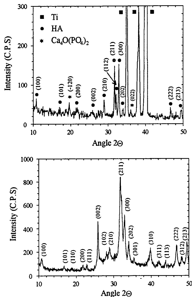
Fig.2. XRD spectra of : a) HA film deposited on Ti substrate ( in mix of Ar/H 2 O vapors, T d = 600°C, E T = 3 Jcm -2 , film thickness 240 nm), b) target
