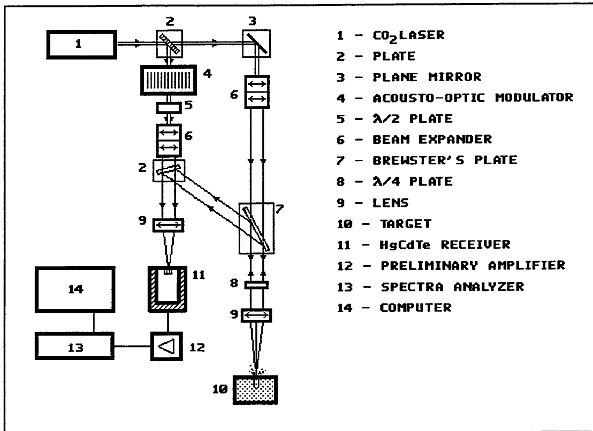
FIG. 1. EXPERIMENTAL SETUP.
