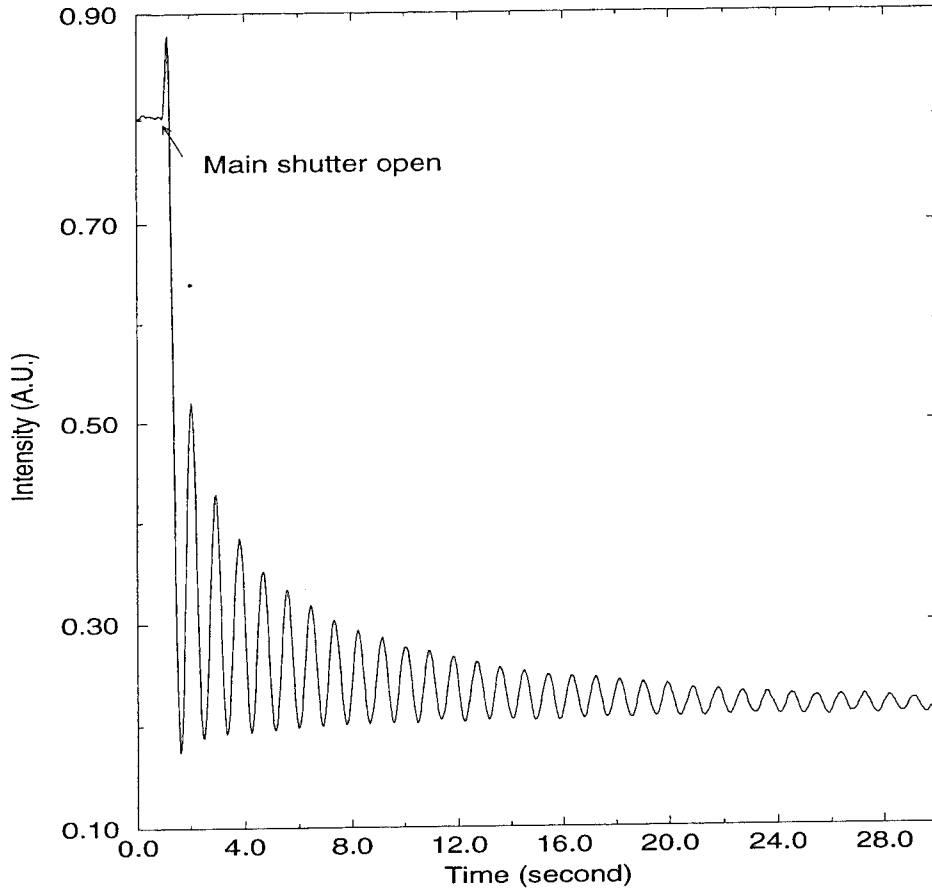
Fig. 4.3. RHEED oscillations of a GaAs surface on a (001) GaAs substrate at a substrate temperature of 580^\circ .
