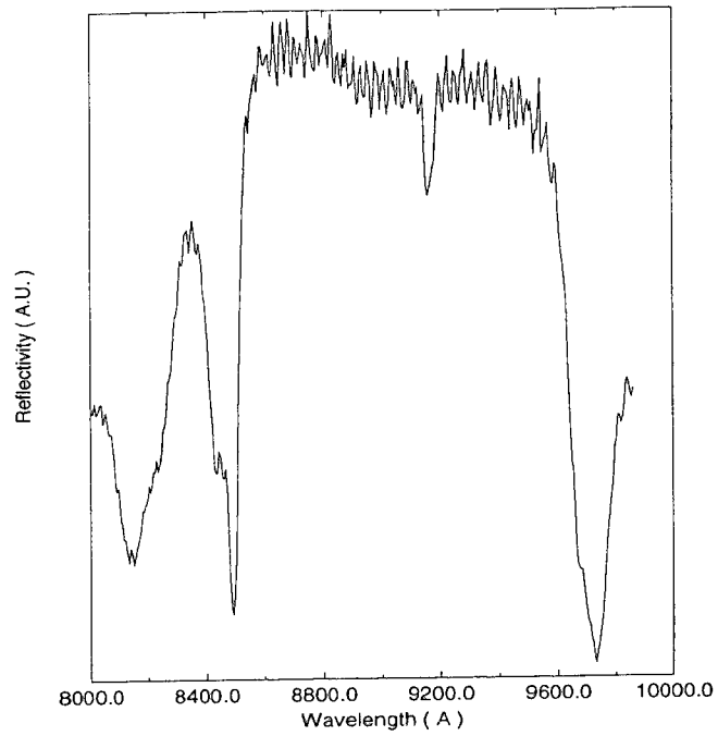
Fig. 7.1: The reflectivity spectrum of a VCSEL grown on a (110) GaAs substrate
