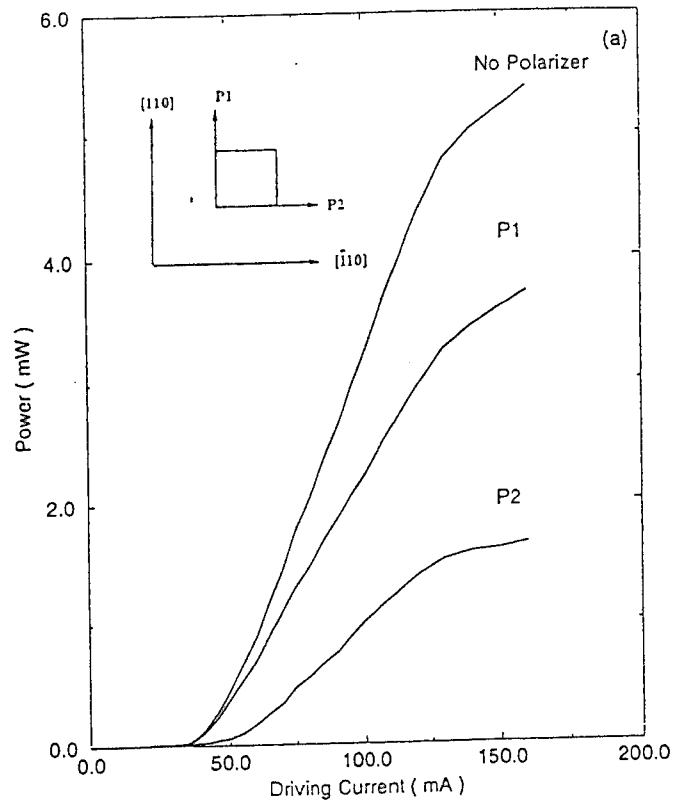
Fig. 6.2: Light output from a 50\ \mu\text{m} square VCSEL with and without a polarizer aligned along the directions as shown in the inset.
