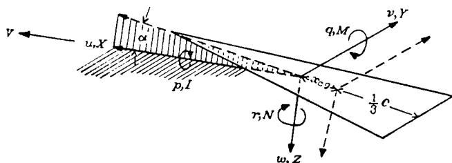
FIGURE 3. Velocities, forces, and moments relative to stability axes with origin at \frac{2}{3}c - x_0 . Principal axes of figure 2 dashed in for comparison.
