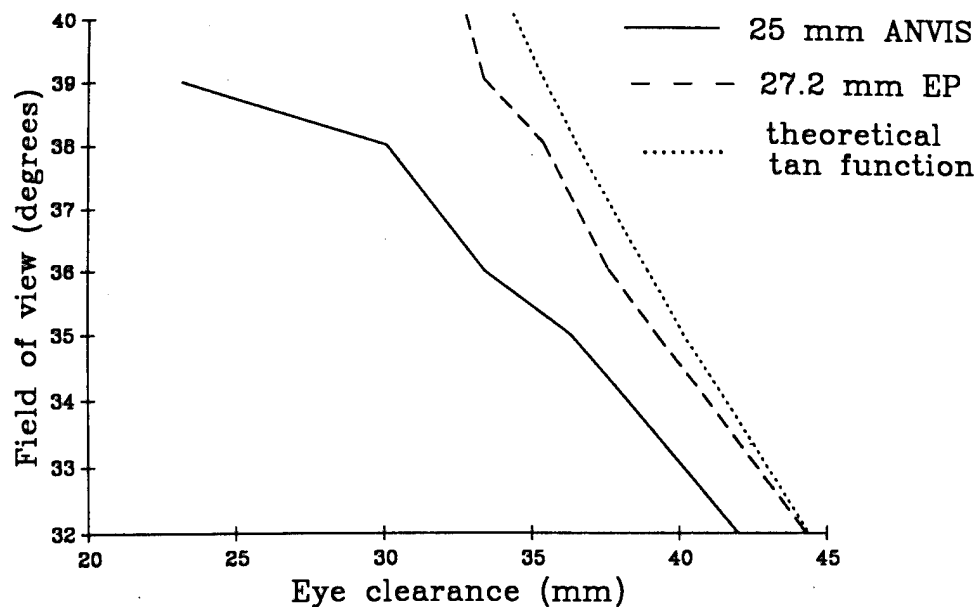
Figure 4. Plots of FOV versus Eye Clearance for 25-mm ANVIS eyepiece 27.2-mm mechanical iris theoretical calculated data.
