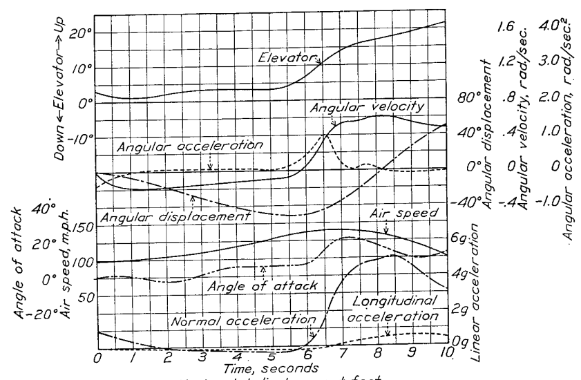
FIGURE 10.—First pull-out from dive
