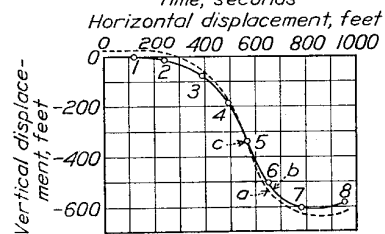
FIGURE 10.—First pull-out from dive
