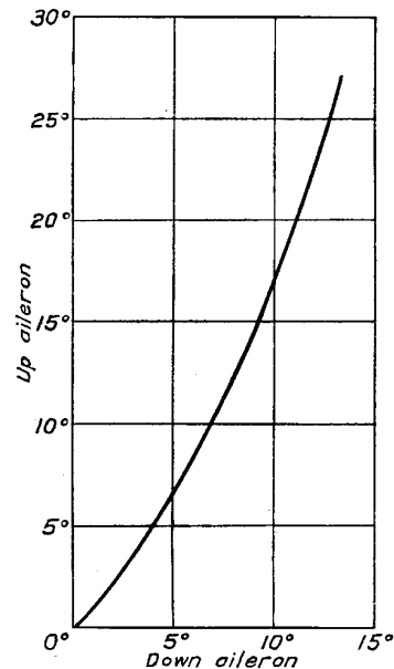
FIGURE 5.—Differential aileron action on F6C-3 airplane
