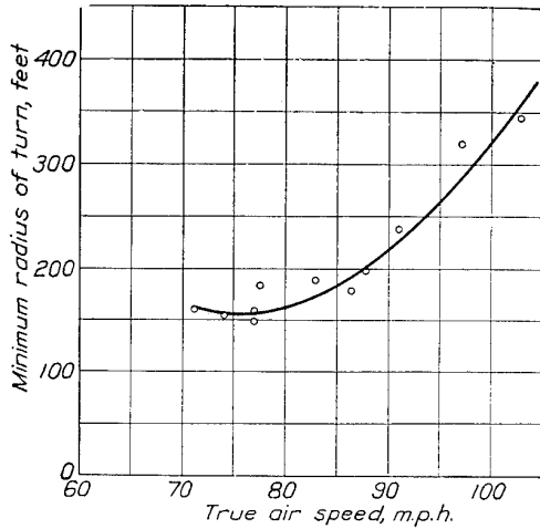
FIGURE 17.—Minimum radius of turn versus air speed
