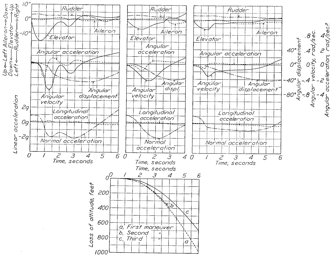
FIGURE 9.—Push-downs
