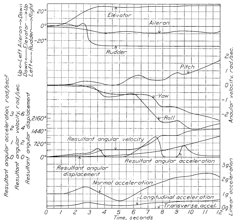
FIGURE 21.—First left spin
