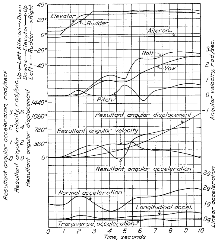
FIGURE 20.—Right spin
