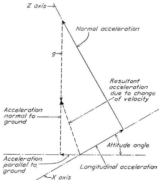
FIGURE 6.—Resolution of linear accelerations into horizontal and vertical components
