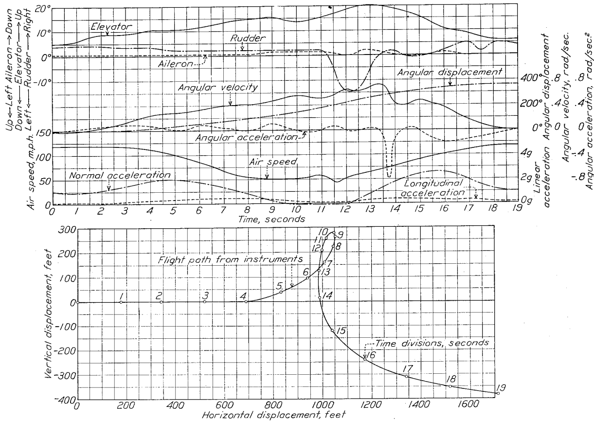
FIGURE 7.—Low-speed loop
