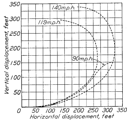
FIGURE 15.—Comparison of flight paths for abrupt pull-ups
