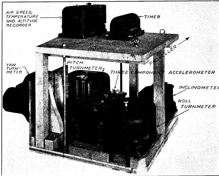
FIGURE 3.—Special instrument mounting
