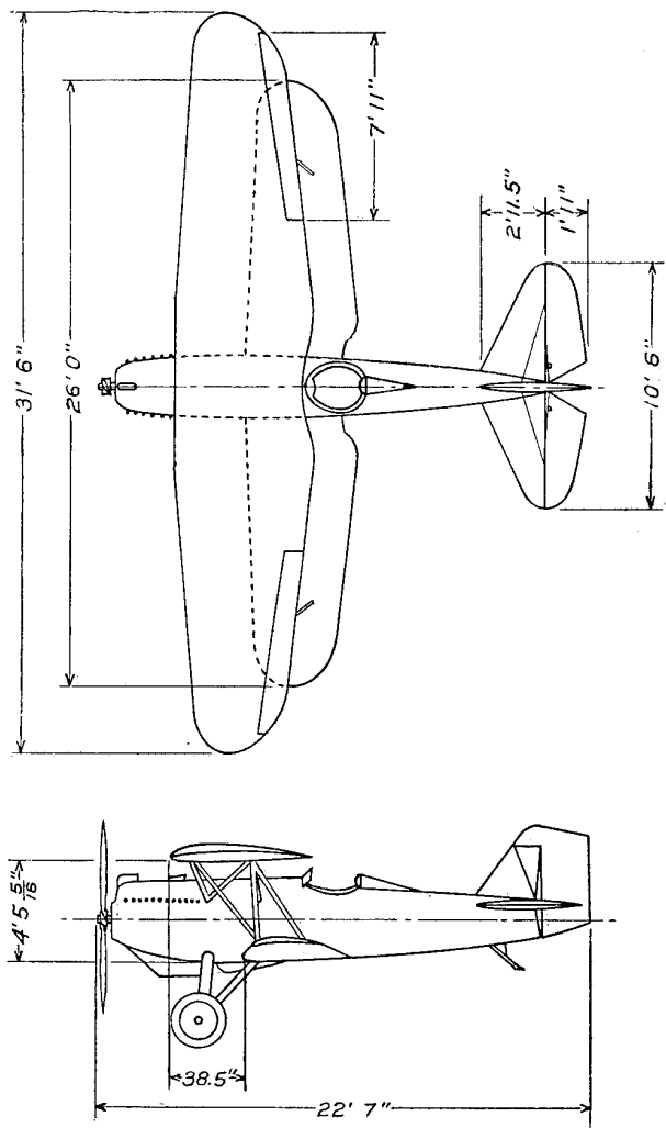
FIGURE 1.—Plan and elevation of the F6C-3 airplane
