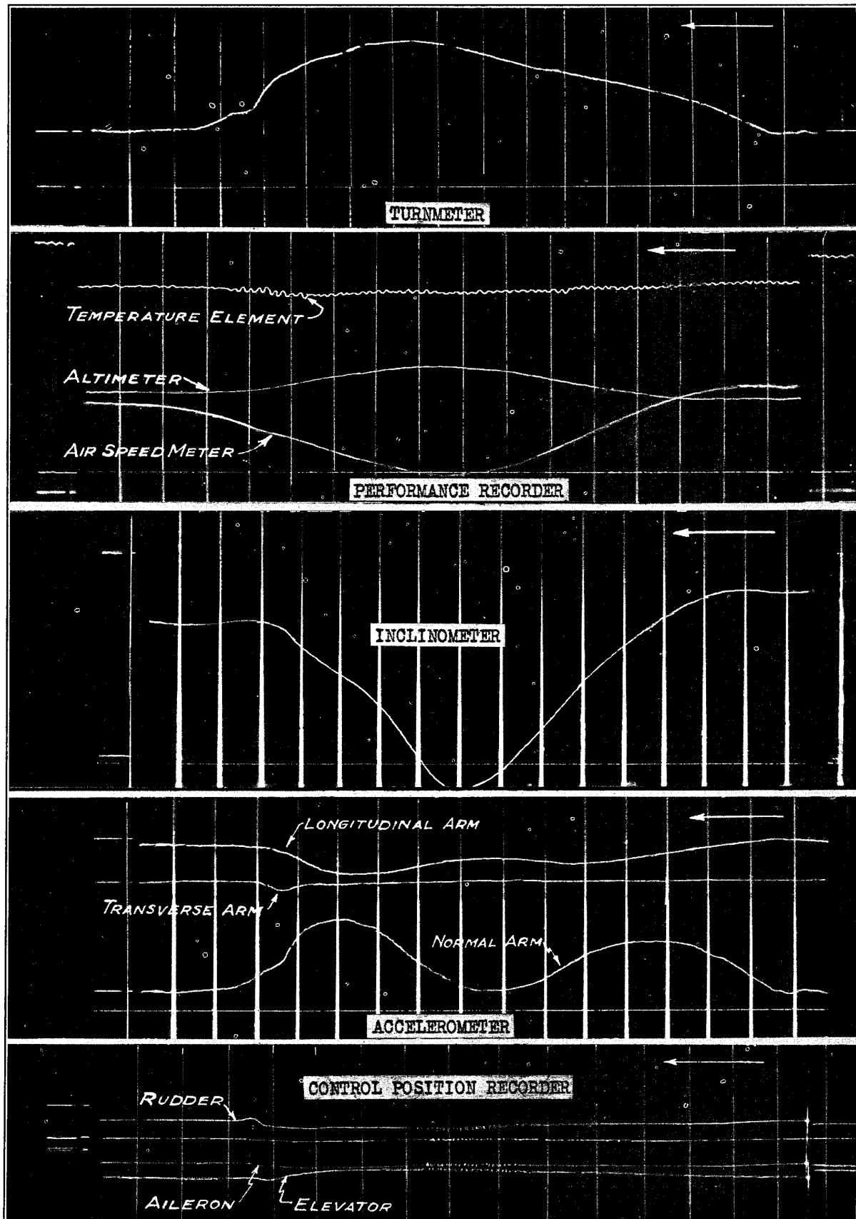
FIGURE 2.—Instrument records for a loop
