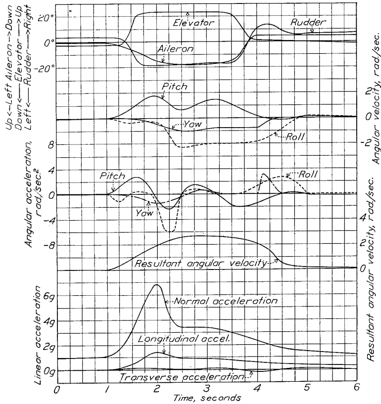
FIGURE 19.—Left barrel-roll started at 140 m. p. h.
