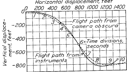
FIGURE 11.—Second pull-out from dive
