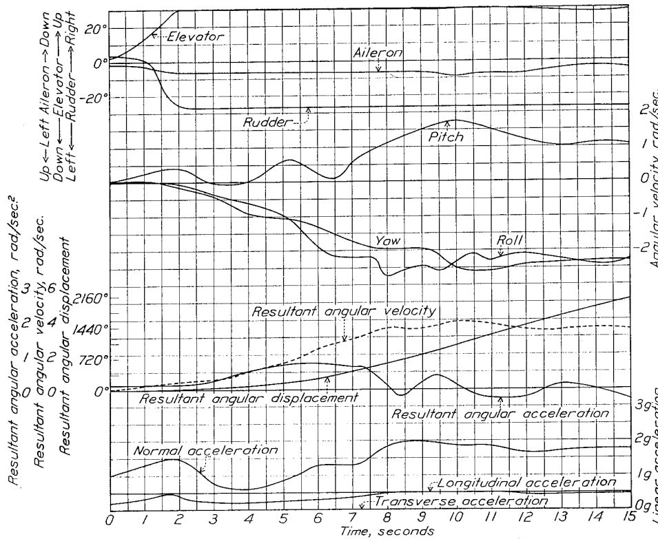
FIGURE 22.—Second left spin
