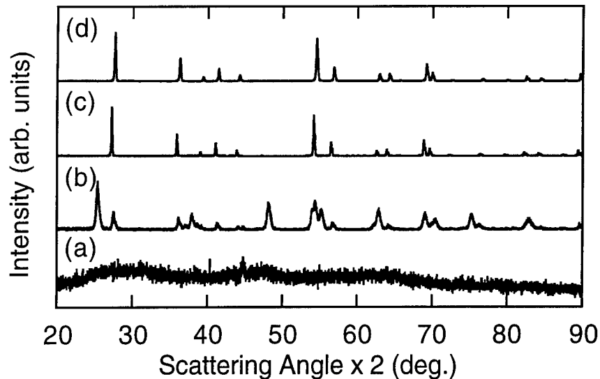
Figure 8. X-ray diffraction data for \text{TiO}_2 samples. (a) sol-gel powder; (b) calcined powder; (c) microwaved sample 2 (1 hr @ 1200 °C); and (d) microwaved sample 3 (2 hr @ 1200 °C).
