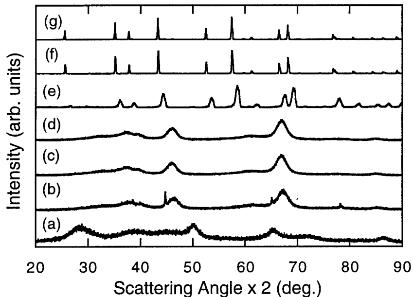
Figure 7. X-ray diffraction data for Al 2 O 3 samples. Curve a: sol-gel powder; b: calcined powder; c: CIP'ed green body; d: microwaved sample 1-1 (30 min. @1100°C); e: microwaved sample 1-4 (25 min. @1720°C), f: microwaved sample 2-3 (120 min. @1550°C), g: microwaved sample 2-8 (65 min. @1450°C and 71 min. @1650°C).
