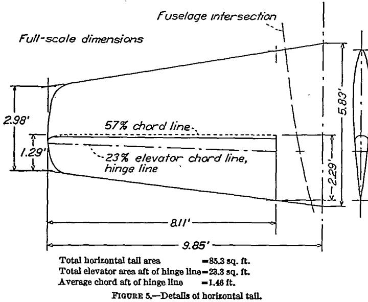
FIGURE 5.—Details of horizontal tail.
