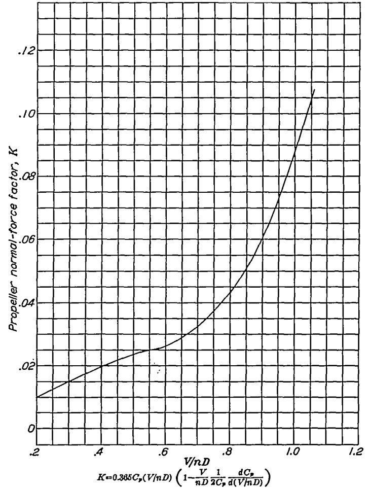
FIGURE 7.—Variation of K with V/nD for model propeller at a blade angle of 21.0° at 0.75 radius.
