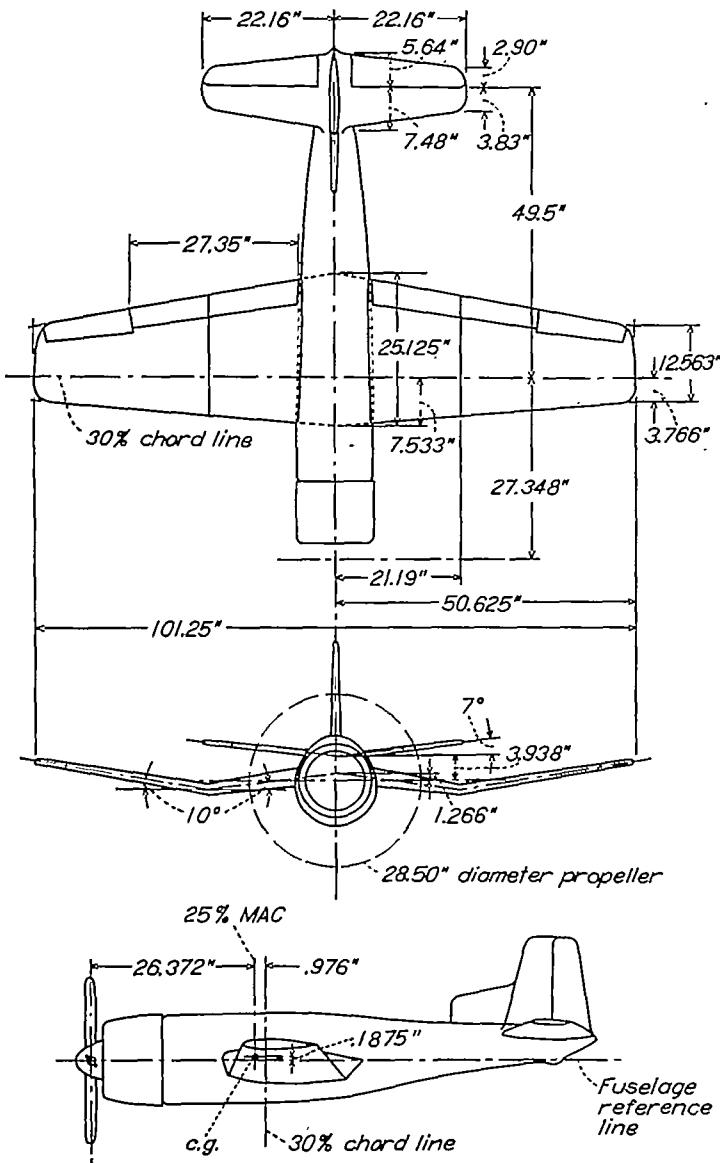
FIGURE 3.—Three views of a \frac{3}{16} -scale model of a single-engine airplane.
