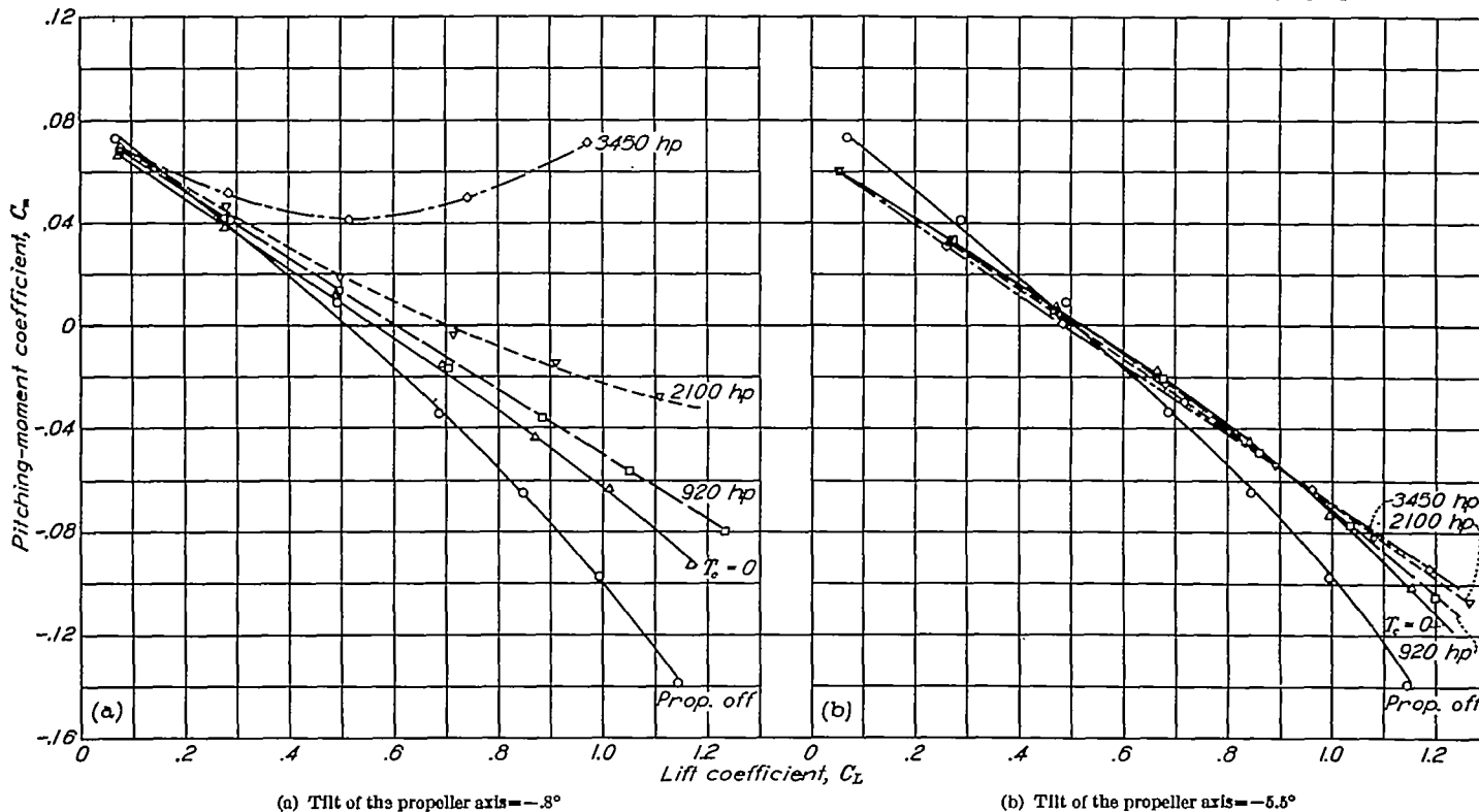
FIGURE 14.—Effect of propeller operation on longitudinal stability of a single-engine airplane with two tilts of the propeller axis. Raised tail position, \delta_a = 0^\circ , flaps up.
