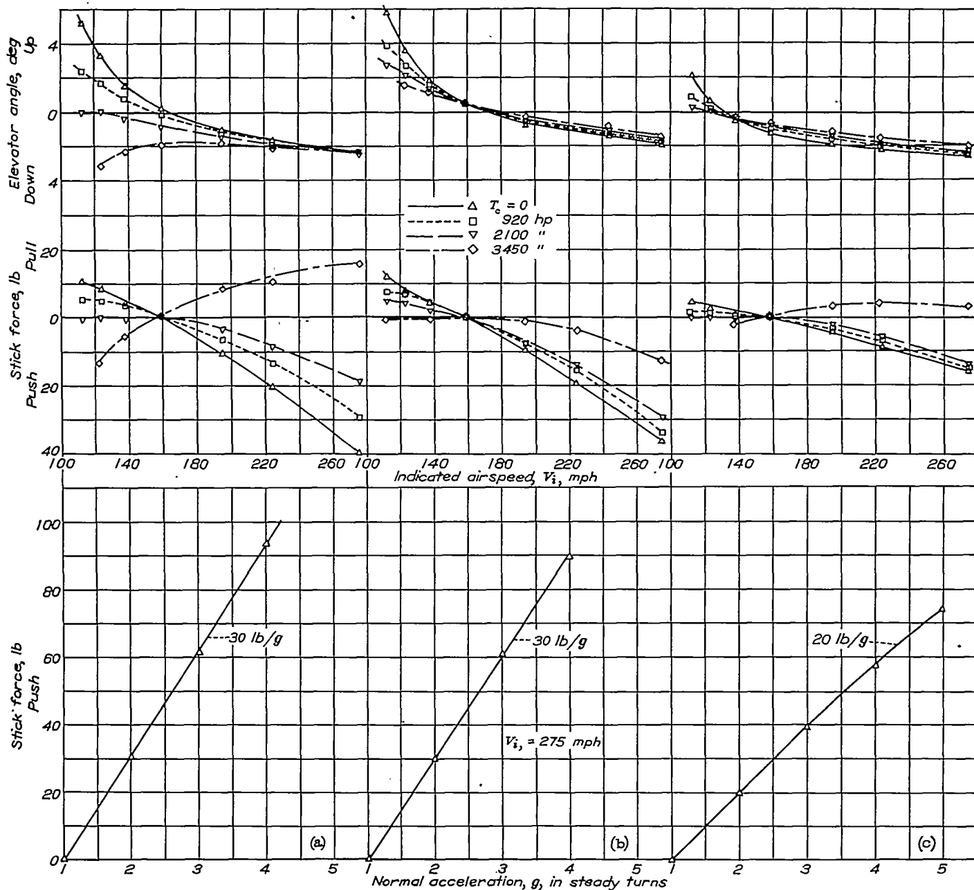
(a) Tilt of the propeller axis = -0.8^\circ c.g. at .25 M.A.O. (b) Tilt of the propeller axis = -5.5^\circ c.g. at .25 M.A.O. (c) Tilt of the propeller axis = -5.5^\circ c.g. at .30 M.A.O. FIGURE 26.—Effect of propeller operation on longitudinal handling characteristics of a single-engine airplane with two tilts of the propeller axis. Steady flight normal tail position, flaps up.
