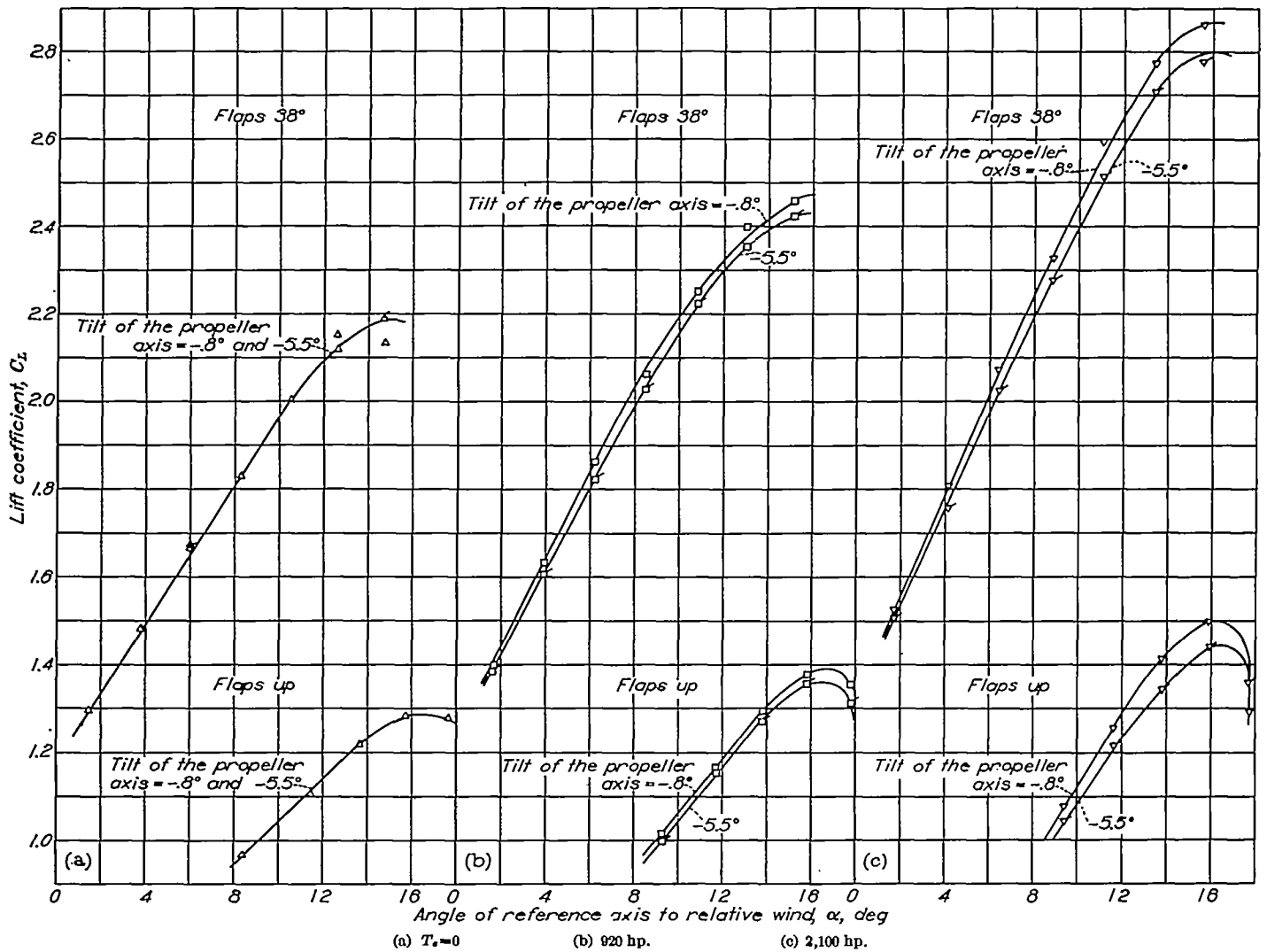
FIGURE 25.—Effect of tilt of propeller axis on the maximum lift coefficient of a single-engine airplane for three power conditions. Tall off, flaps up and flaps deflected 38^\circ .
