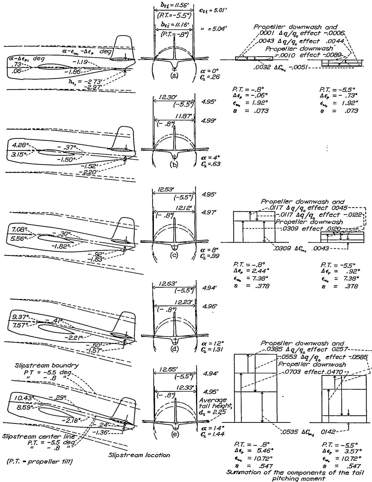
FIGURE 36.—Schematic pictures of slipstream location with two tilts of the propeller axis. Normal tail location, flaps 0^\circ , 2,100 horsepower.
