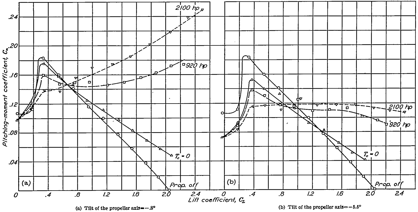
FIGURE 18.—Effect of propeller operation on longitudinal stability of a single-engine airplane with two tilts of the propeller axis. Normal tail position \delta_e = -10^\circ flaps deflected 38^\circ .
