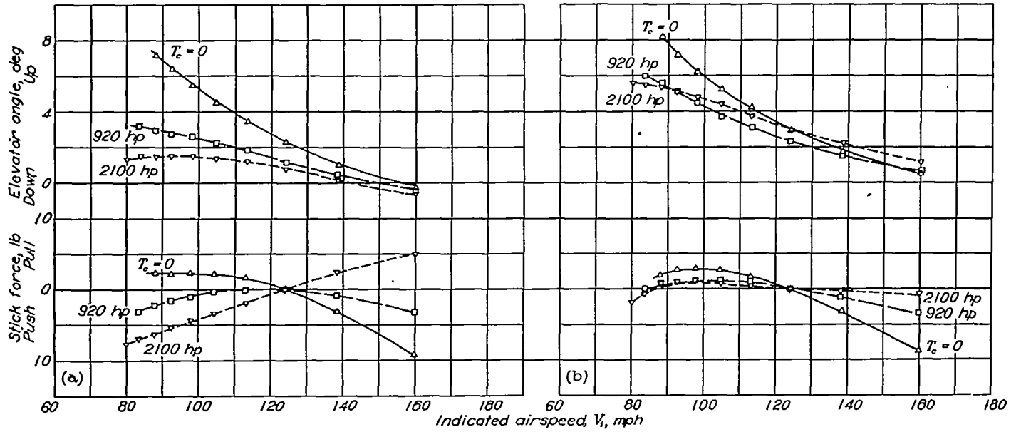
(a) Tilt of the propeller axis = -3° c.g. at 25 M.A.O. (b) Tilt of the propeller axis = -5.5° c.g. at 25 M.A.O. FIGURE 27.—Effect of propeller operation on longitudinal handling characteristics of a single-engine airplane with two tilts of the propeller axis. Steady flight, normal tail position, common flaps deflected 38°.
