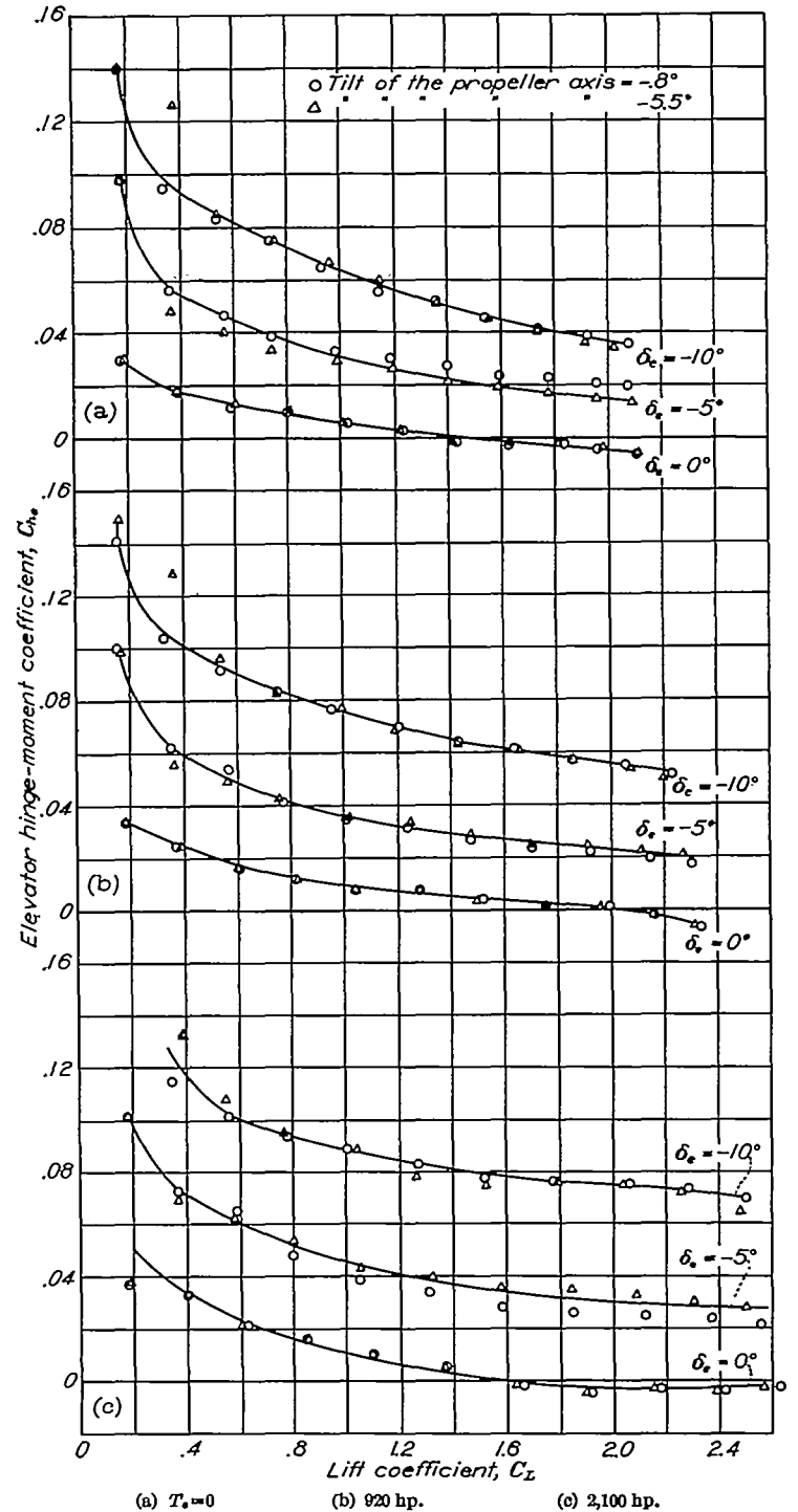
FIGURE 24.—Effect of propeller operation on elevator hinge moment of a single-engine airplane with two tilts of the propeller axis. Normal tail position, flaps deflected 33^\circ .
