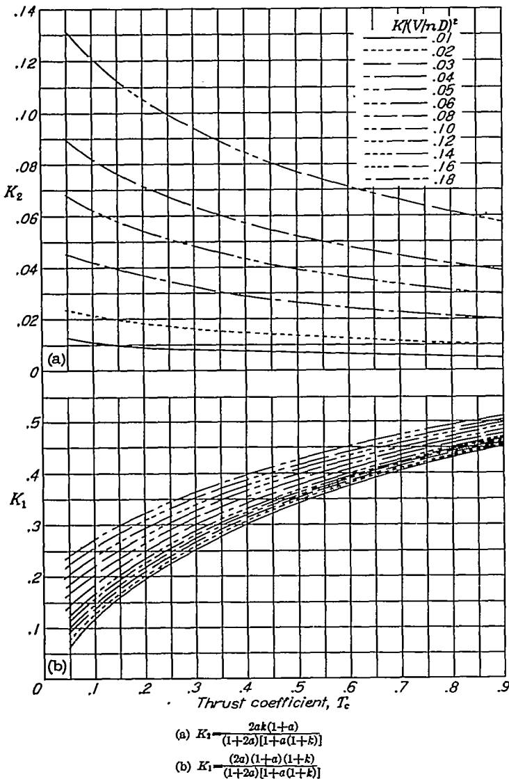
FIGURE 32.—Variation of K_1 and K_2 with T_c and K/(V/nD)^2 .
