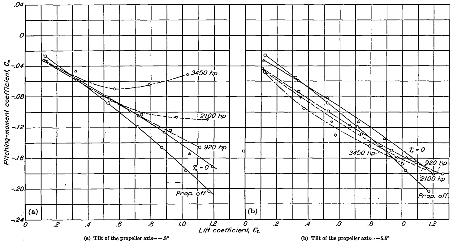
FIGURE 11.—Effect of propeller operation on longitudinal stability of a single-engine airplane with two tilts of the propeller axis. Normal tail position \delta_e = 5^\circ flaps up.
