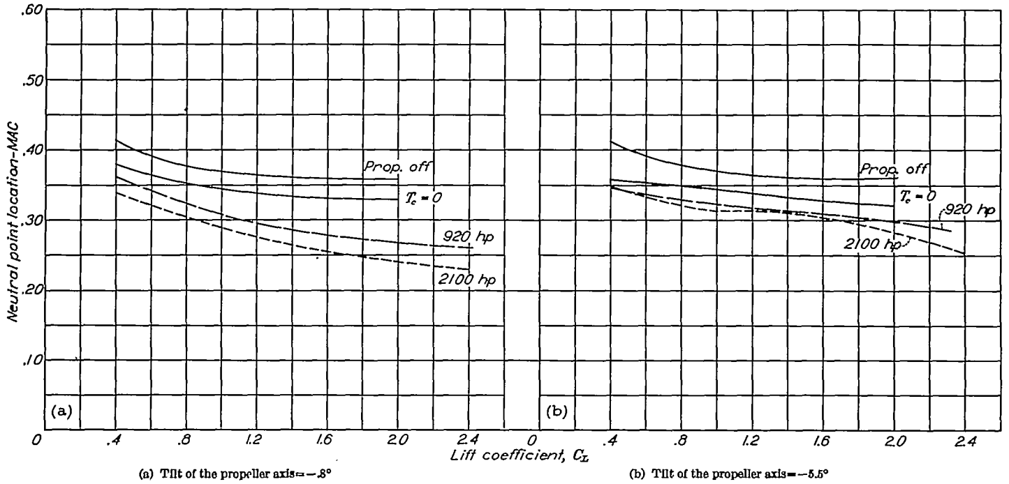
FIGURE 21.—Effect of propeller operation on neutral point location of a single-engine airplane with two tilts of the propeller axis. Normal tail position, elevator deflection to trim, flaps deflected 38^\circ .
