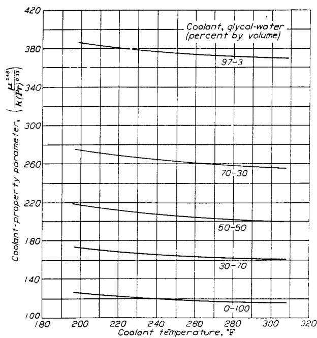
FIGURE 16.—Variation of coolant-property parameter \left( \frac{\mu^{0.48}}{k(P_T)^{0.33}} \right) with coolant temperature for cylinder-head-temperature correlation.
