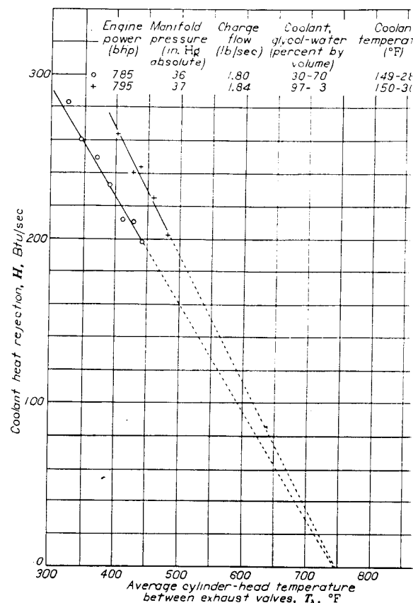
FIGURE 19.—Determination of T_g from variation of coolant heat rejection with cylinder-head temperature between exhaust valves for coolant-heat-rejection correlation. Coolant flow, 200 gallons per minute; engine speed, 2600 rpm; fuel-air ratio, 0.095; dry manifold temperature, 254° F; exhaust pressure, 29-30 inches mercury absolute; standard ignition timing.
