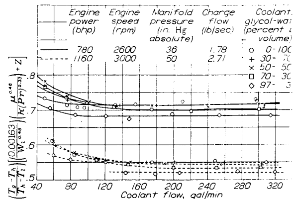
FIGURE 17.—Variation of \left( \frac{T_c - T_h}{T_h - T_i} \right) \left[ \left( \frac{0.00163}{W_c^{0.48}} \right) \left( \frac{\mu^{0.48}}{k(P_T)^{0.33}} \right) + Z \right] with coolant flow as indication of boiling. Average coolant temperature, 245^\circ F; engine D.
