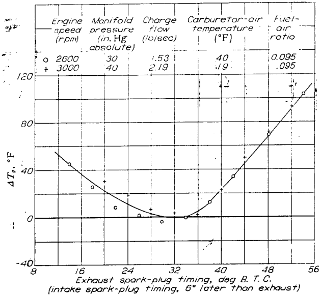
FIGURE 7.—Variation of change in effective cylinder-head temperature with ignition timing for cylinder-head-temperature correlation. Engine D.
