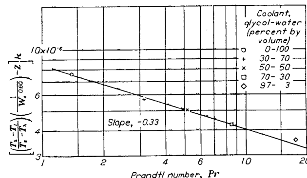
FIGURE 13.—Determination of exponent s on Prandtl number Pr for cylinder-head-temperature correlation from variation of \left[ \left( \frac{T_h - T_i}{T_s - T_h} \right) \left( \frac{1}{W_c^{0.60}} \right) - Z \right] k with Pr as obtained from cross plot of figure 12 at value for W_i/\mu of 55,000. Average coolant temperature, 245° F; engine D.
