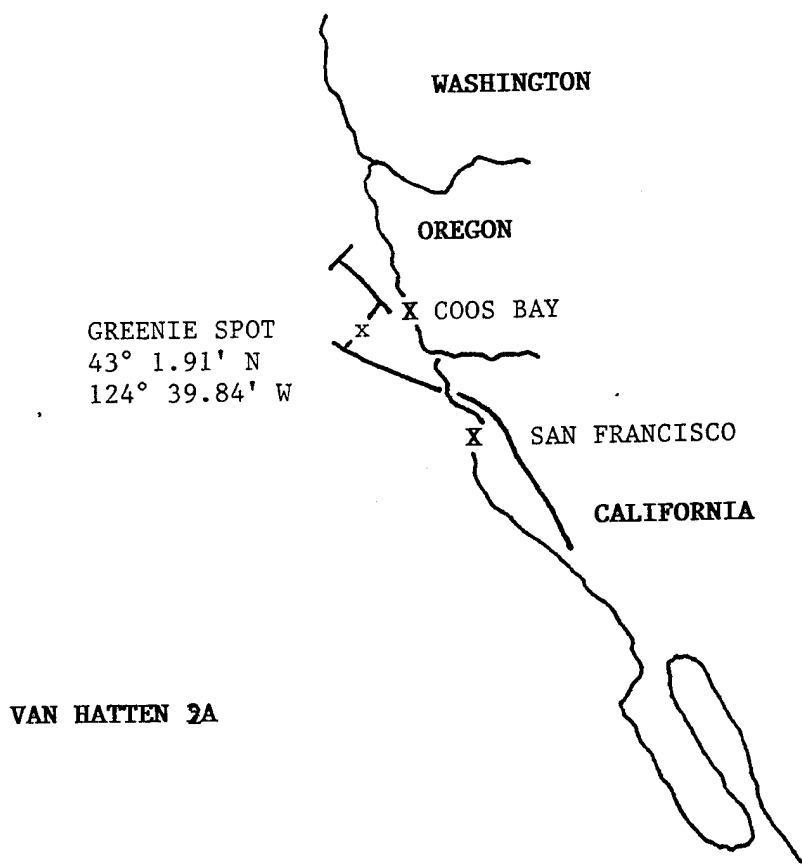
FIG. 2: The Greenie Spot on the Juan de Fuca Ridge
