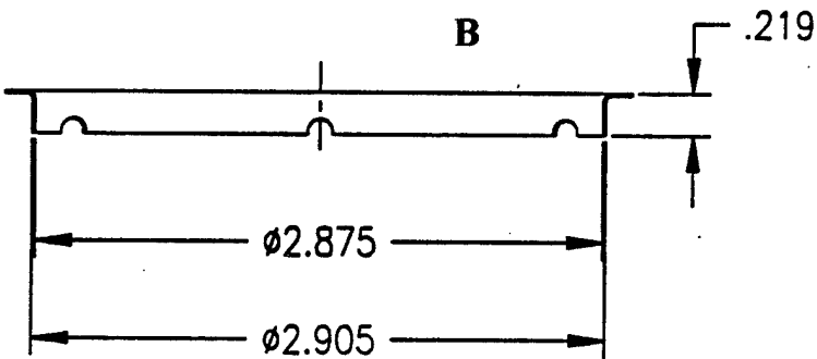
FLANGE CONTROL GRID INSULATOR 372441 KOVAR
