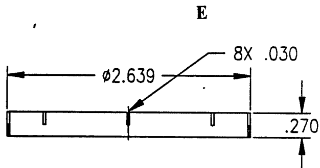
SHADOW GRID SUPPORT CYLINDER 372426 KOVAR
