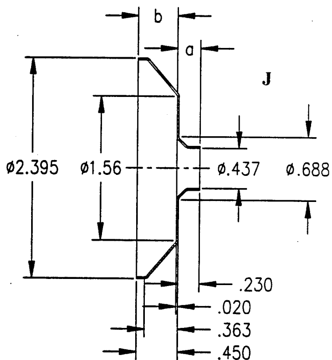
SEAL KOVAR 372454
