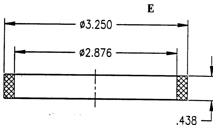
INSULATOR 372437 AL-300
