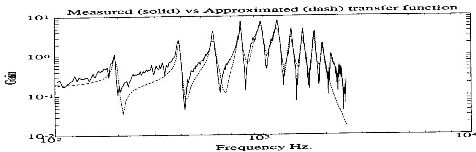
Figure 16: Measured transfer function and analytical approximation
