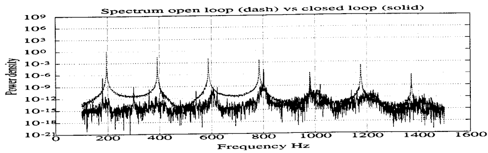
Figure 21: Comparison of open and closed Loop power spectrums
