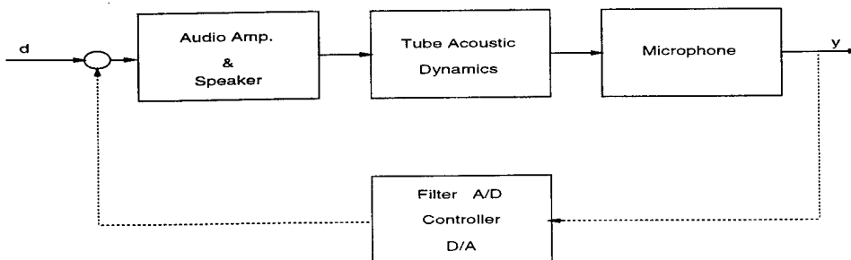
Figure 15: System I.D. and controller setup
