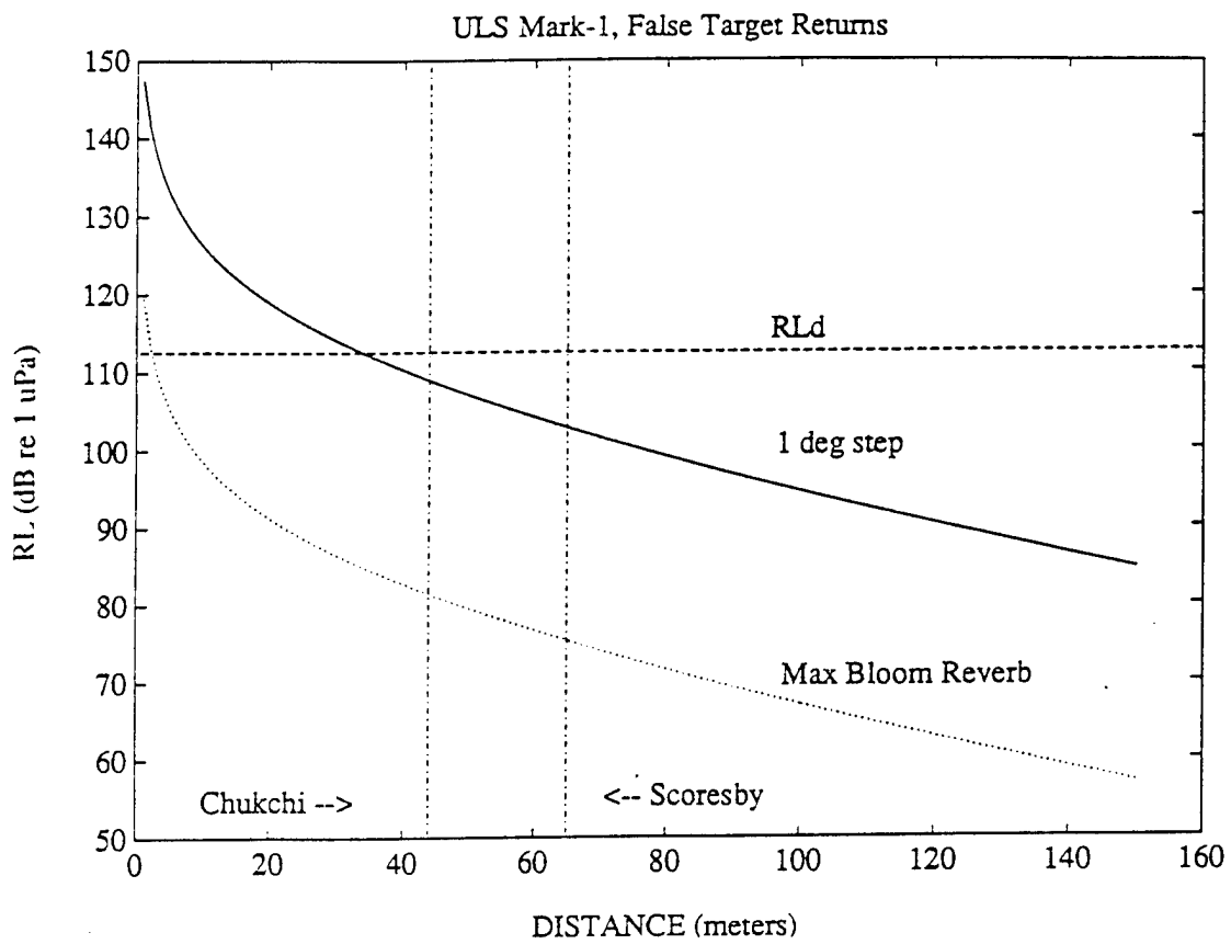
Figure 7: Received level as a function of distance for ULS Mark-1. Targets are: 1° C temperature step in seawater (solid curve) and volume reverberation from maximal plankton bloom (dotted curve).
