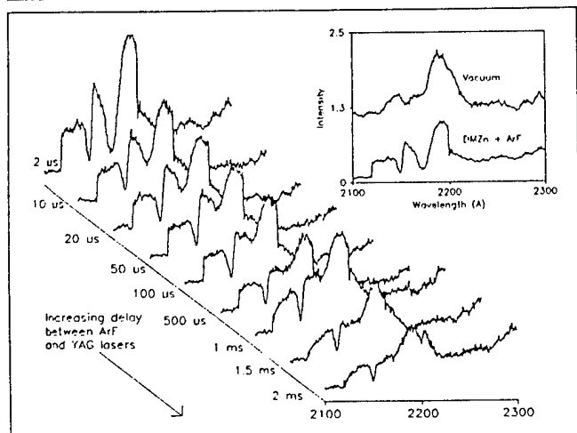
Fig. 6. Variation of absorption profiles at different delay times. A plasma spectra through vacuum and the spectra taken at 2 \mu s delay is shown for reference in the inset. The CH_3 absorbance decays after several hundred microseconds, while the Zn profile remains constant (the relative depth of the Zn absorption is the same at 2 \mu s as at 2 ms). The overall signal intensity decreases as undissociated DMZn flows back into the dissociation region. The resolution of the spectrometer for these experiments was 6Å.
