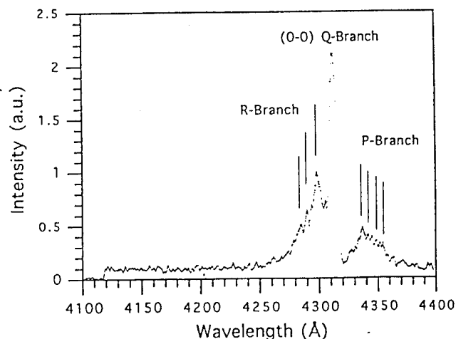
Fig. 12. Emission from the \text{A} \rightarrow \text{X} transition of the CH radical. The peak at 4315 Å is due to the 0-0 Q-branch transition, and the P-branch and R-branch vibrational transitions are also evident. Also of note is the lack of emission at 4128 or 4176 Å which are identified with the \text{A} \rightarrow \text{X} transitions of MMZn. The spectral resolution of the spectrometer for these experiments was 10 Å.
