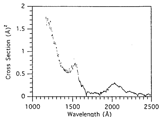
FIG. 7. Absorption cross section for DMZn from 1150 to 2500 Å. The peaks have been identified by Ibuki and co-workers (Ref. 25) as the Rydberg transitions 4p \leftarrow 2a_1'' ( \sim 2020 \text{ Å} ), 4p \leftarrow 3a_1' ( \sim 1520 \text{ Å} ), and 3p \leftarrow 2e and/or 3p \leftarrow 2e'' ( \sim 1180 \text{ Å} ).
