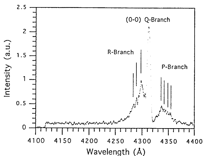
FIG. 11. Emission from the A \rightarrow X transition of the \text{CH} radical. The peak at 4315 Å is due to the 0-0 Q -branch transition, and the P -branch and R -branch vibrational transitions are also evident. Also of note is the lack of emission at 4128 or 4176 Å which are identified with the A \rightarrow X transitions of \text{MMZn} . The resolution of the spectrometer for these experiments was 10 Å.
