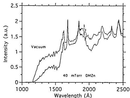
FIG. 2. Typical spectral output of the plasma emission from 1000 to 2500 Å. The upper trace is the detected plasma spectrum with vacuum in the absorption cell, and the lower trace is the detected plasma spectrum with 40 mTorr of DMZn in the absorption cell. Two broadband absorptions can be seen, one around 2000 Å (near the wavelength of the ArF laser), and another in the deep VUV from 1200 to 1600 Å. The peaks in both spectra are line emission from ionized argon, mainly Ar II and Ar III, while the broad continuum is due mainly to free-free transitions, or bremsstrahlung.
