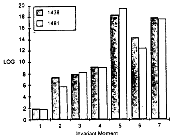
Fig. 6 Histogram of the absolute value of the log of the invariant moments corresponding to the reference floe.
