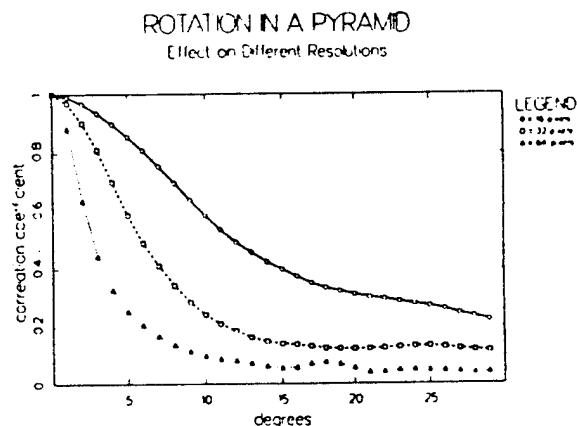
Fig. 4. Two-dimensional cross-correlation function with respect to angle of rotation for window sizes of 16, 32, and 64 pixels to a side all depicting the same area of 16x16 kilometers. Twenty SAR sea ice scenes, extracted from SEASAT orbits 1396 and 1439, were used in the averaging process.
