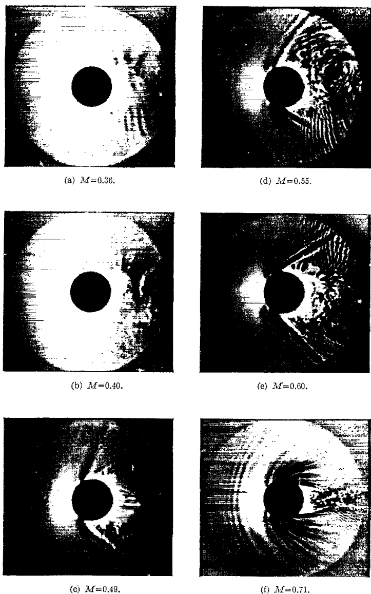
FIGURE 10.—Shadowgraphs of flow about the 2¼-inch-diameter circular cylinder. Static water depth, 1.00 inch.
