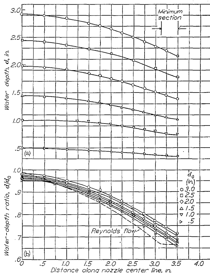
(a) Variation of water depth along center line showing shape of free surface. (b) Variation of water-depth ratio d/d_0 along center line for different values of the total head d_0 .
