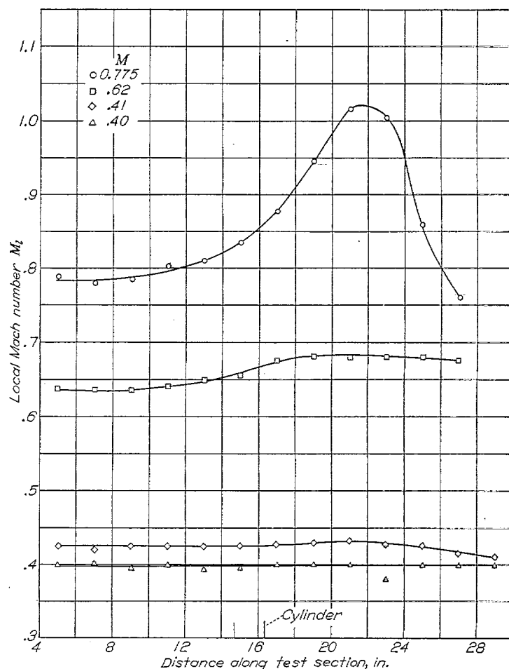
FIGURE 22.—Variation of local Mach number along channel wall with a 1\frac{1}{4} -inch-diameter circular cylinder.
