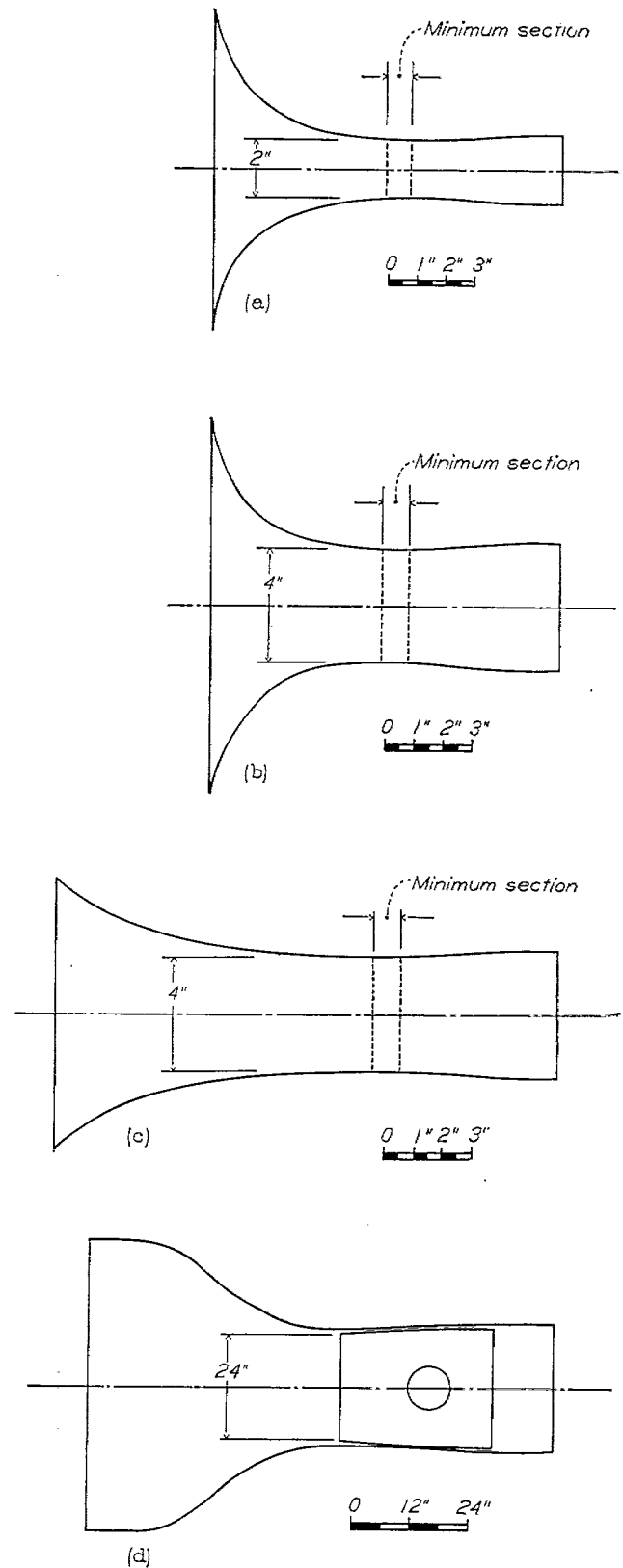
(a) Two-inch Laval nozzle (reference 4). (b) Four-inch Laval nozzle (reference 4). (c) Four-inch Laval nozzle with modified approach. (d) Twenty-four-inch nozzle, final wall shape.
