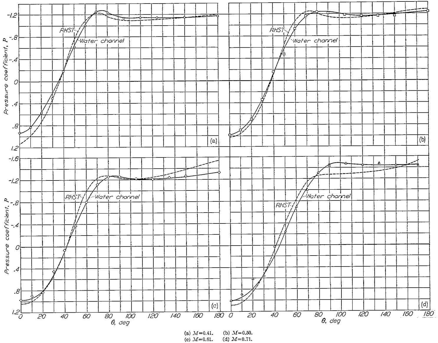
FIGURE 20.—Comparison of pressure distributions about a 2\frac{3}{4} -inch circular cylinder in the water channel with the pressure distributions about a \frac{3}{4} -inch circular cylinder in the Langley rectangular high-speed tunnel (RHST).
