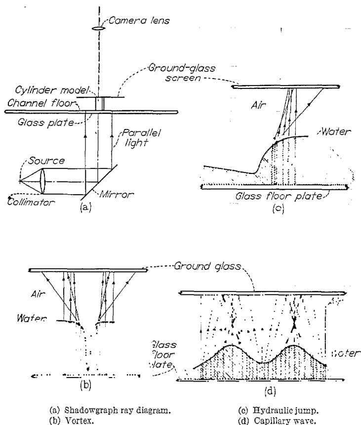
FIGURE 7.—Analysis of method for photographing free surface.
