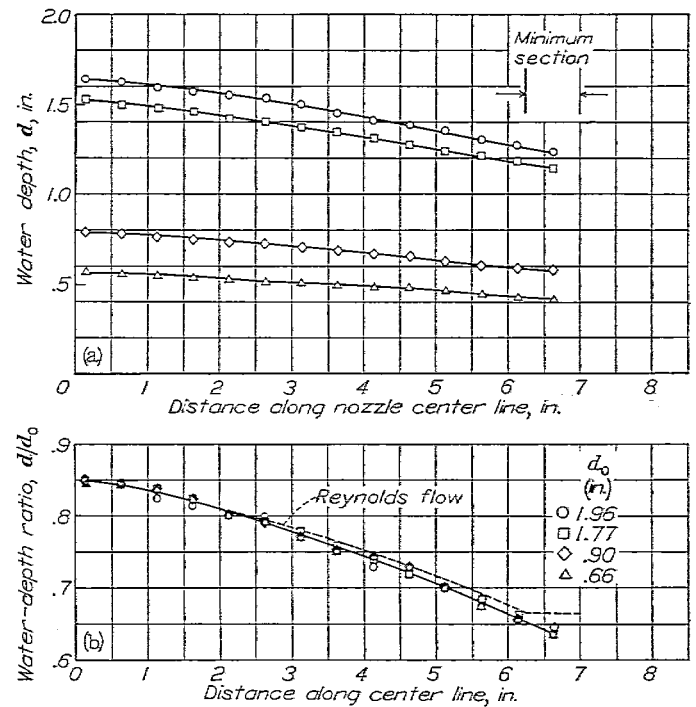
(a) Variation of water depth along center line showing shape of free surface. (b) Variation of water-depth ratio d/d_0 along center line for different values of the total head d_0 .
