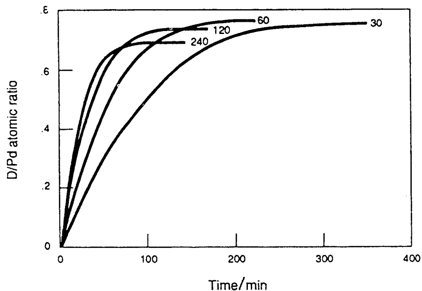
Figure 2. Model calculation of loading curves as a function of current density: electrode radius 0.05 cm; current densities are indicated in mA cm -2 ; diffusion coefficient 1.6 \times 10^{-6} cm 2 s -1 , other parameters are listed in Table 1.
