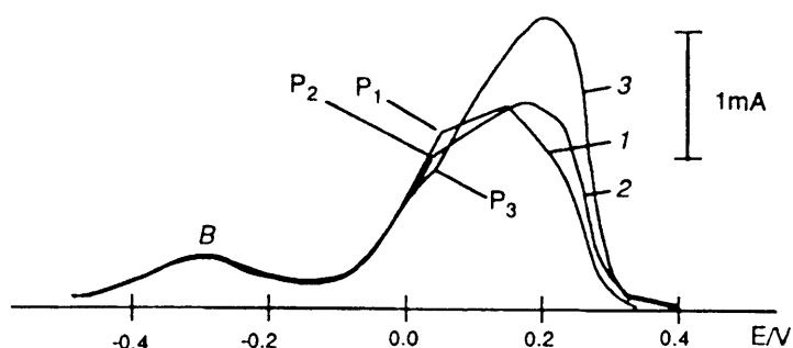
Figure 6. Effect of addition of light water, electrode surface black palladium electrolyte, 0.3 M \text{Li}_2\text{SO}_4 , pH 12, scan rate 10 \text{ mV s}^{-1} : curve 1, 10 ml \text{D}_2\text{O} , 2 ml \text{H}_2\text{O} ; curve 2, 10 ml \text{D}_2\text{O} , 5 ml \text{H}_2\text{O} ; curve 3, 10 ml \text{D}_2\text{O} , 10 ml \text{H}_2\text{O} .
