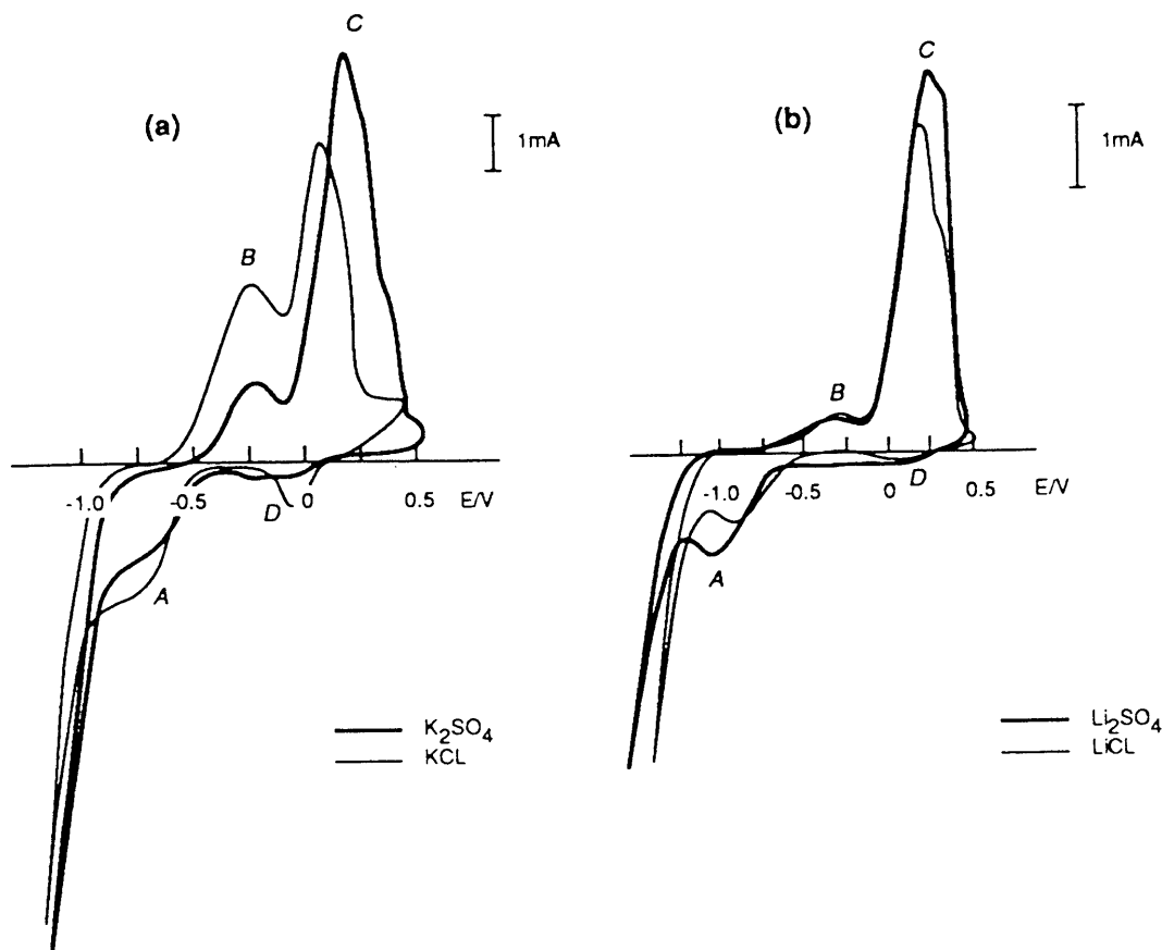
Figure 9. Effect of the supporting electrolyte, scan rate 10 \text{ mV s}^{-1} , electrode surface black palladium, pH 12, solvent D 2 O: (a) 0.3 M potassium salts ( \text{Cl}^- , \text{SO}_4^{2-} ); (b) 0.3 M lithium salts (as above), \text{SO}_4^{2-} thick line, \text{Cl}^- thin line.
