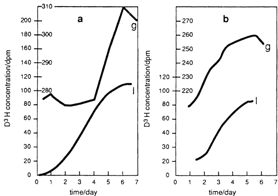
Figure 4. Distribution of .^3H generated by electrochemical compression of ^2H . Electrolyte: a – 0.3 N LiCl in ^2H_2O ; b – 0.3 N Li_2SO_4 in ^2H_2O ; 1 – electrolyte phase, g – gas phase.
