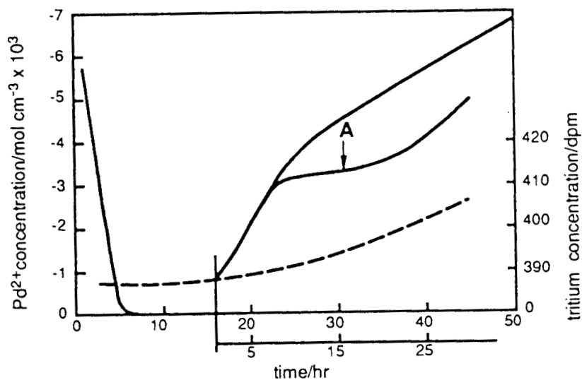
Figure 3. Early period in the co-deposition process. Left – \text{Pd}^{2+} concentration as a function of time; right – ^3\text{H} as a function of time; point A indicates addition of \text{SC}(\text{NH}_2)_2 ; dashed line – calculated isotopic enrichment.
