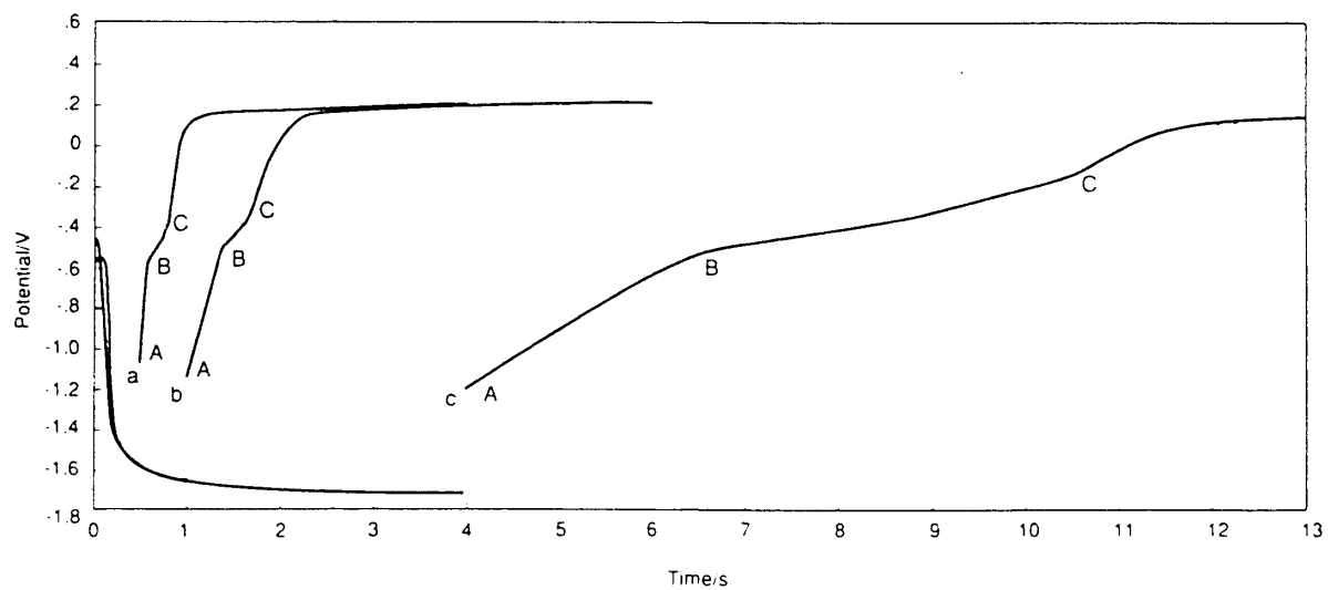
Figure 3. Approach to electrode rest potential \Phi(t)_{j=0} upon termination of the codeposition. Cathodic current density j = -10^{-1} \text{ A cm}^{-2} terminated at 0.5 s, 1 s and 4 s (curves a, b, and c respectively).
