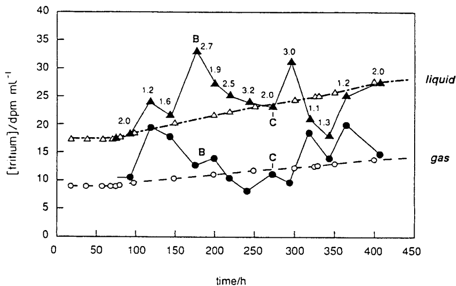
Figure 7. Tritium distribution as a function of time (electrode, prepared by codeposition from \text{PdCl}_2 solution; mode of operation, open cell with cell current profile indicated): ——— calculated distribution using s = 2.0 ; ——— experimentally measured tritium content (data from ref. 12). Experimental s values are indicated.
