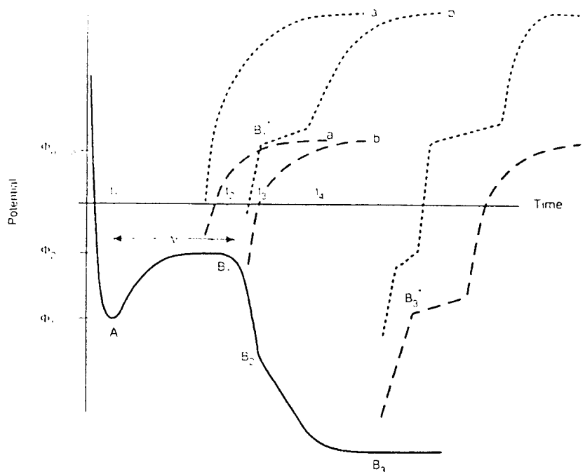
Figure 1. Idealized representation of the \Phi(t) response to a galvanostatic pulse (solid curve) and the \Delta\Phi(t) relaxation on current interruption at points indicated (broken curves): point A, onset of crystallization (nucleation); period \Delta t represents an asymptotic approach to a complete coverage by \text{PdD}_x deposit; points B_1, B_2, \dots, B_1^* indicate a change in the reaction path. Curves a, b, c for \Phi(t)|_{j=0} ; curves a', b', c' for \Phi(t)|_{j>0} .
