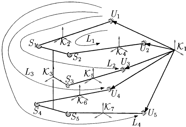
Figure 34: Schematic model of the five-point wheel suspension
