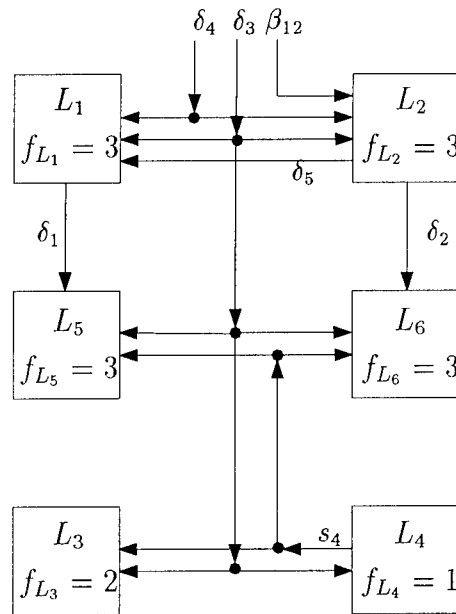
Figure 49: Kinematical network of the mixer unit
