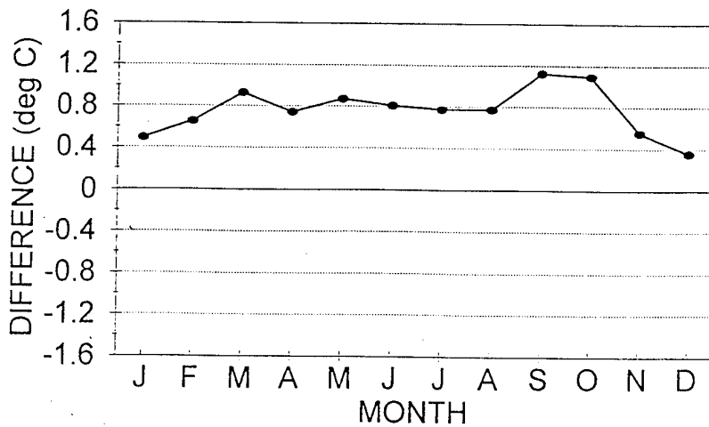
Figure 35. Zonal differences for 50 degrees South.
