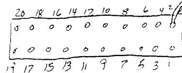
CONNECTOR VIEW (WIRE SIDE)
