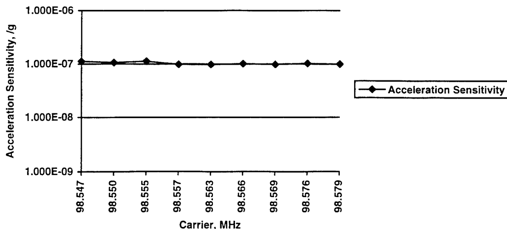
Acceleration Sensitivity Vs. Frequency Vibration Frequency = 5000 Hz
