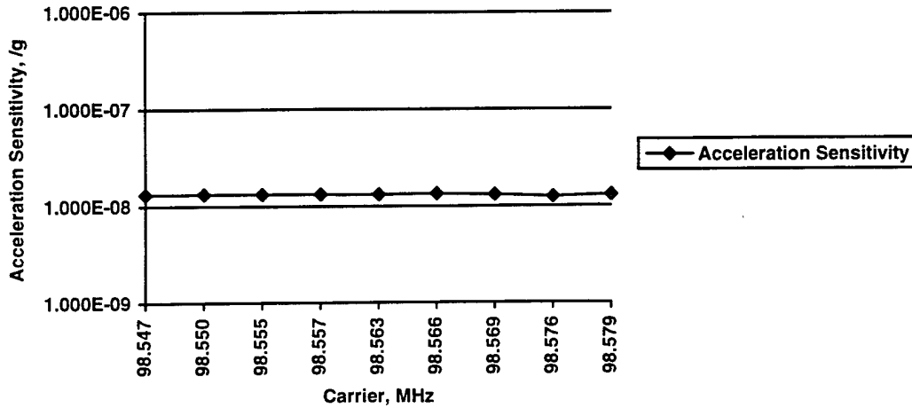
Acceleration Sensitivity Vs. Frequency Vibration Frequency = 500 Hz
