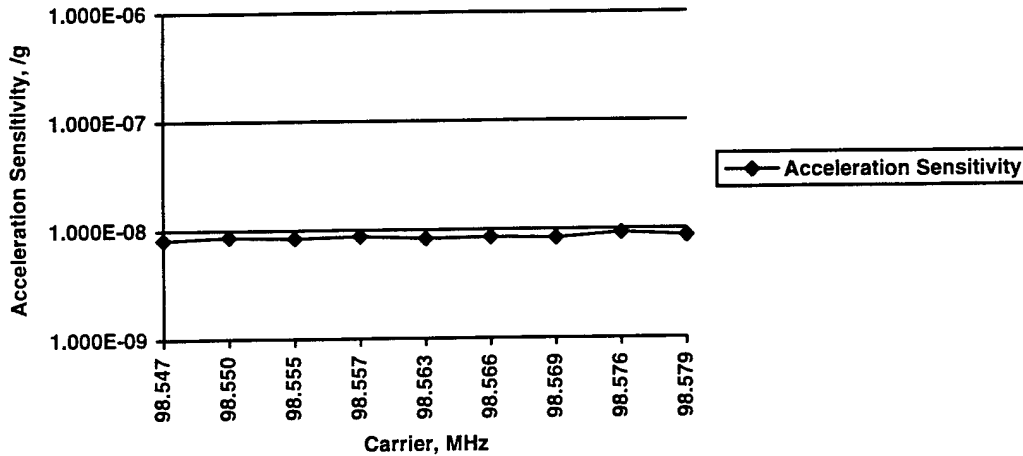
Acceleration Sensitivity Vs. Frequency Vibration Frequency = 90 Hz
