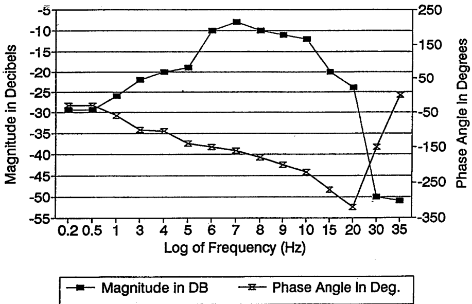
Figure 10. Coupled TF of Joint 2 - Input on Joint 1
