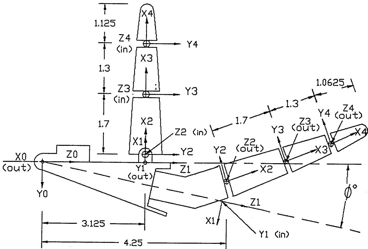
Figure 3. The Utah/MIT Dexterous Hands - Plan View
