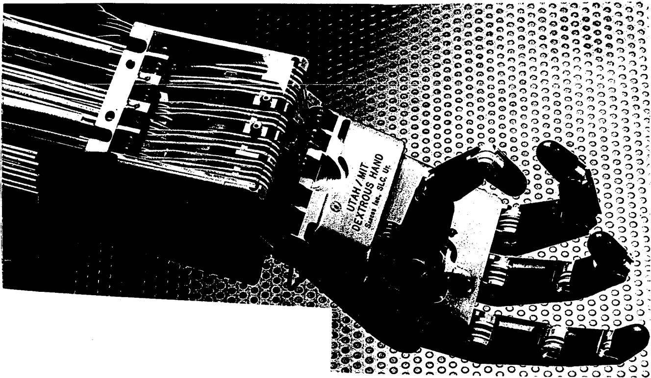
Figure 5. The Utah/MIT Dexterous Hand
