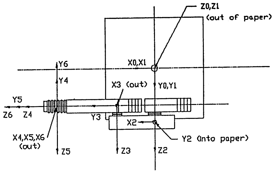
Figure 2. The Merlin 6500 Manipulator Frame Assignments - Plan View
