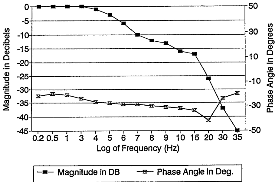
Figure 9. Transfer Function (TF) of Joint 1 - Input on Joint 1
