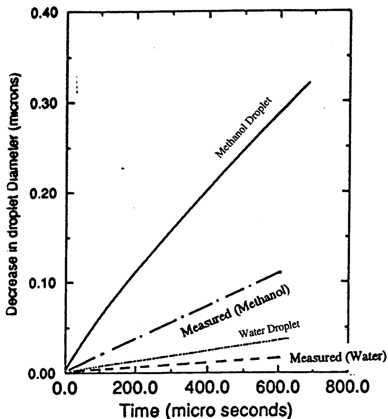
Figure 23 Comparison Between Experimental and Numerical Results for Quiescent Air Case
