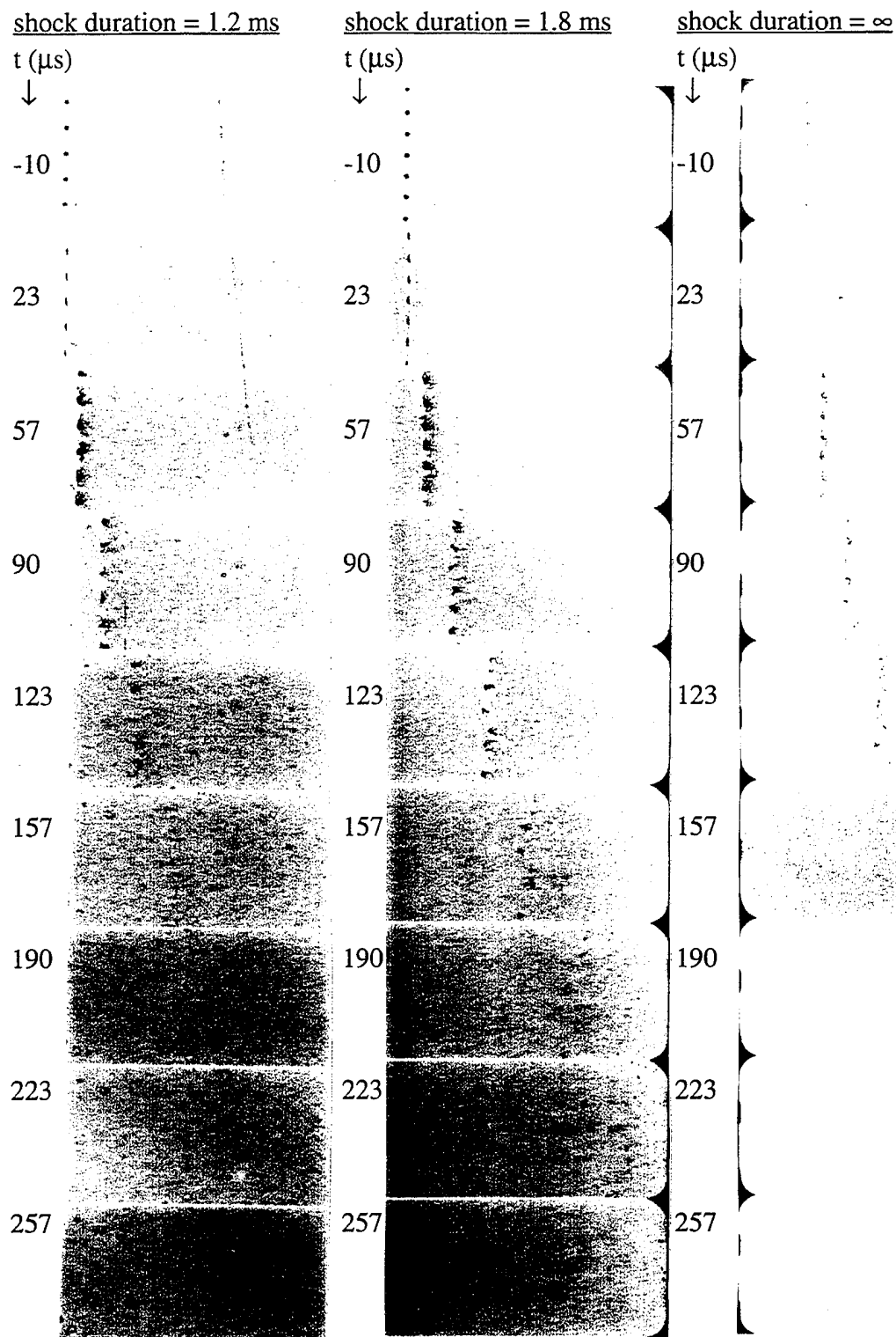
Figure 21b Shadowgraph Images of Methanol Drop Stream Interacting with a Shock Wave D = 145 \mu\text{m} , Shock Strength = 1.5, Shock Direction: Left-to-Right
