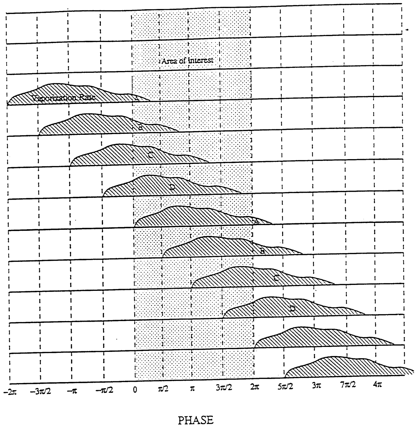
Figure 3: Vaporization rate (schematic) distribution for various droplets present in the combustor .
