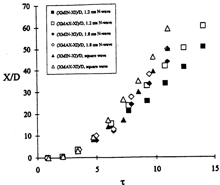
Figure 22b Methanol Droplet Displacement as a Function of Time D = 145 \mu\text{m} , Shock Strength = 1.5
