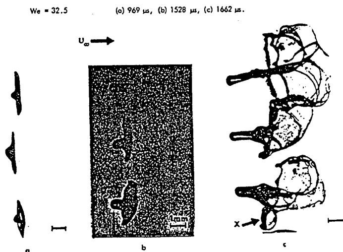
Figure G-2 Typical Parasol Mode Droplet Breakup
