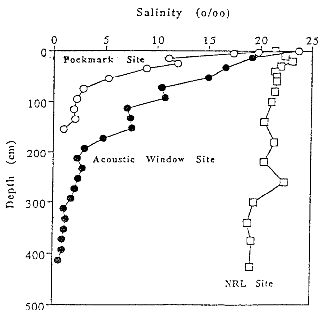
Figure 6. Overlay of salinity profiles from the three sites.
