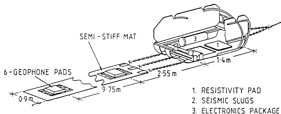
Fig.2 The UCNW sea floor sled- 'magic carpet'
