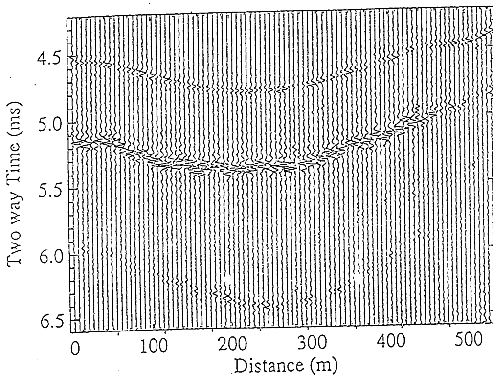
Figure: 7 Acoustic record made with a deconvolved 1.0 msec, 30--15 kHz sweep over the same region as that shown in Fig. 6.
