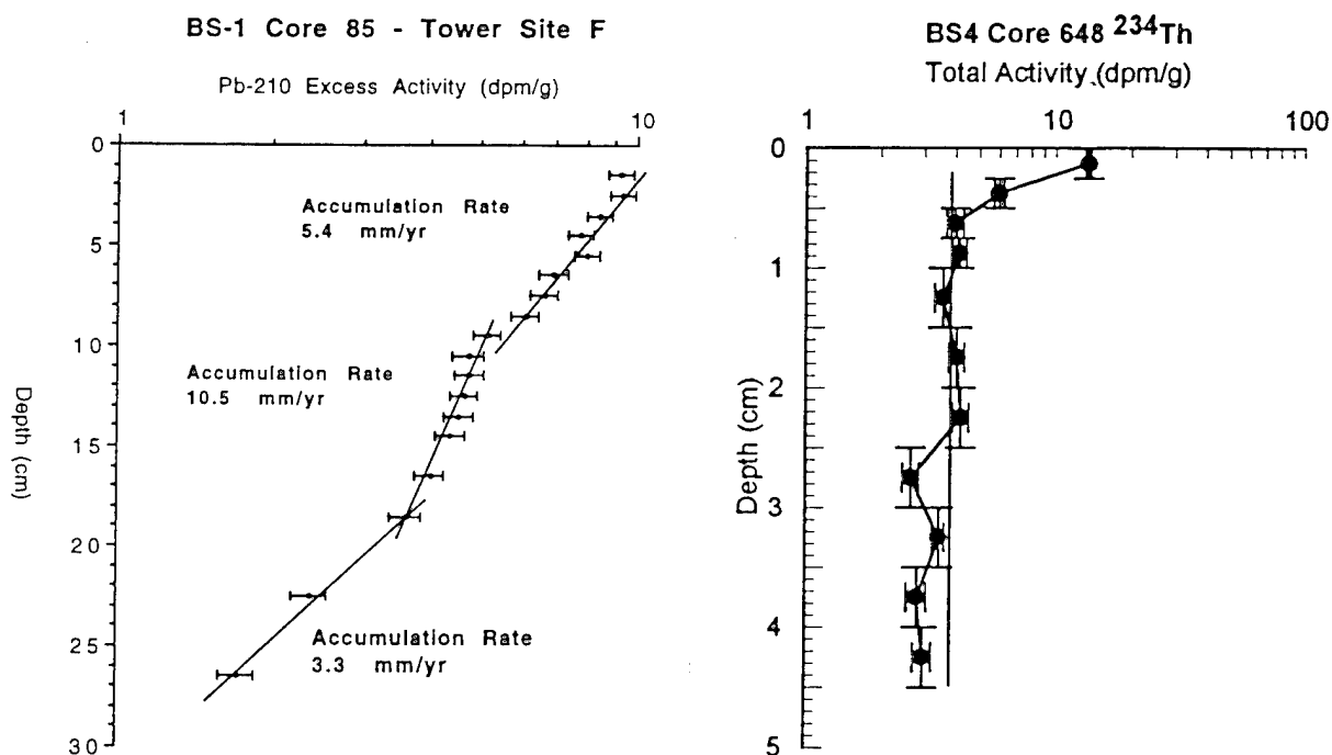
Fig. 4 Radiochemical profiles. A) Excess ^{210}\text{Pb} , BS1-85 (Station F, Fig. 2), note changes in accumulation rate through time; B) Total ^{234}\text{Th} , BS4-648, background levels are \sim 4 dpm/g and excess activities are restricted to the upper 5 mm.
