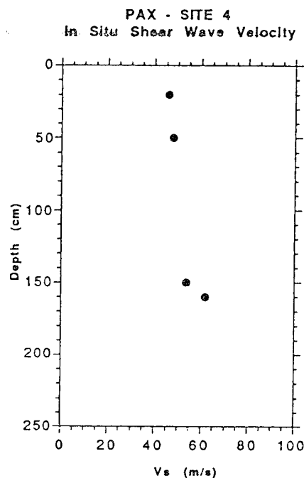
Figure 5. Shear wave velocity calculated from shear modulus values using a density of 1.25 \text{ g/cm}^3 from Site #4.
