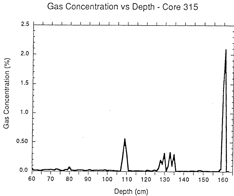
Figure 1. Depth Profile of Free Gas Volume Concentration Based on 3-D CT Scan Data Base for Backscattering Tower Site Core.
