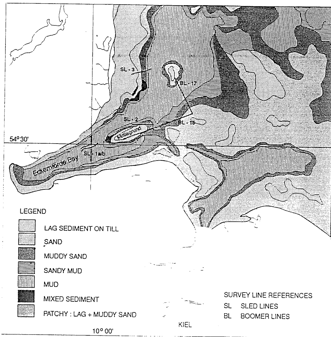
Fig.1 Location map showing UCNW's sled and Uniboam survey tracks in relation to sediment distribution
