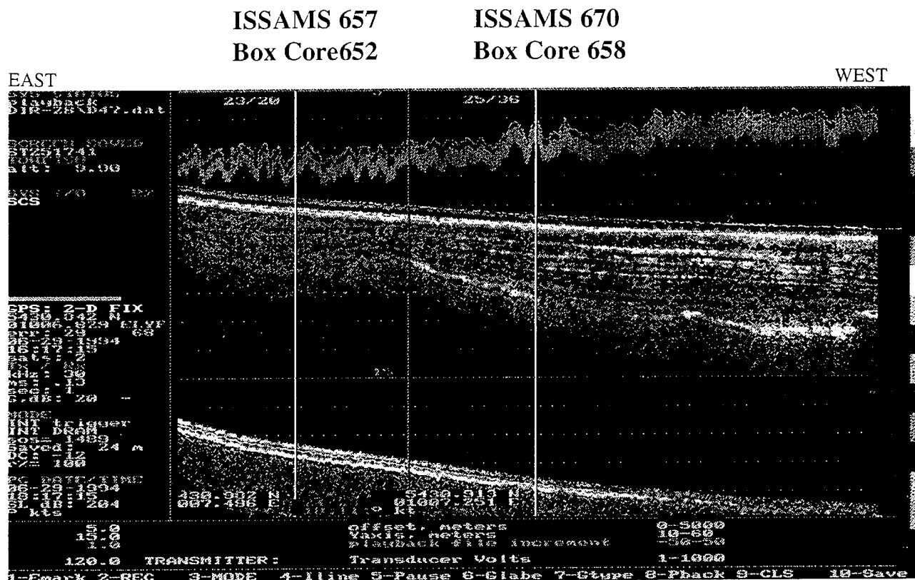
Figure 3a. ASCS 30 kHz seismic record across Line 47 showing the location of Core Site 658 and ISSAMS Site 670 in Eckernfoerder Bay, Germany
