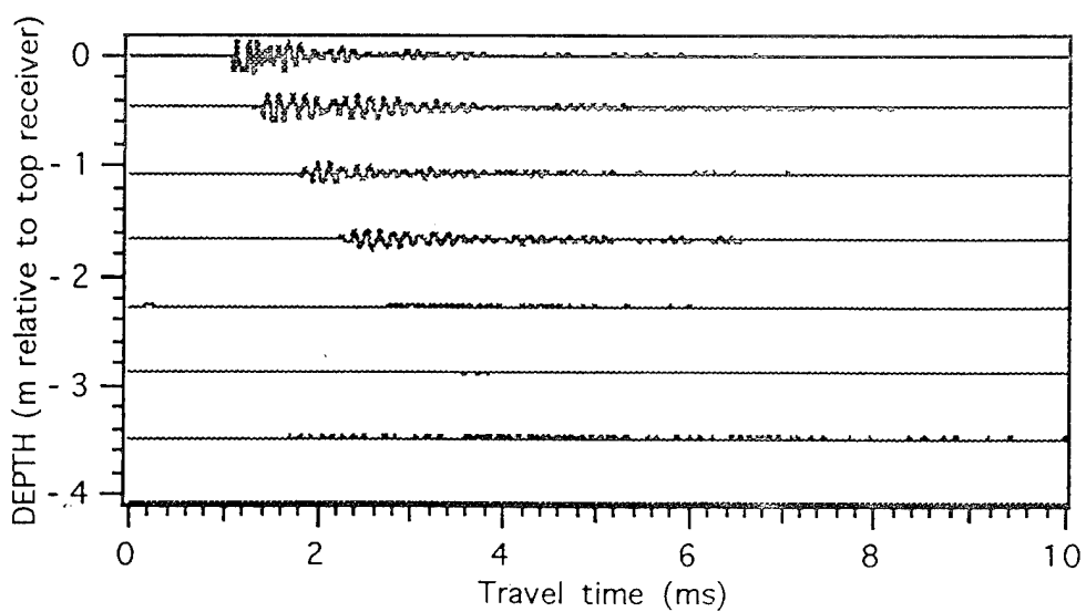
Signals received in gassy sediments (STN #625, normalized). Gassy layer start at 2.2 mbsf.
