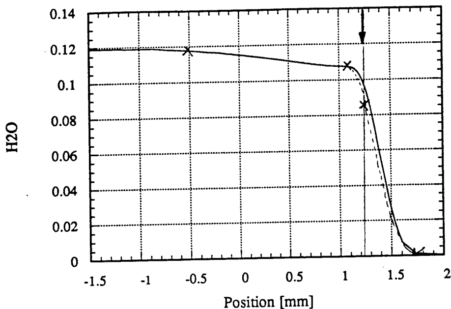
Figure 22. A comparison between the computed H_2O mass fraction profile for a highly strained atmospheric pressure, stoichiometric, methane-air flame employing a \lambda = 2.58 \cdot 10^{-4} c_p (T/T_u)' transport model and the "starting" chemistry mechanism (solid line) and the profile of Rogg [7] (dashed line). \epsilon = 10^3 \text{ s}^{-1} . The vertical arrow indicates the location of maximum fuel-consumption rate.
