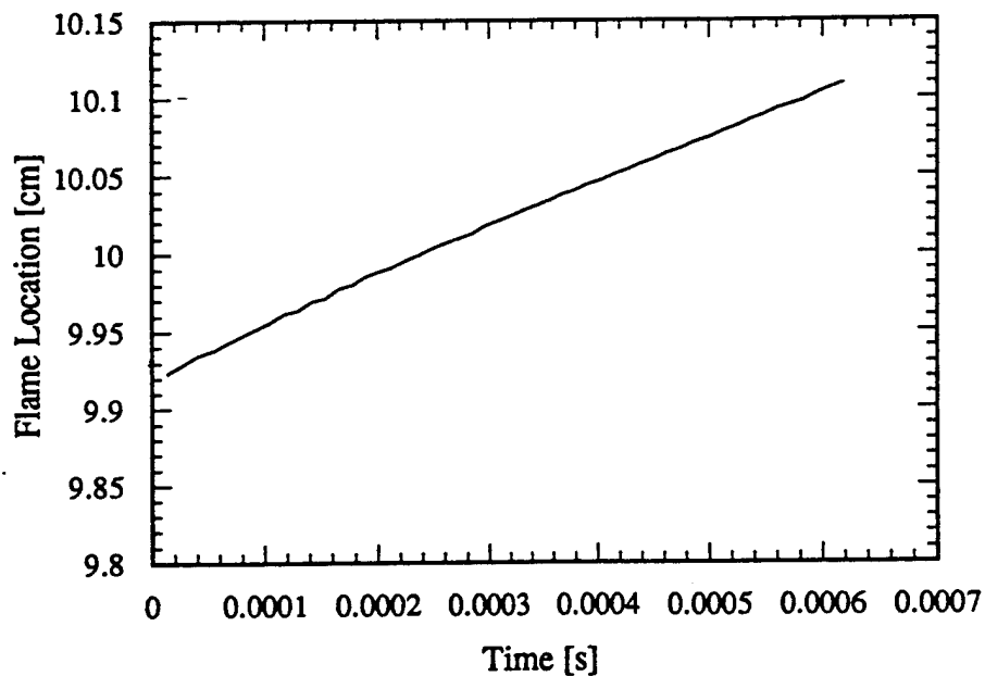
Figure 6c. The flame location of a freely-propagating, premixed, atmospheric pressure, stoichiometric flame as a function of time. Transport model \lambda = 2.58 \cdot 10^{-4} c_p (T/T_u)^r , r=0.7 , the "starting" chemical kinetics mechanism. Strain rate \epsilon = 10^{-4} \text{ s}^{-1} .
