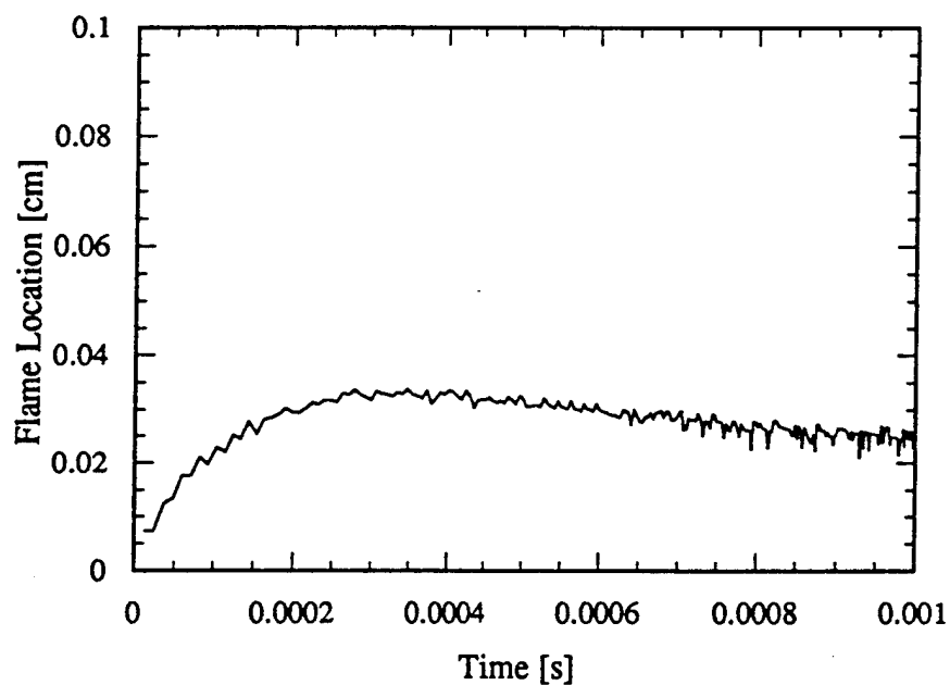
Figure 30. The flame location of a highly strained, premixed, atmospheric pressure, stoichiometric flame as a function of time. Transport model \lambda = 2.58 \cdot 10^{-4} c_p (T/T_u)^r , the "starting" chemical kinetics mechanism; two-zone strain, y_* = y_f(t) . Strain rate \epsilon_u = 10^3 \text{ s}^{-1} .
