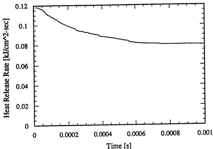
Figure 16c. The heat release rate of a strained, premixed, atmospheric pressure, stoichiometric flame as a function of time. Transport model \lambda = 2.58 \cdot 10^{-4} c_p (T/T_w)' , r=0.7 , the "starting" chemical kinetics mechanism. Strain rate \epsilon = 10^3 \text{ s}^{-1}
