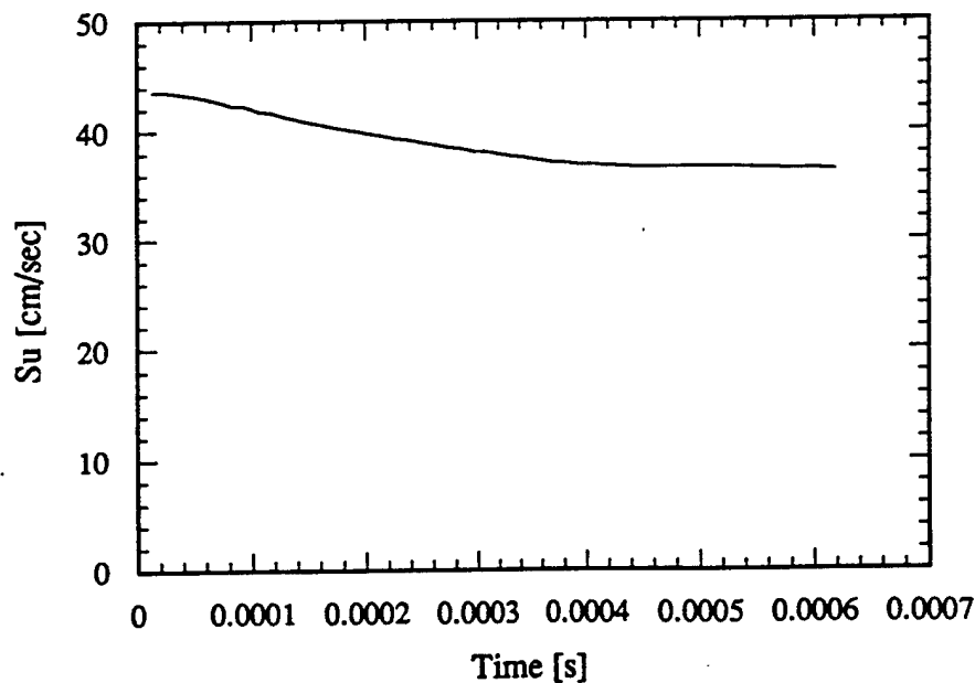
Figure 6a. The laminar burning velocity of a freely-propagating, premixed, atmospheric pressure, stoichiometric flame as a function of time. Transport model \lambda = 2.58 \cdot 10^{-4} c_p (T/T_u)^r , the "starting" chemical kinetics mechanism. Strain rate \varepsilon = 10^{-4} \text{ s}^{-1}
