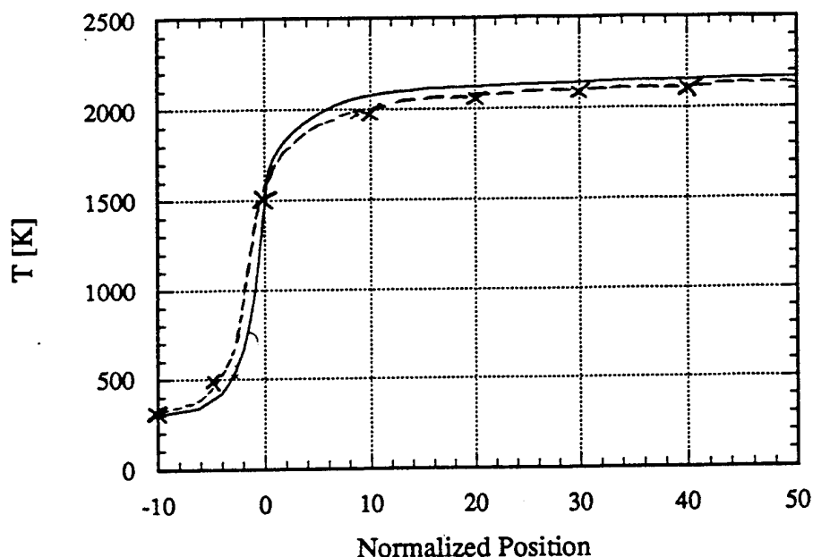
Figure 7. A comparison between the computed temperature profiles as a function of the normalized distance for an atmospheric pressure, stoichiometric, methane-air flame employing a \lambda = 2.58 \cdot 10^{-4} c_p (T/T_u)' transport model and the "starting" chemical kinetics mechanism (solid line); and the profiles obtained by Smooke [2] (dashed line).
