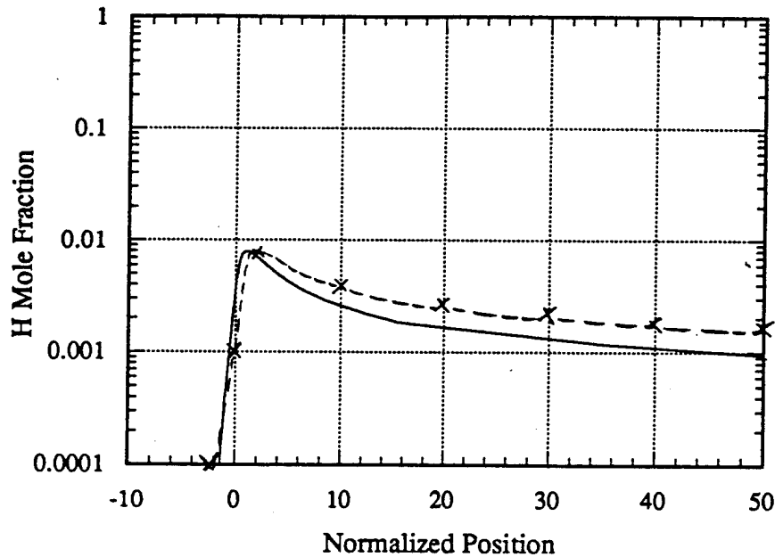
Figure 15. A comparison between the computed H mole fraction profiles as a function of the normalized distance for an atmospheric pressure, stoichiometric, methane-air flame employing a \lambda = 2.58 \cdot 10^{-4} c_p (T/T_u)^r transport model and the "starting" chemical kinetics mechanism (solid line); and the profiles obtained by Smooke [2] (dashed line).
