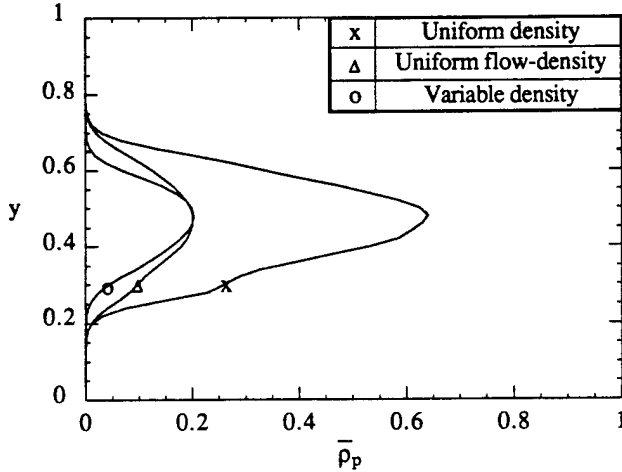
Figure 6. The time-averaged product density profiles of the uniform density, uniform flow-density and variable density unforced cases at x=5 .
