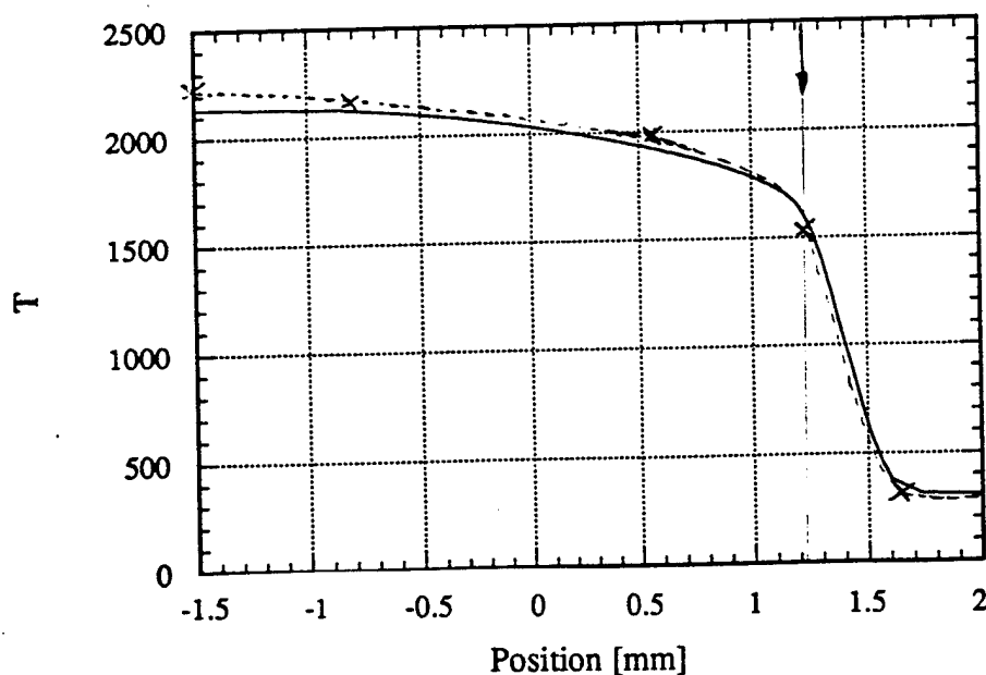
Figure 17. A comparison between the computed temperature profile for a highly strained atmospheric pressure, stoichiometric, methane-air flame employing a \lambda = 2.58 \cdot 10^{-4} c_p (T/T_w)' transport model and the "starting" chemistry mechanism (solid line) and the profile of Rogg [7] (dashed line). \epsilon = 10^3 \text{ s}^{-1} . The vertical arrow indicates the location of maximum fuel-consumption rate.
