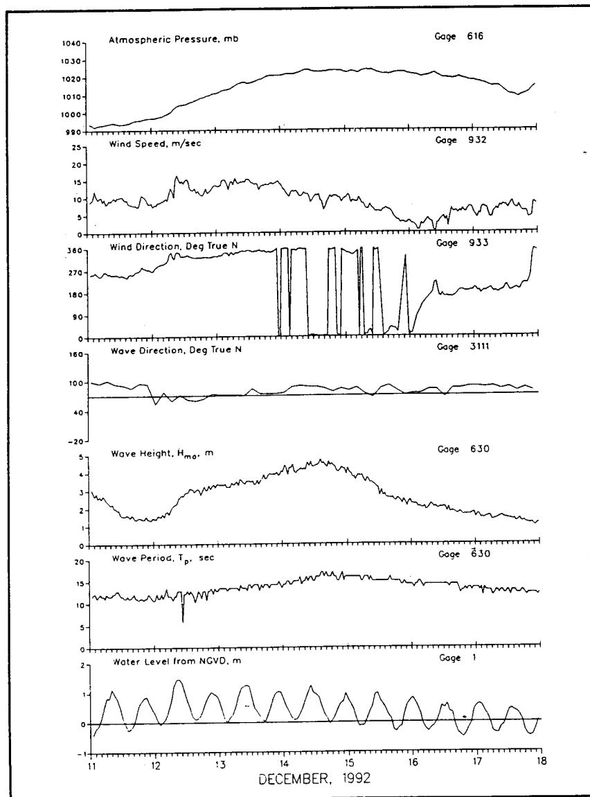
Figure 37. Data for 12-16 December 1992 storm
