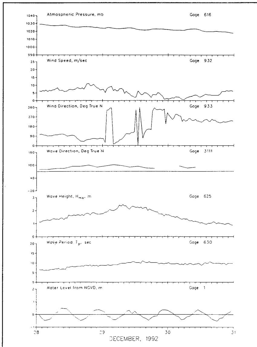
Figure 38. Data for 29 December 1992 storm
