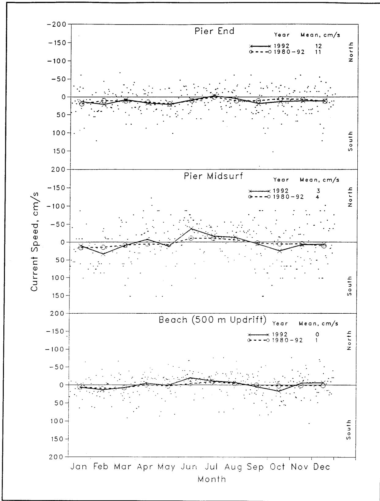
Figure 16. Daily current speeds and directions with monthly means for 1992
