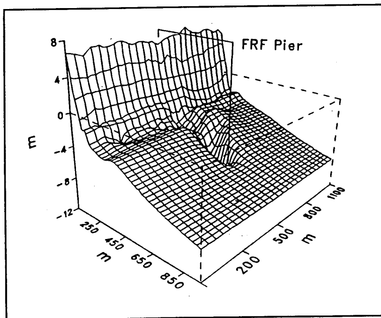
Figure 22. Permanent trough under the FRF pier, 24 January 1992
