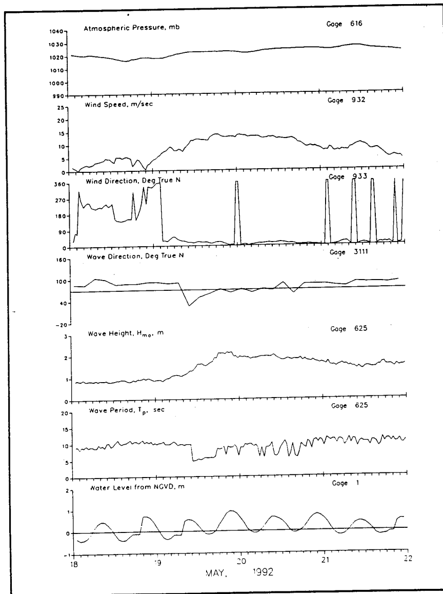
Figure 33. Data for 19-20 May 1992 storm
