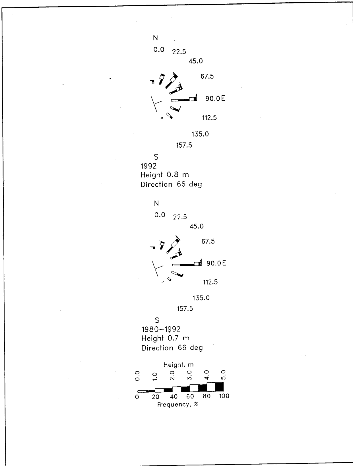
Figure 13. Annual wave roses
