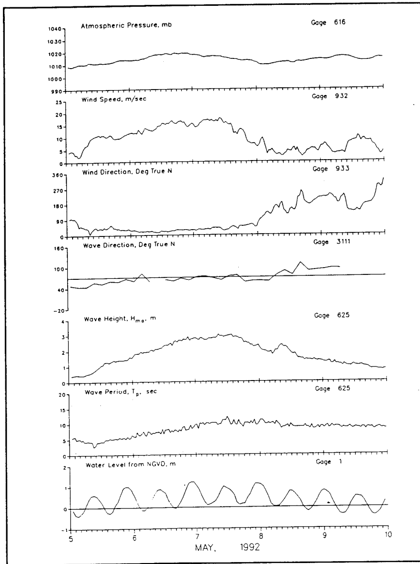
Figure 32. Data for 6-8 May 1992 storm
