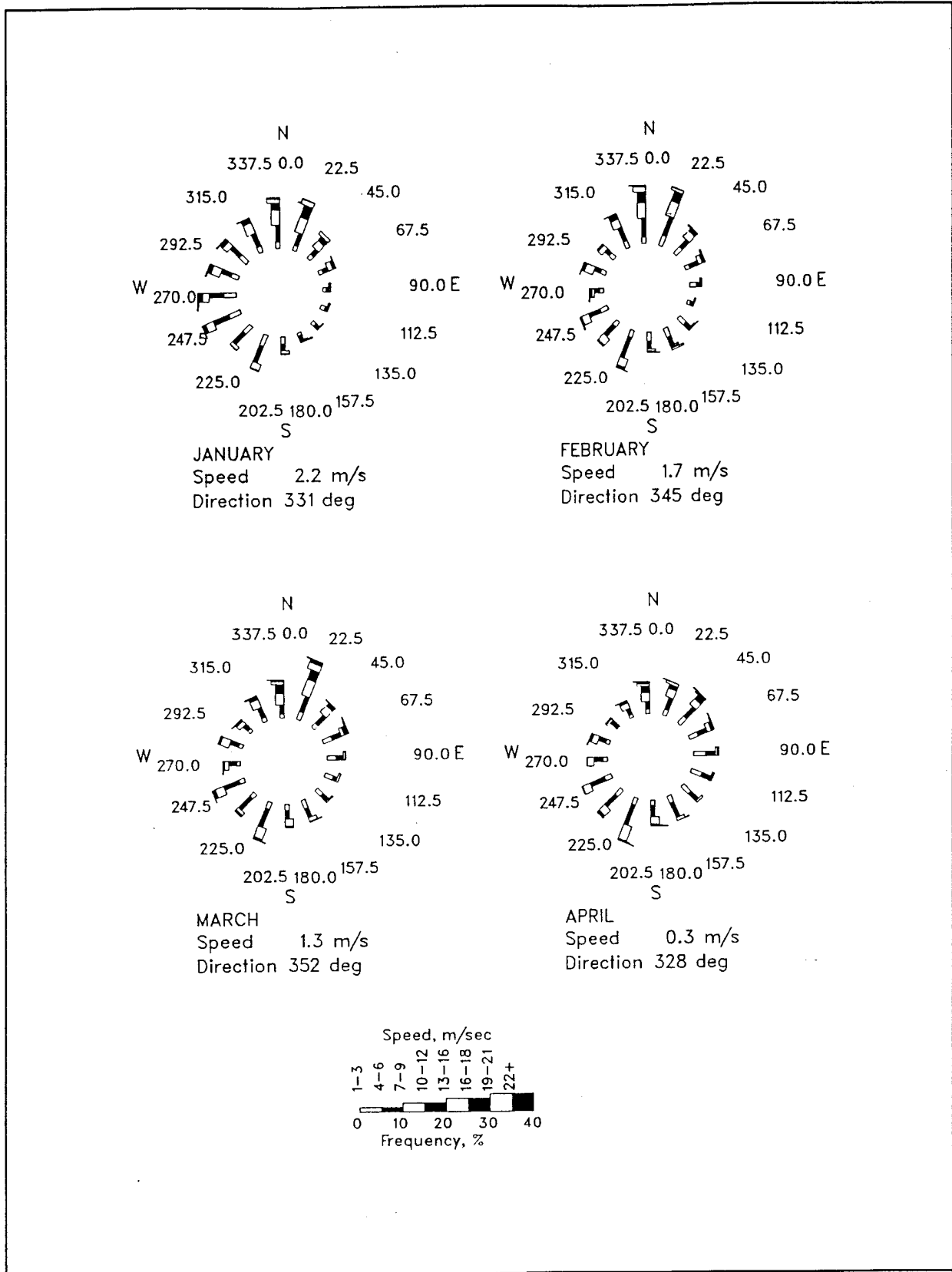
Figure 8. Monthly wind roses for 1980 through 1992 (Continued)
