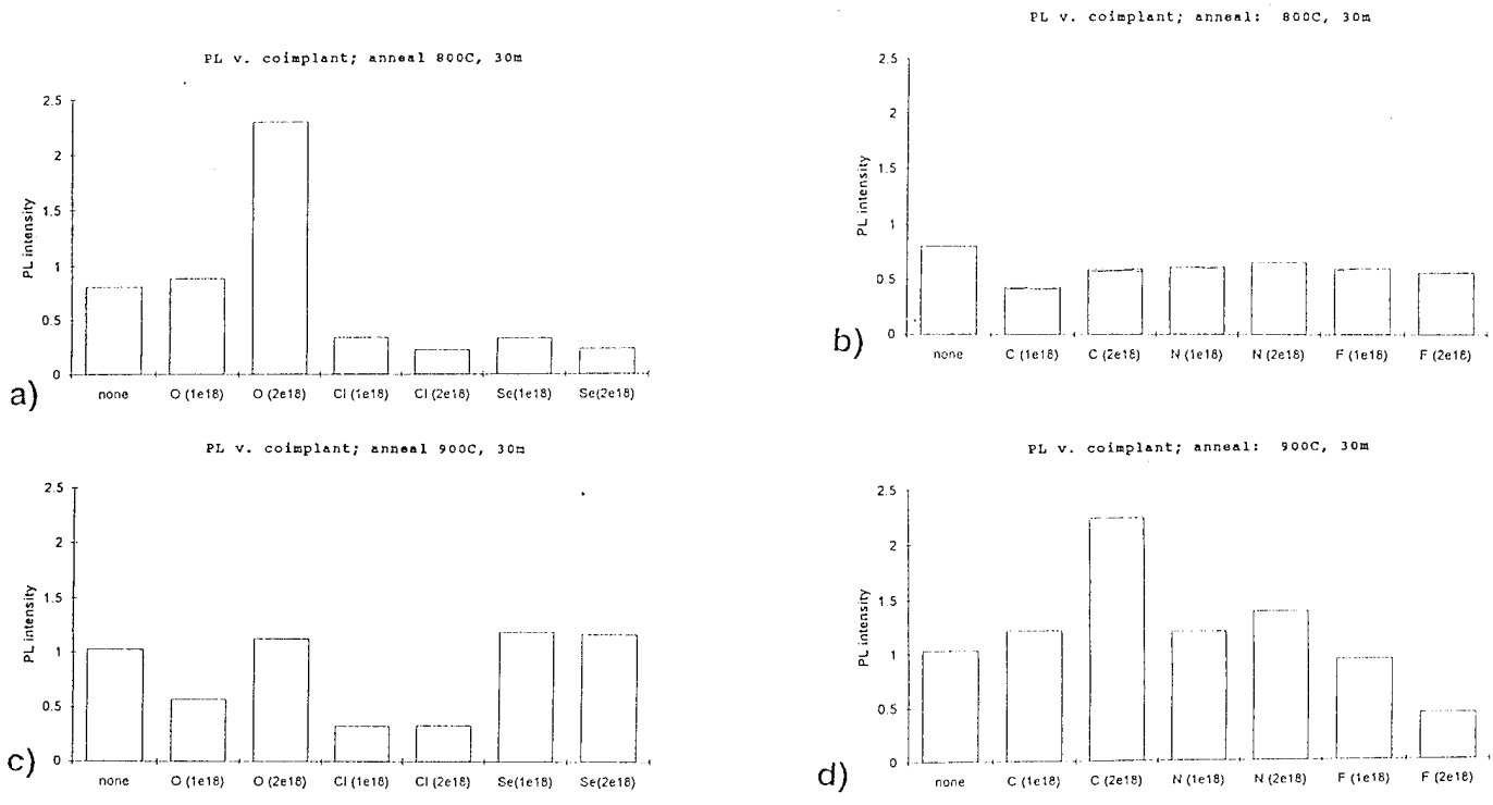
FIGURE 2 Photoluminescence results for 30 minute anneals at 800 and 900° C.
