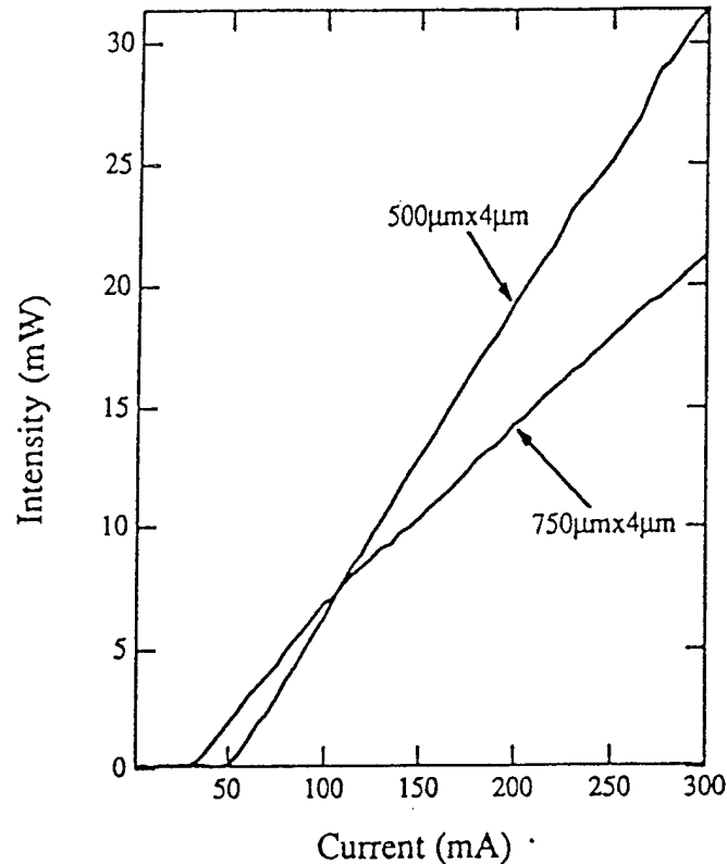
Figure 22. LI characteristic of a quantum well ridge laser etched using the low-damage cryogenic etching technique.
