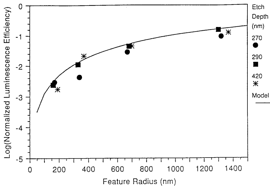
Fig. 29: Quantum box luminescence efficiency for quantum boxes etched to different depths using 400 W (75 V bias) MIE.
