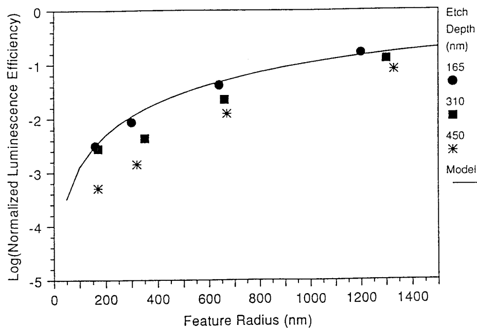
Fig. 28: Quantum box luminescence efficiency for quantum boxes etched to different depths using 200 W (30 V bias) MIE.
