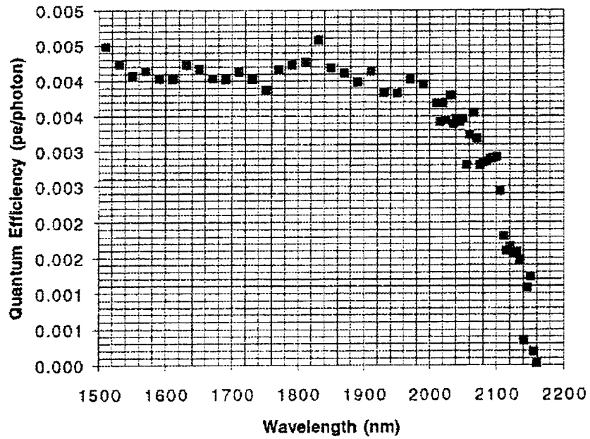
Figure 6: Responsivity and quantum efficiency for the 2.1 \mu m APD
