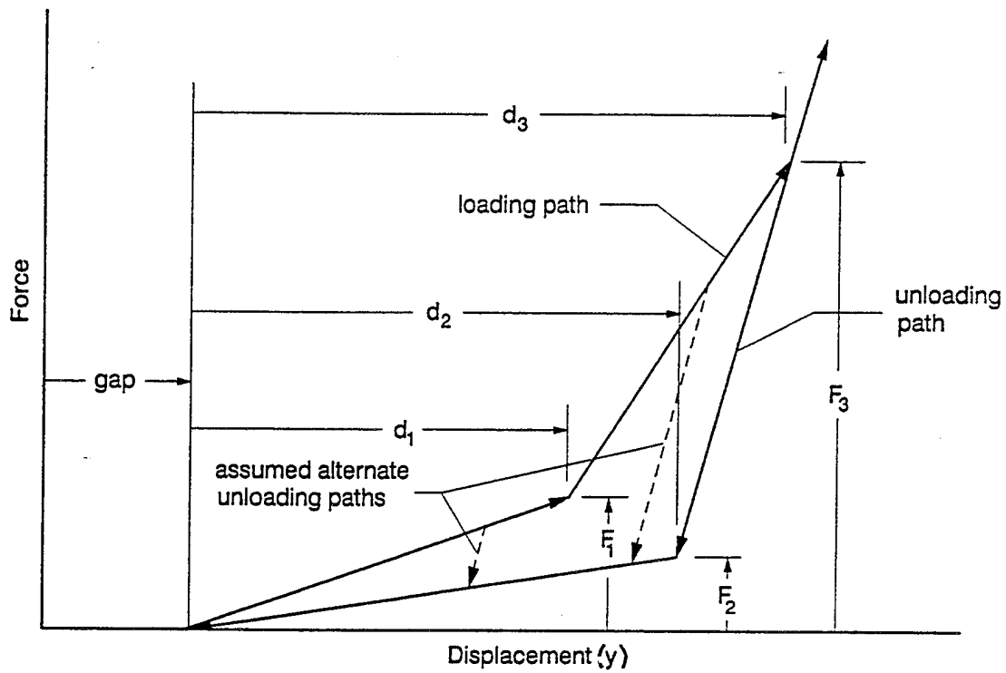
Figure D-2. Idealized Belleville spring behavior.
