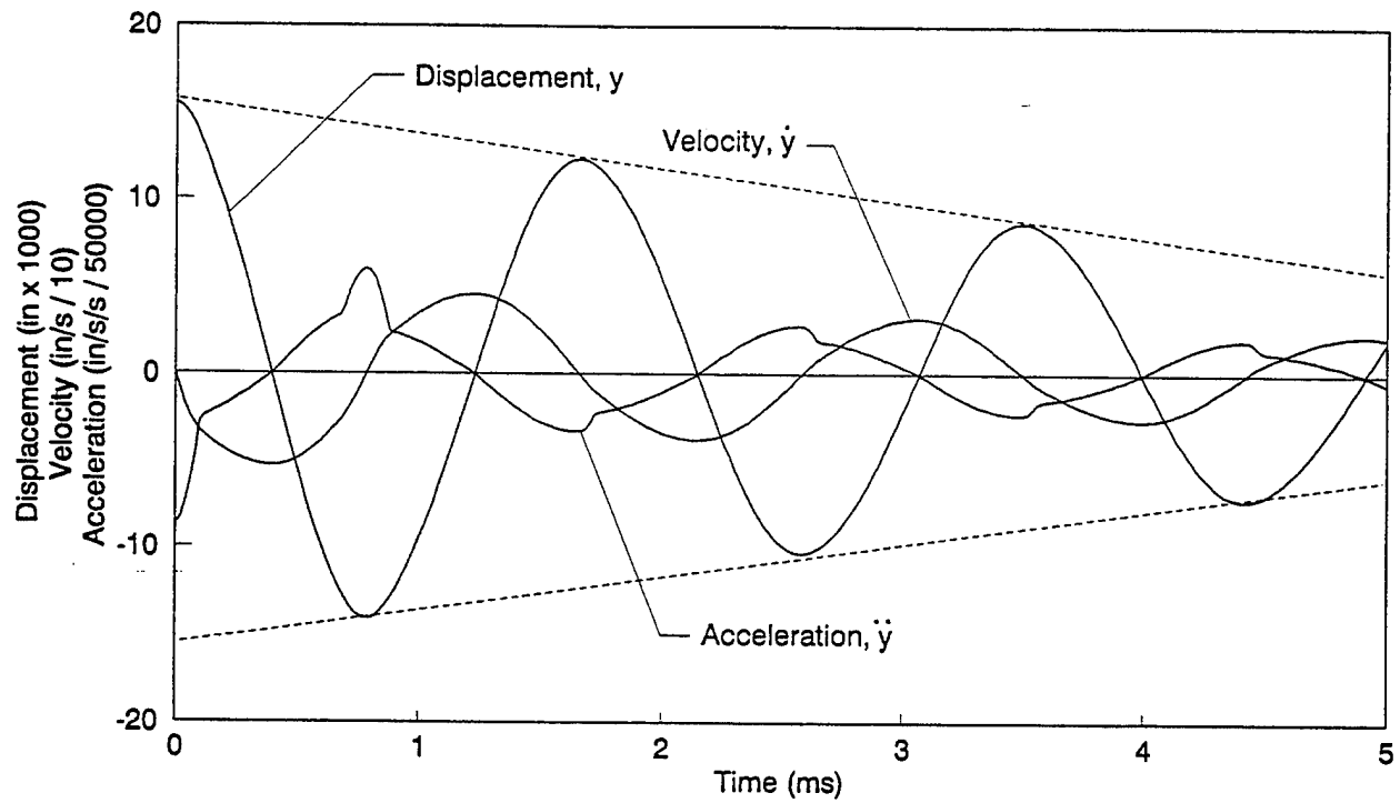
Figure C-5. Normal ringdown—closing Belleville washer.
