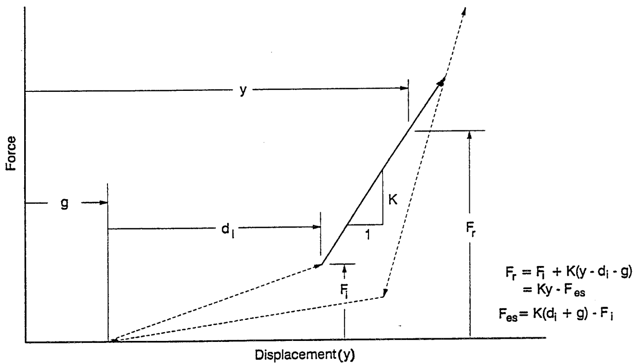
Figure D-3. Typical Belleville spring load segment restoring force.
