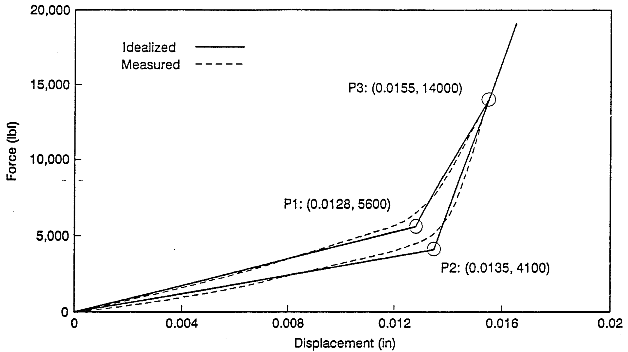
Figure D-4. Belleville closing spring stiffness characteristics.
