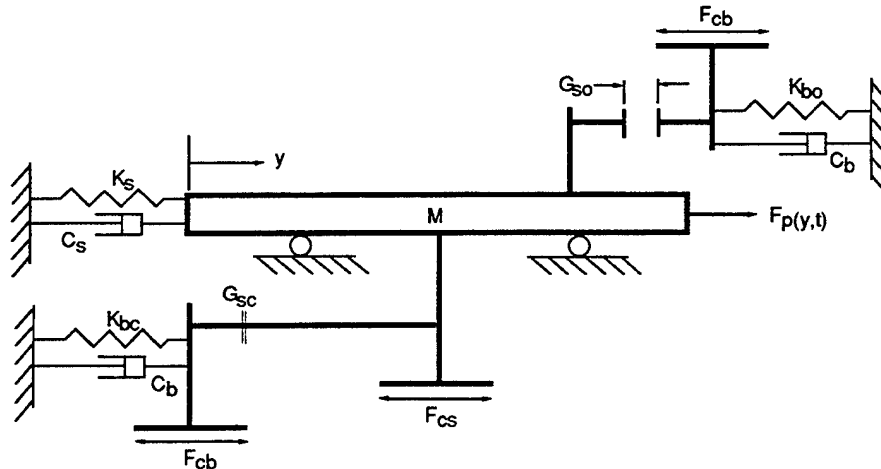
Figure D-1. ETVE mechanical motion model.
