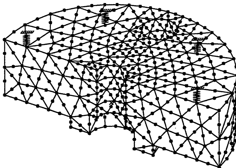
Figure 3. Model of Stop Plate (Isometric View)
