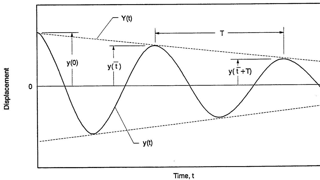
Figure C-2. Typical Belleville washer damping behavior.
