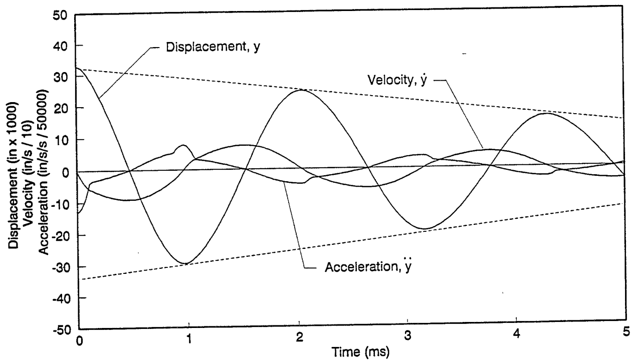
Figure C-3. Normal ringdown—opening Belleville washer.
