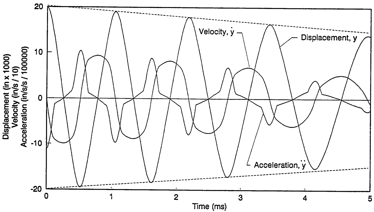
Figure C-5. Overload ringdown—closing Belleville washer.
