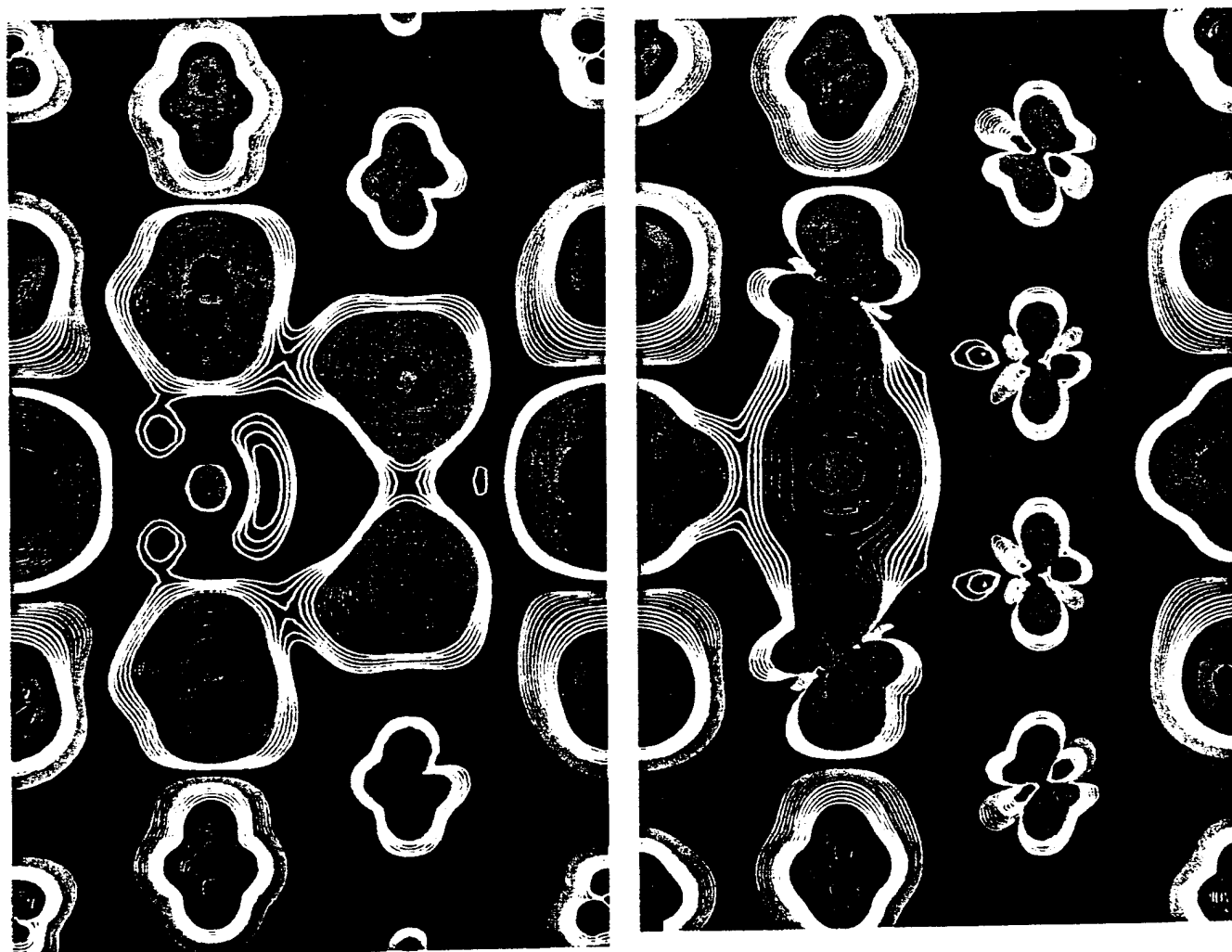
FIG. 4. The calculated spin density difference for (a) P/Fe and (b) B/Fe GB. Contours start from 1 \times 10^{-3} e/a.u. 3 and increase successively by a factor of 2^{\frac{1}{4}} ; green, yellow, red and pink colors denote positive differences and light and dark blue colors denote negative differences.
