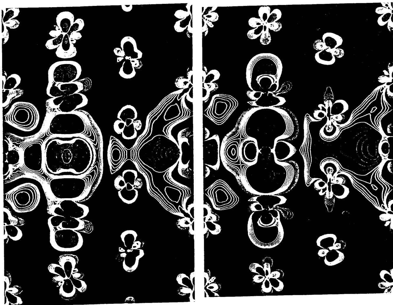
FIG. 3. The calculated valence charge density difference for (a) P/Fe and (b) B/Fe GB. Contours start from 1 \times 10^{-3} e/a.u.^3 and increase successively by a factor of 2^{\frac{1}{4}} ; green, yellow, red and pink colors denote positive differences and light and dark blue colors denote negative differences.
