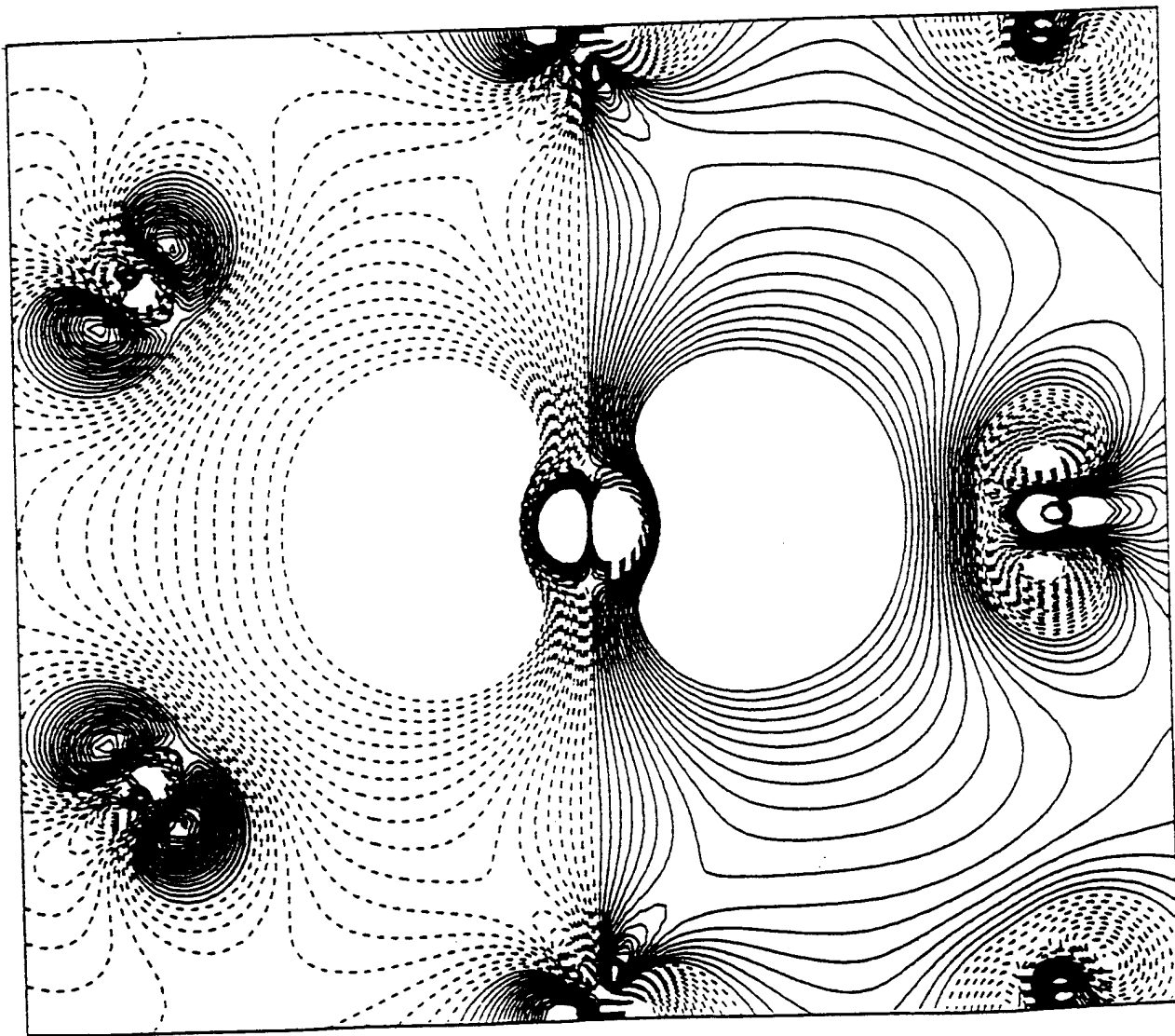
FIG. 3. Contour plot of molecular orbitals for S in the Fe GB. The contour spacing is 0.004. (b)
