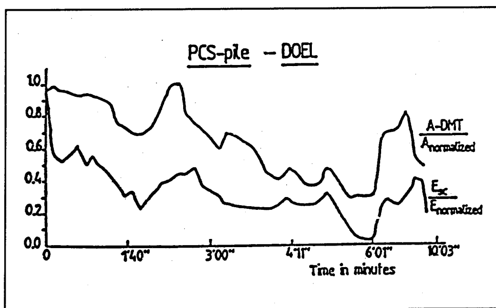
Figure 6. PCS-installation energy function as compared to DMT A-readings
