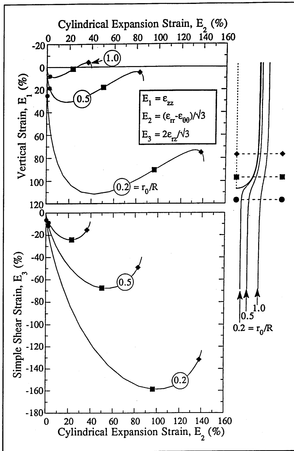
Figure 1a. Strain paths during simple pile penetration (after Baligh, 1985)
