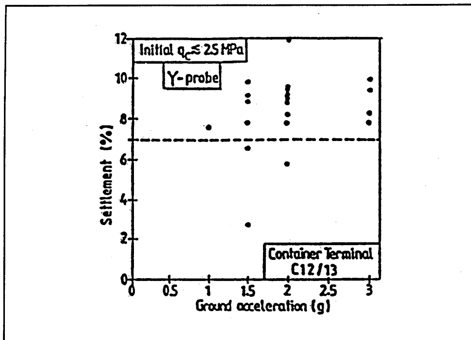
Figure 13. Ground surface settlements due to resonant compaction
