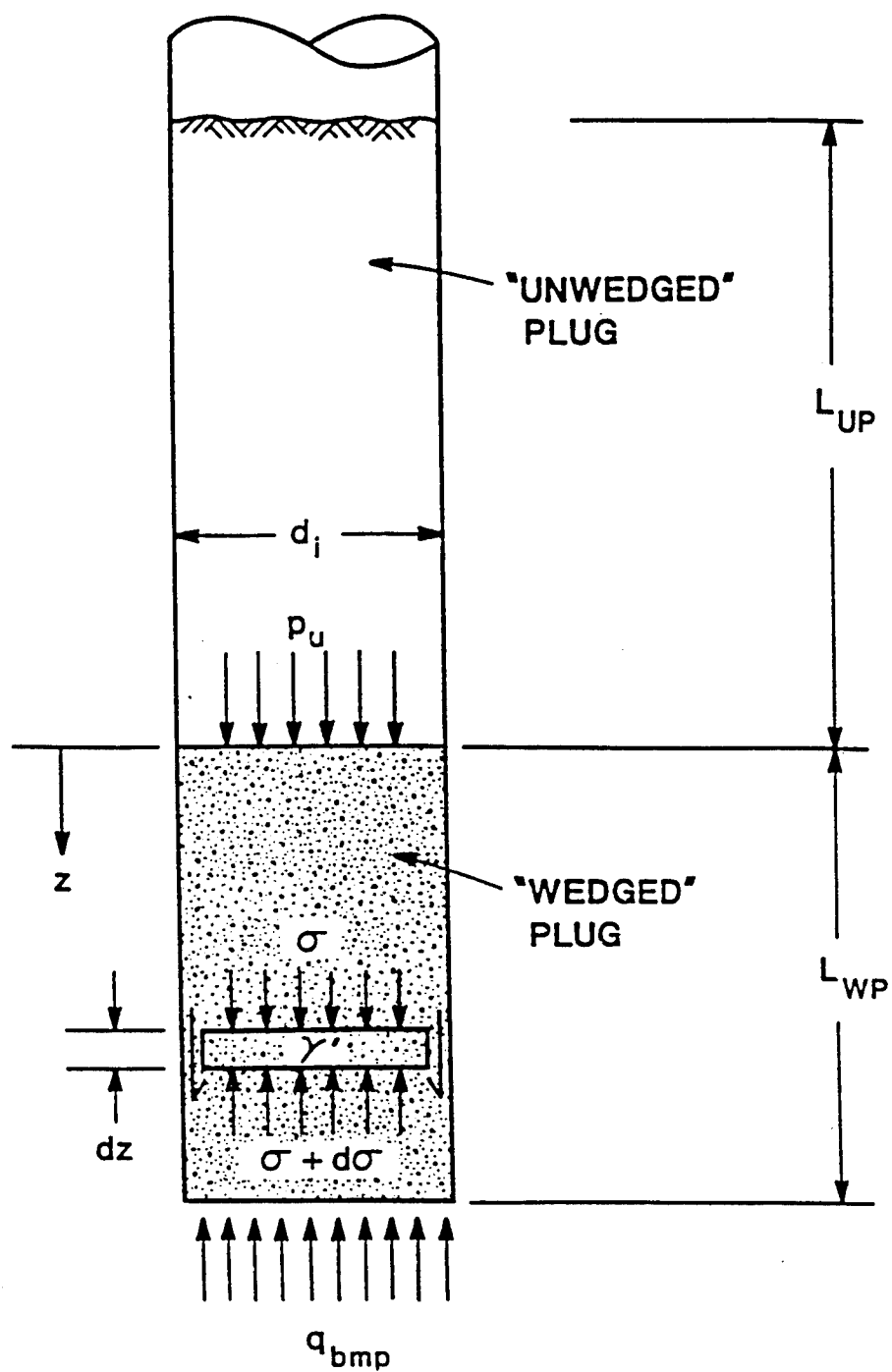
FIG. 12. Schematic Definition Diagram for Plug Equations
