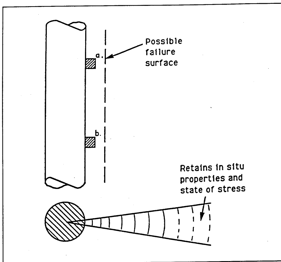
Figure 3. Variation of state of stress and soil properties around a driven pile
