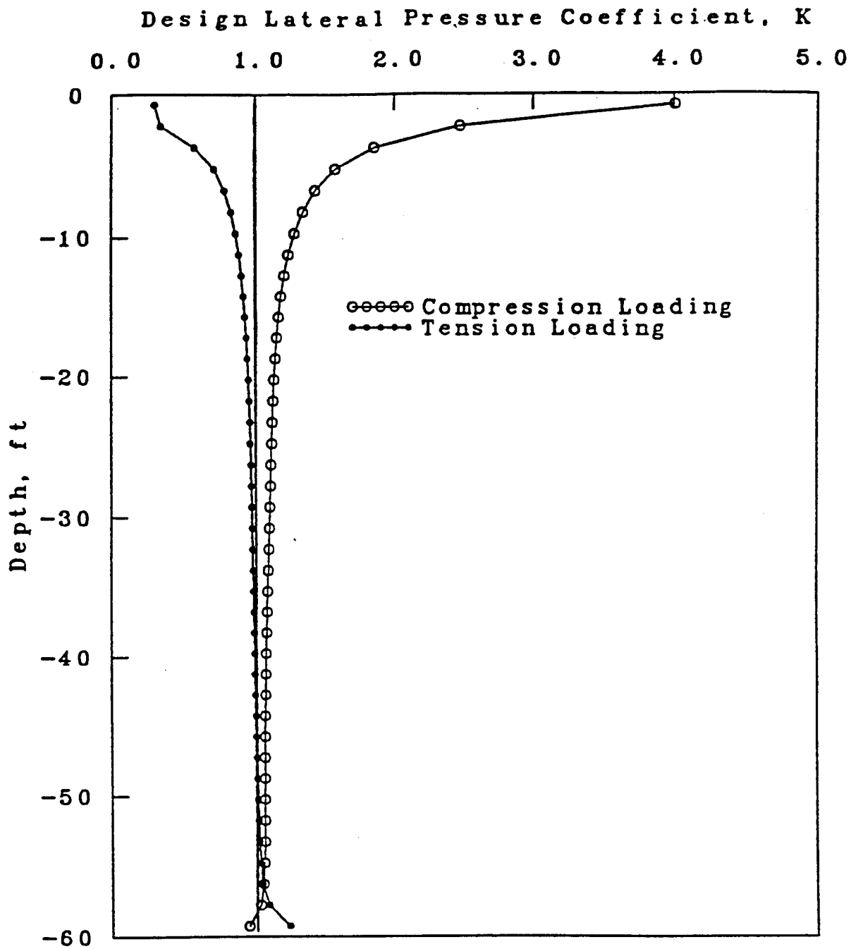
FIG. 65. K (Eq. 4) VS. DEPTH, 60-FT PILE, COMPRESSION VS. TENSION, DENSE SAND, NONDILATANT CASE, K_0 = 1
