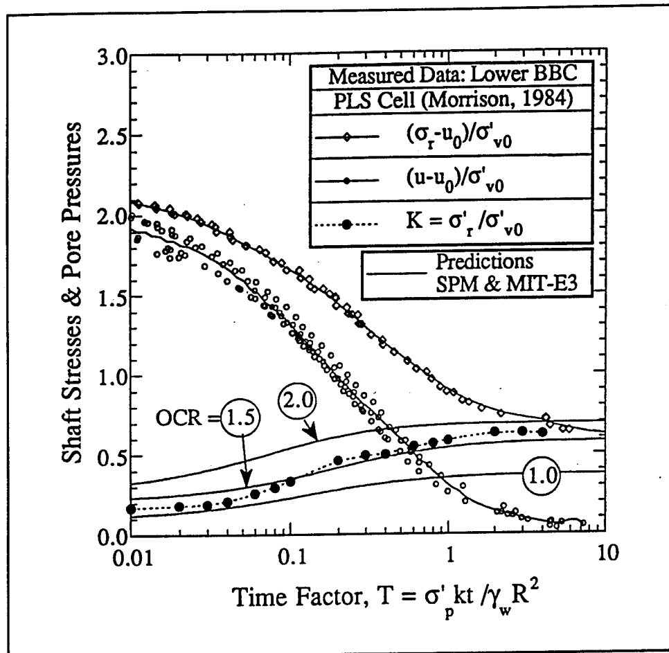
Figure 10. Evaluation of effective stress set-up in lower BBC
