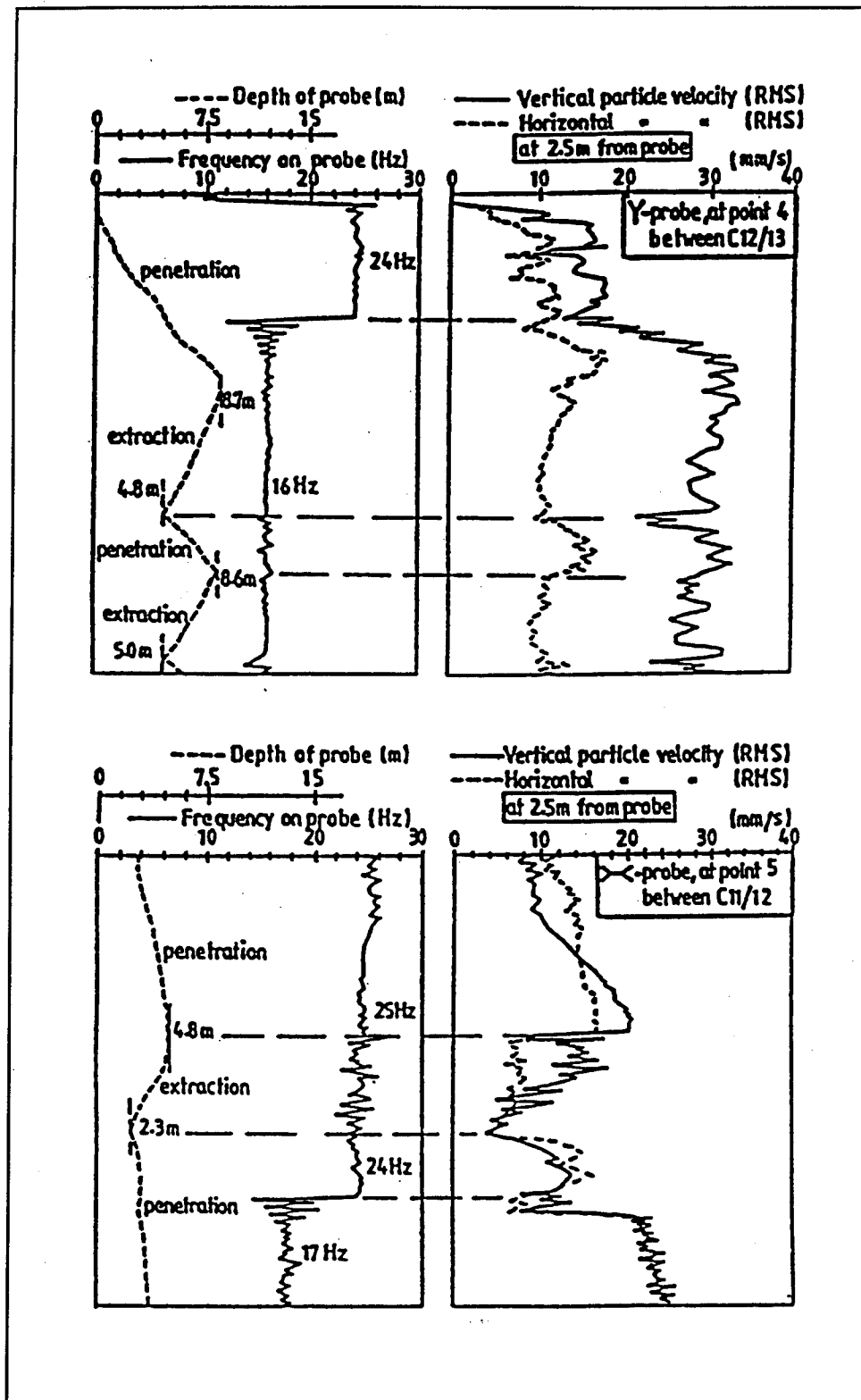
Figure 6. Part of resonant compaction procedure at container terminal test site
