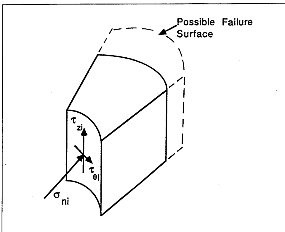
Figure 4. Generalized state of stress at interface of pile and soil
