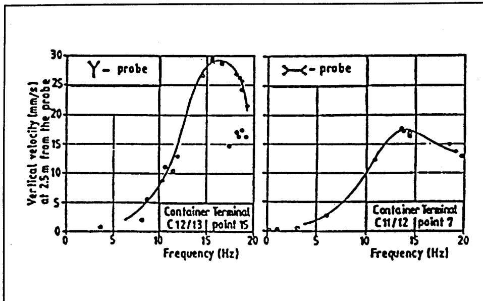
Figure 4. Frequency spectrum-vertical particle velocity peaks, for the two probes
