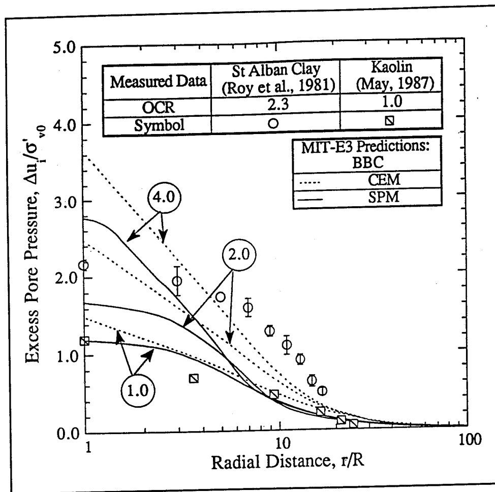
Figure 6. Distribution of excess pore pressures during installation
