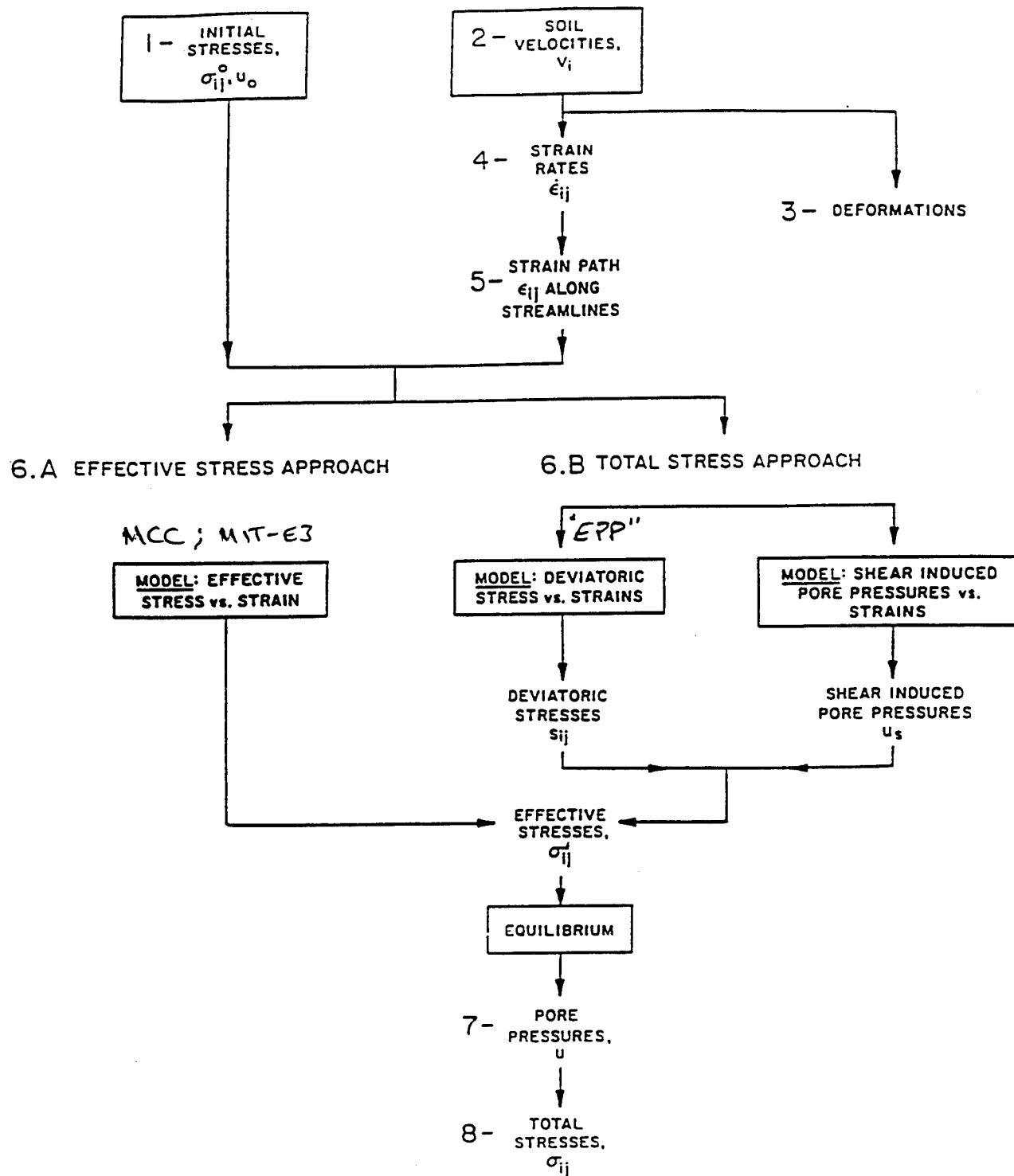
The Strain Path Method (Baligh, 1985)
