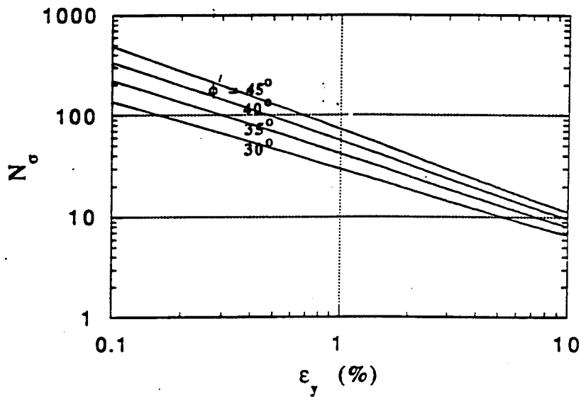
(b) Point Resistance Factor Versus Axial Yield Strain
