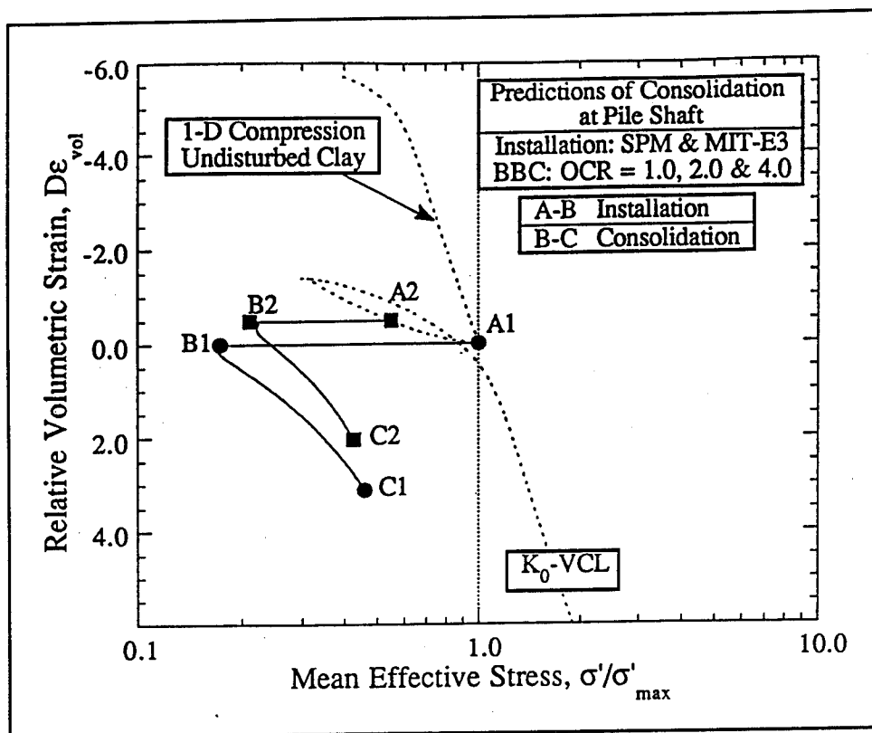
Figure 12. Predicted volumetric behaviour of soil elements adjacent to the pile shaft
