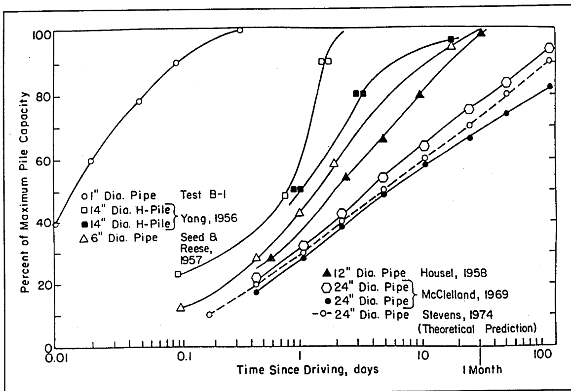
Figure 1. Pile diameter versus time to 50 percent consolidation (log-log plot) (after Grosch and Reese 1980) 1 in. = 25.4 mm
