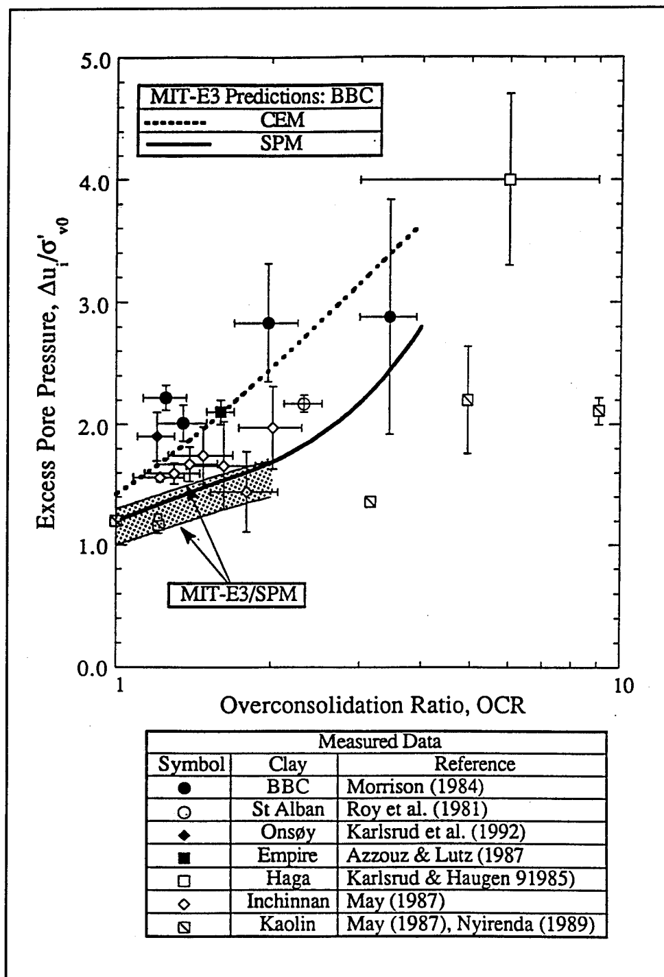
Figure 5. Evaluation of installation pore pressures at pile shaft
