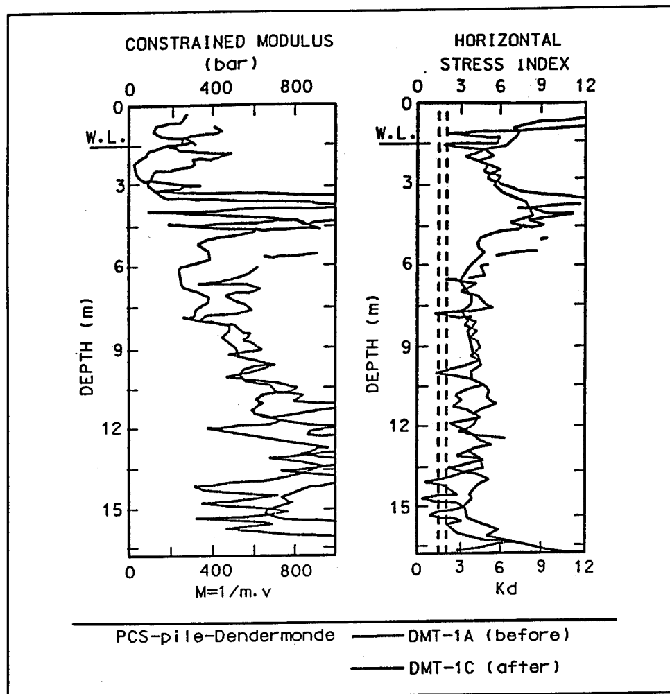
Figure 1a. DMT results at Dendermonde
