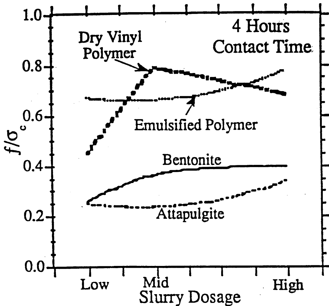
Comparison of mean normalized perimeter shear for 4 hours contact time.
