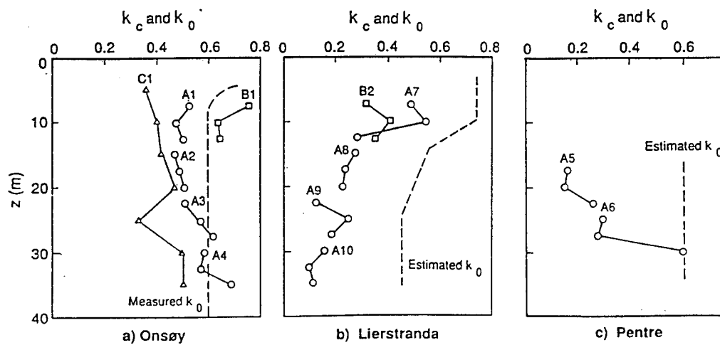
K_c at Three Sites (Karlsrud, Kalsnes & Nowacki, 1992)
