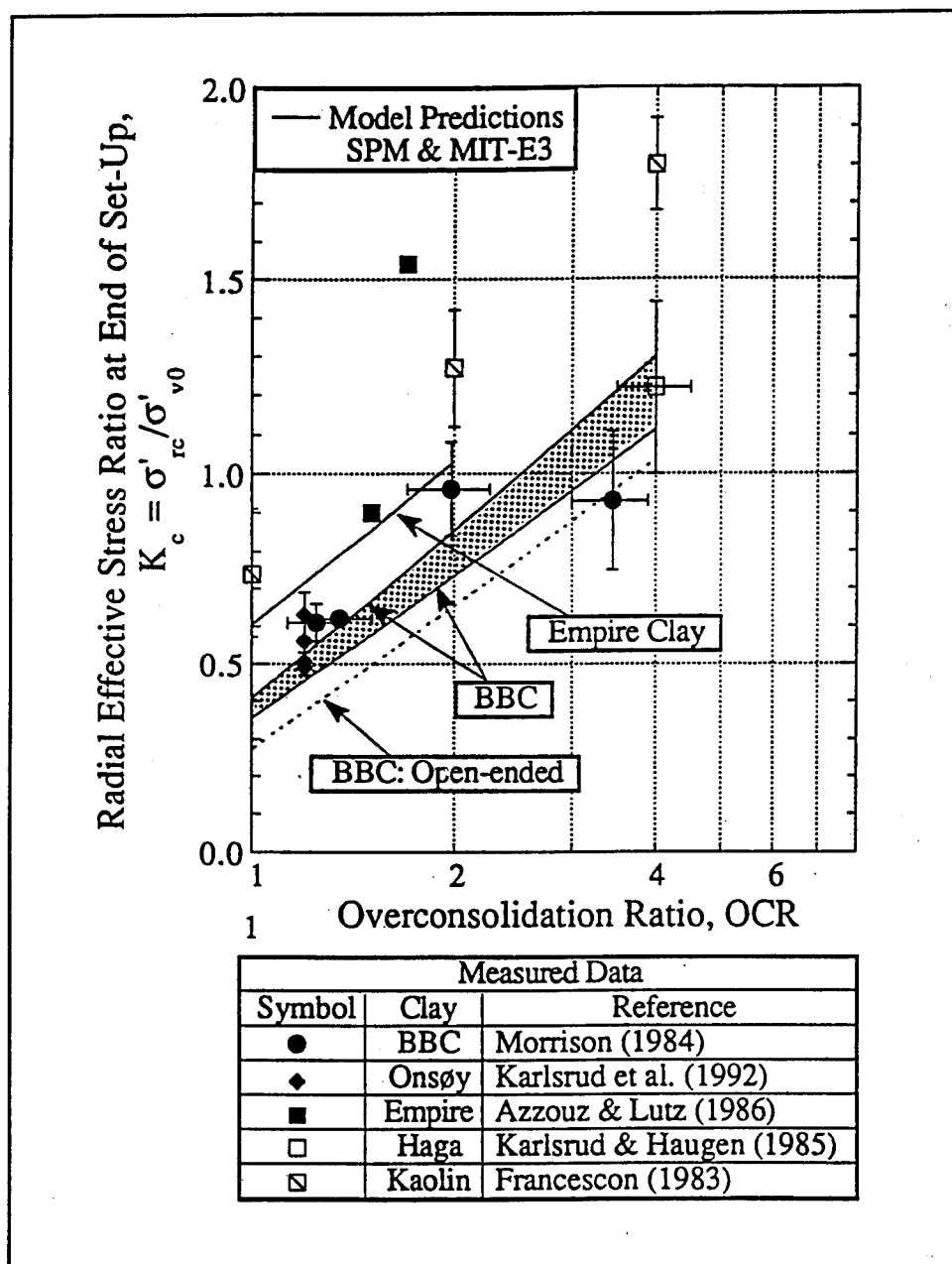
Figure 8. Evaluation of radial stress at end of set-up
