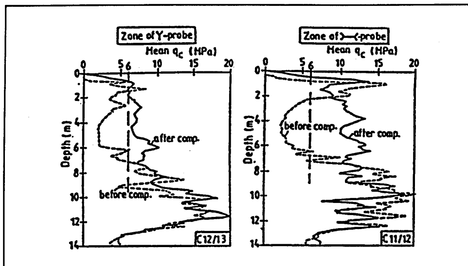
Figure 10. Average densifying efficiency from cone resistances
