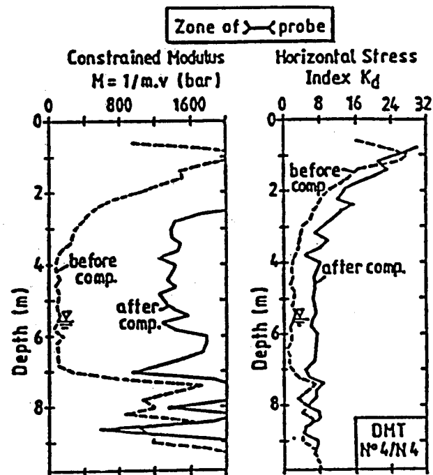
b. DMT-comparison before and after resonant compaction at container terminal (C11/12)
