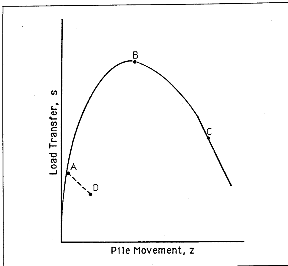
Figure 7. Hypothetical movement-softening load-transfer curve
