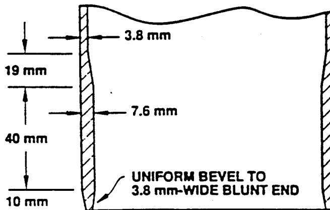
DOUBLE-BEVEL TOE (DB)
