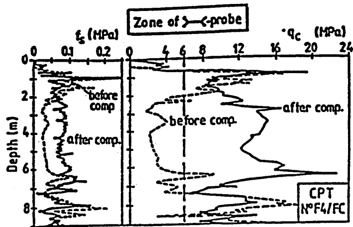
a. CPT cone and friction resistance comparison at container terminal before and after resonant compaction (C11/12)
