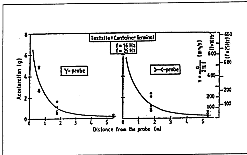
Figure 7. Attenuation of ground acceleration with distance from the probes
