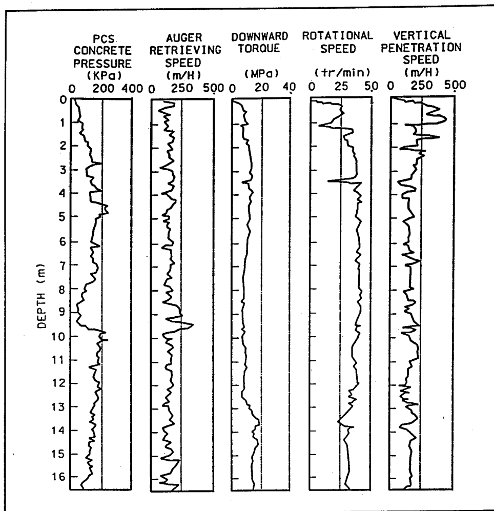
Figure 2. PCS-pile installation parameters at Dendermonde test site
