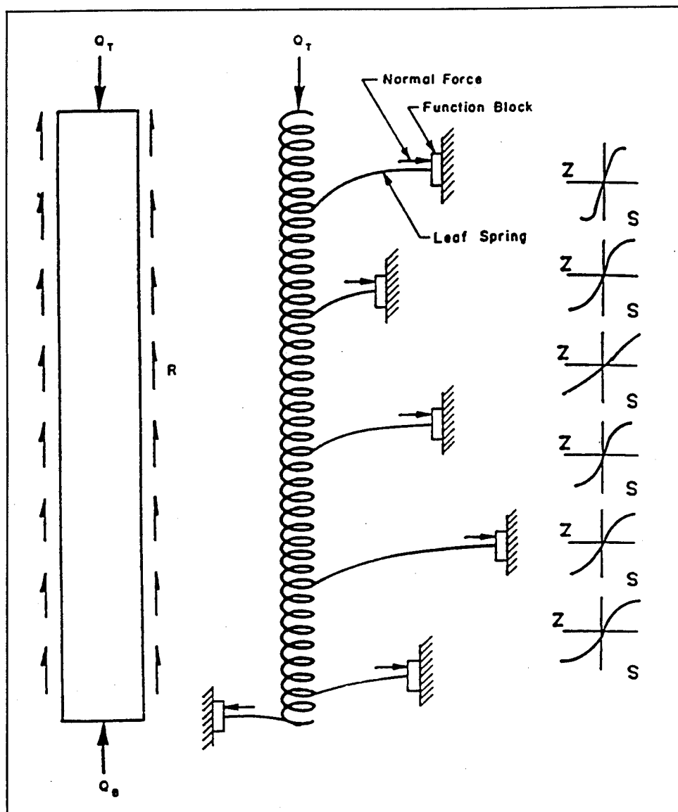
Figure 6. Model of axially loaded pile (after Reese 1964)
