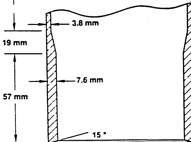
FLAT-BEVEL TOE (FB)
