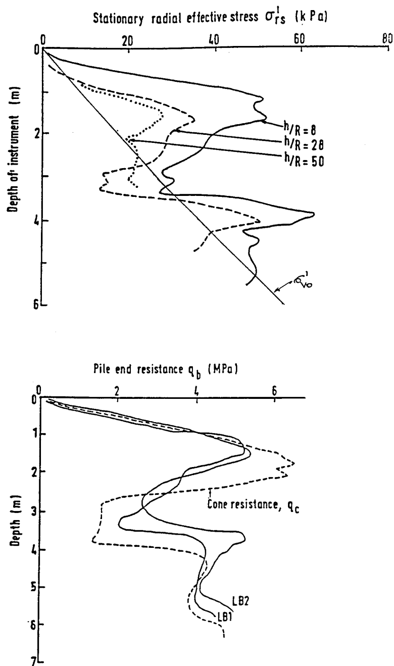
Radial Effective Stress and Tip Resistance (ICP test in Labenne Sand, Lehane, 1992)
