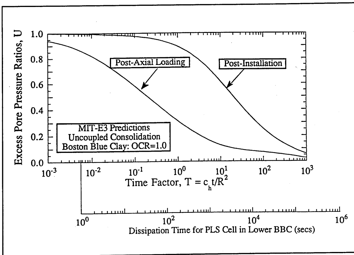
Figure 13. c) Dissipation of excess pore pressures
