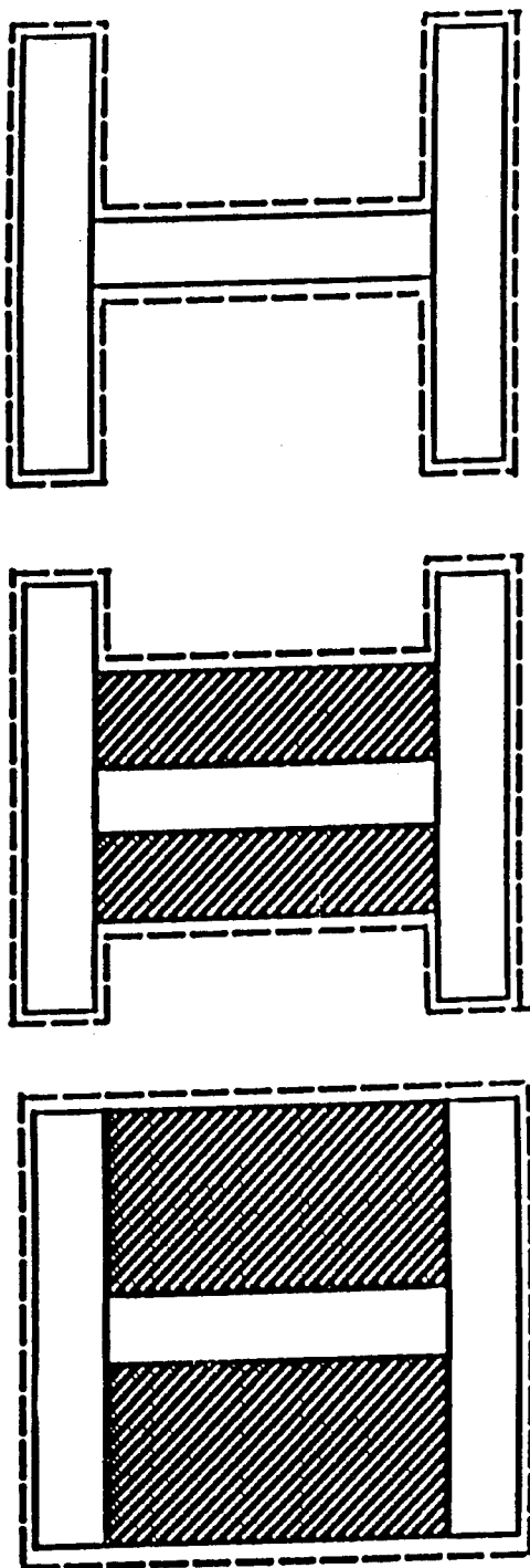
A) Fully Plugged B) Half Plugged C) No Plug ( Assumed for the Present Study) (per Coyle, 1989)
