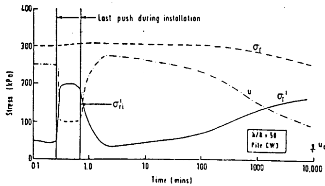
Set-Up Measurements in Cowden Till (Lehane, 1992)
