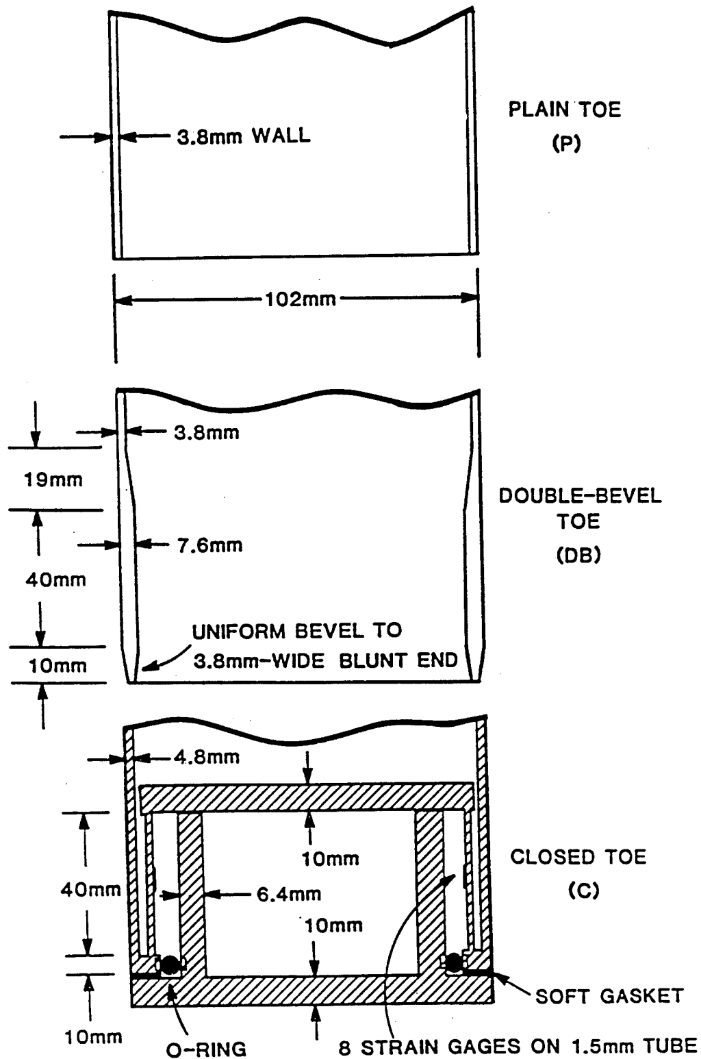
FIG. 3. Schematic of Pile Toes
