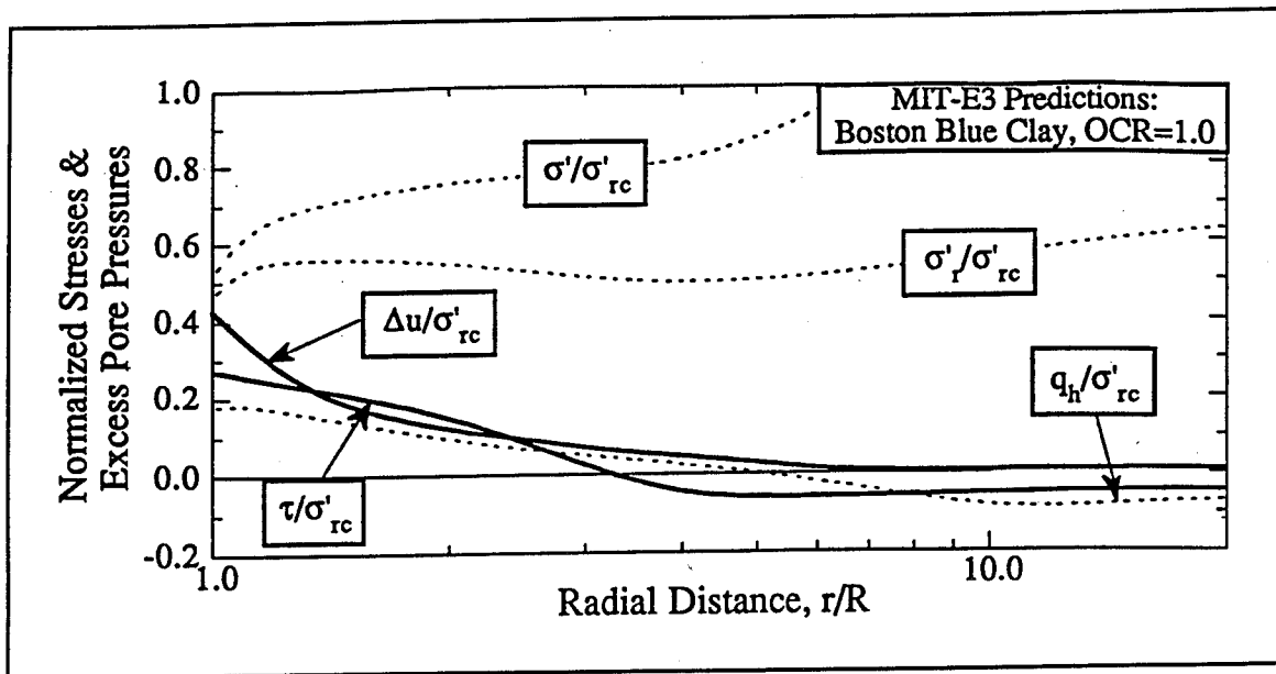
Figure 13. b) Radial distribution of stresses and excess pore pressures at peak shear resistance
