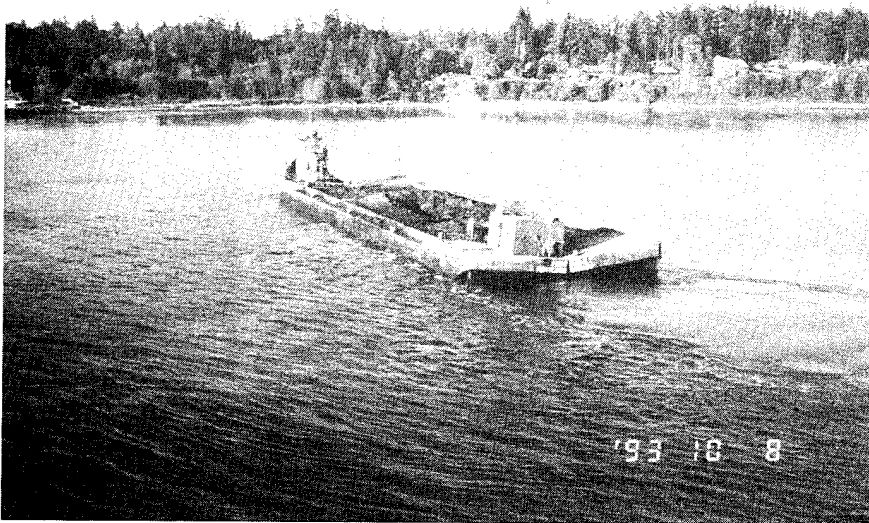
Figure 2. Placement in Area 1 using a bottom-dump barge
