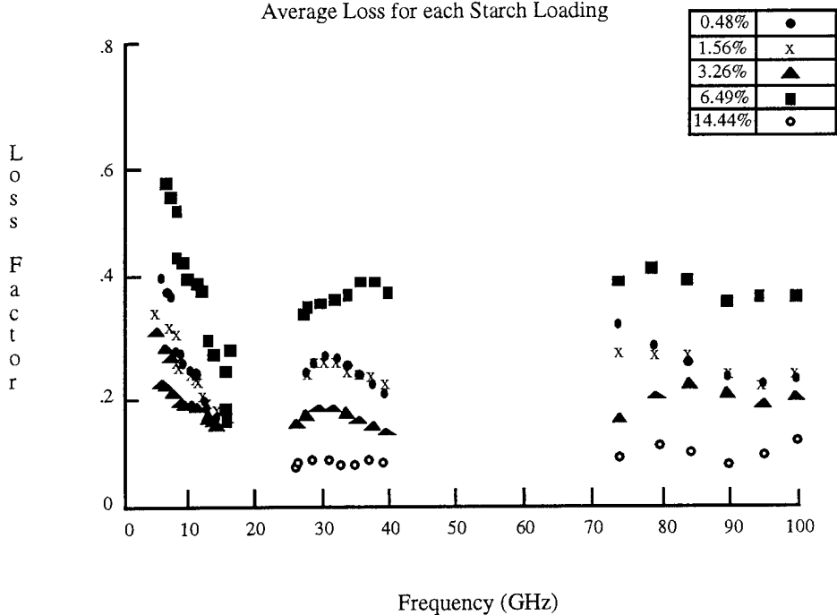
Figure 11. Loss Factors — Initial Starch Iodine Compounds
