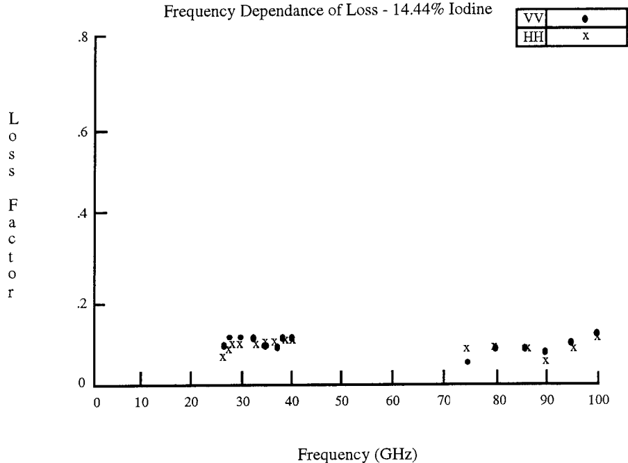
Figure 10. Loss Factor - 14.44% Iodine
