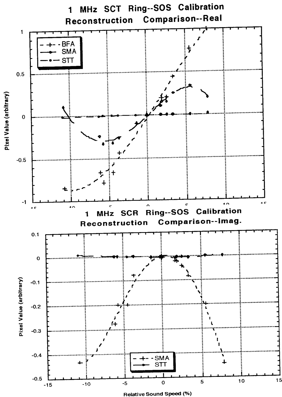
Figure 10. Speed of Sound and Attenuation Contrast Sensitivity for 1 MHz SCT Ring for Three Reconstruction Algorithms. Top: Speed of Sound (Real). Bottom: Attenuation (Imaginary).
