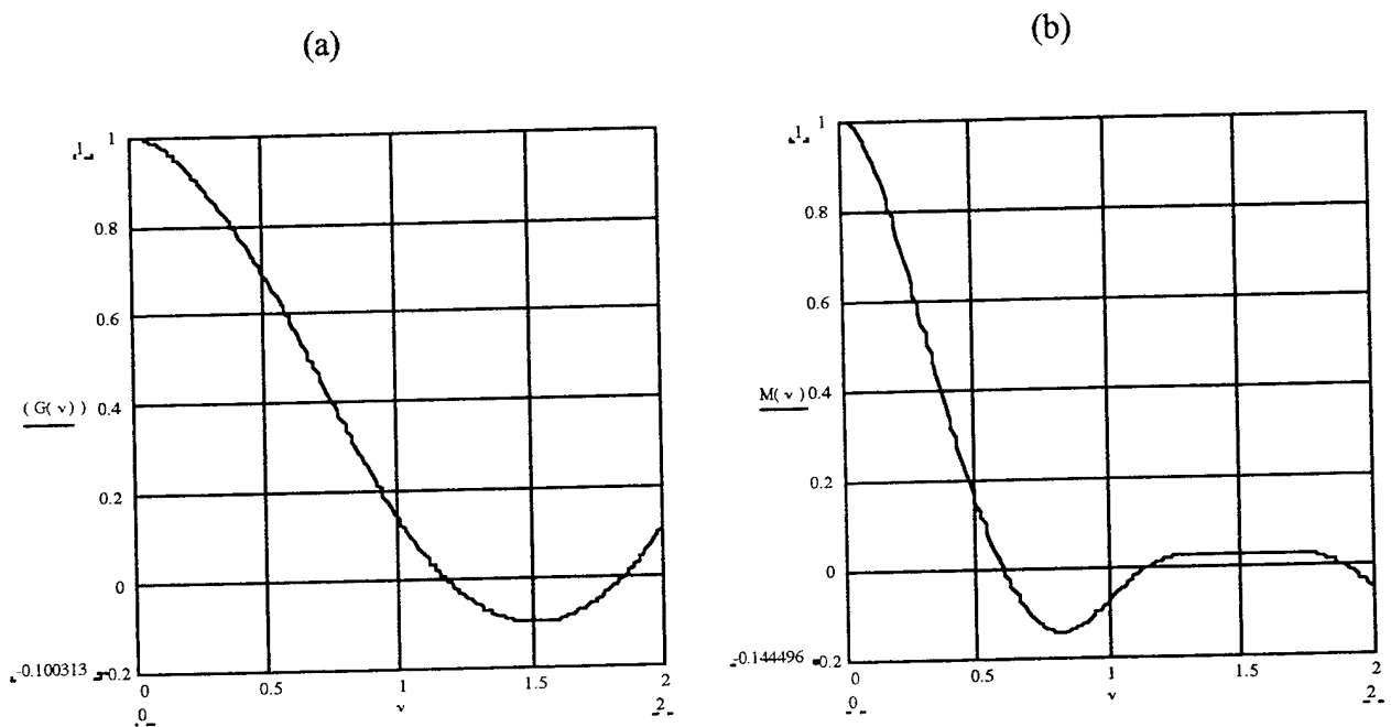
Figure 8. MTF of 1 MHz SCT Ring. First Order Born Magnitude Reconstruction. Object was 120 \mu\text{m} dia. Nylon Filament (a) in Water, (b) inside 2.75 in. dia. Balloon Filled with Saline Solution with Speed of Sound 4.7% Higher than Water.
