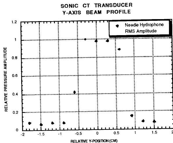
Figure 7. Slice Profile for 1 MHz SCT Ring.
