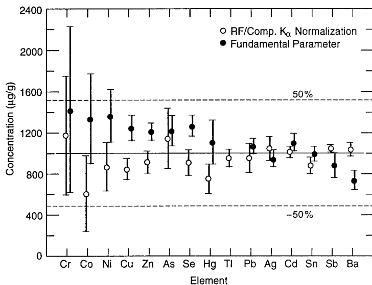
Figure 5. Average and standard deviation of concentrations established for soils spiked with 1000 µg metal/g, as determined by RF/Comp. K α normalization and FP analysis.
