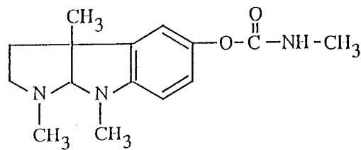
Physostigmine
