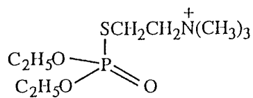
Echothiophate
