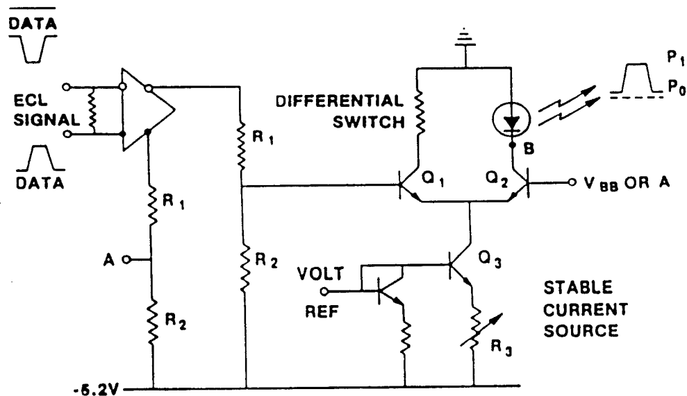
Figure 4-3 Schematic of the Direct Current Modulator Circuit
