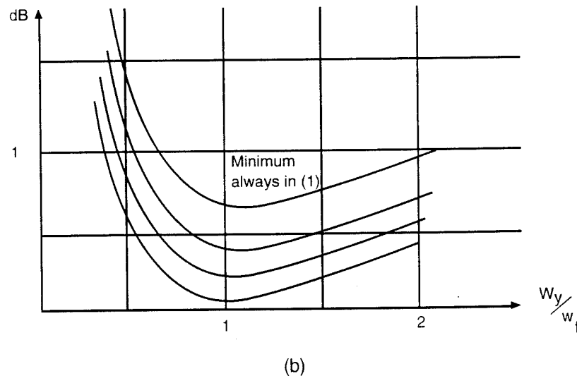
Figure 2-6 (a) Approximate Single-Mode Fiber/Waveguide Coupling Loss (Excluding Fresnel Loss) as a Function of Laser Mode Spot Size, W_f , Horizontal Waveguide Mode Spot Size, W_x , and Vertical Waveguide Mode Spot Size, W_y . (b) Blow up of the minimum loss which deviates around 1.
