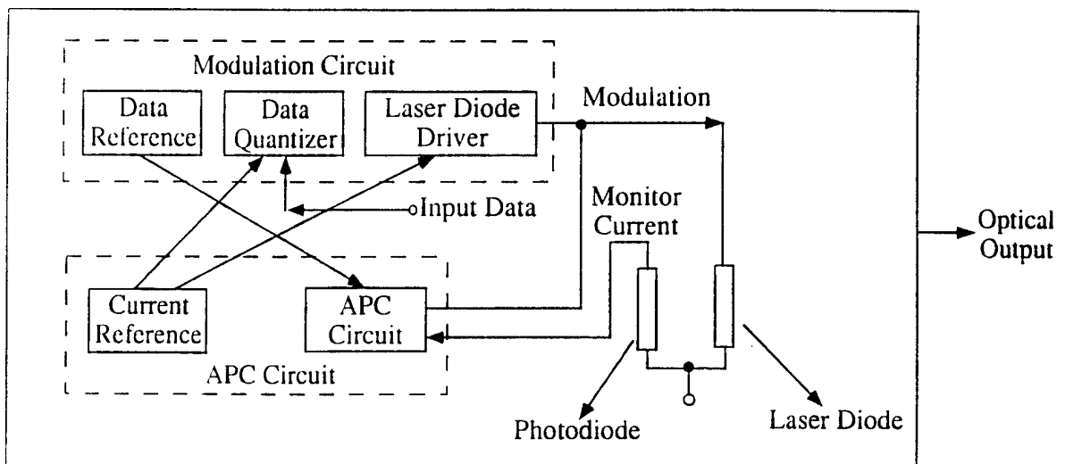
Figure 4-14 Block Diagram of the Transmitter
