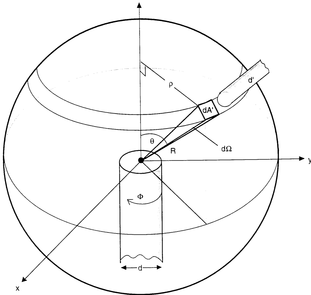
Figure 2-1 Illustration of Fiber-to-Fiber Coupling Geometry. d is the diameter of the input fiber, d' is the diameter of the output fiber, (\theta, \phi) are the spherical angles, R is the fiber-to-fiber distance, d\Omega is the solid angle element, and \rho = R \sin \theta .
