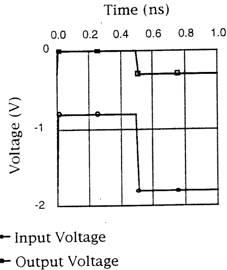
Figure 4-10 Input and Output Voltage Levels (ECL) For the Pure Resistor Model
