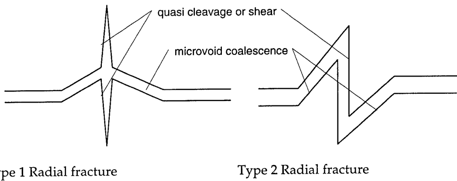
Figure 2. Detail of two types of radial fracture, after Larson and Carr [13]
