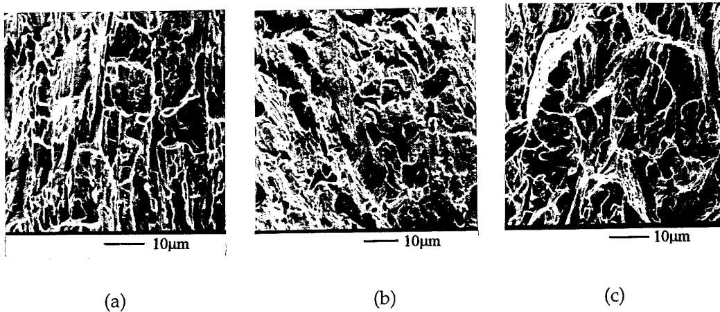
Figure 11. Fracture surfaces of longitudinal splits from BIS 812 EMA plain tensile specimens. Scanning electron micrographs.
