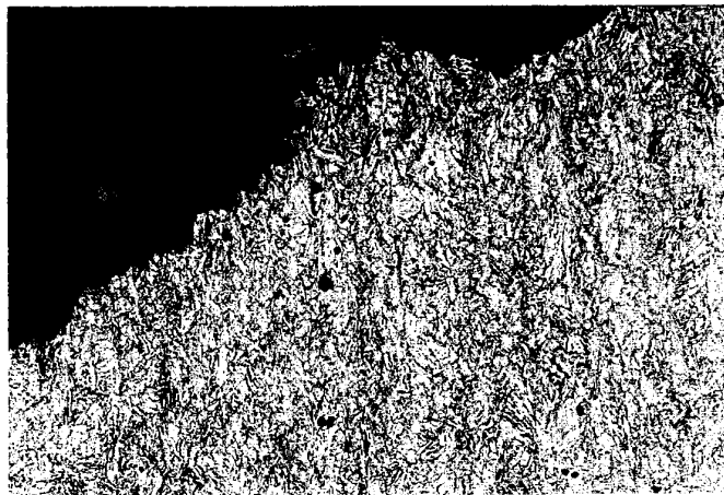
Figure 17. Void formation within the fibrous region of the neck in a notched tensile specimen of BIS 812 EMA steel tested at room temperature. (x100)
