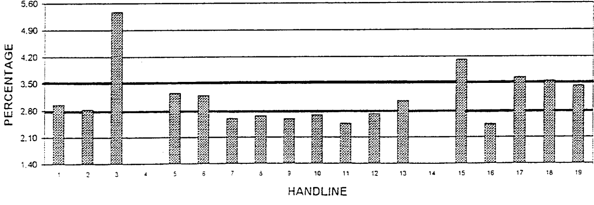
Figure 2 3% AFFF Performance Target Range 2.8 - 3.5%
