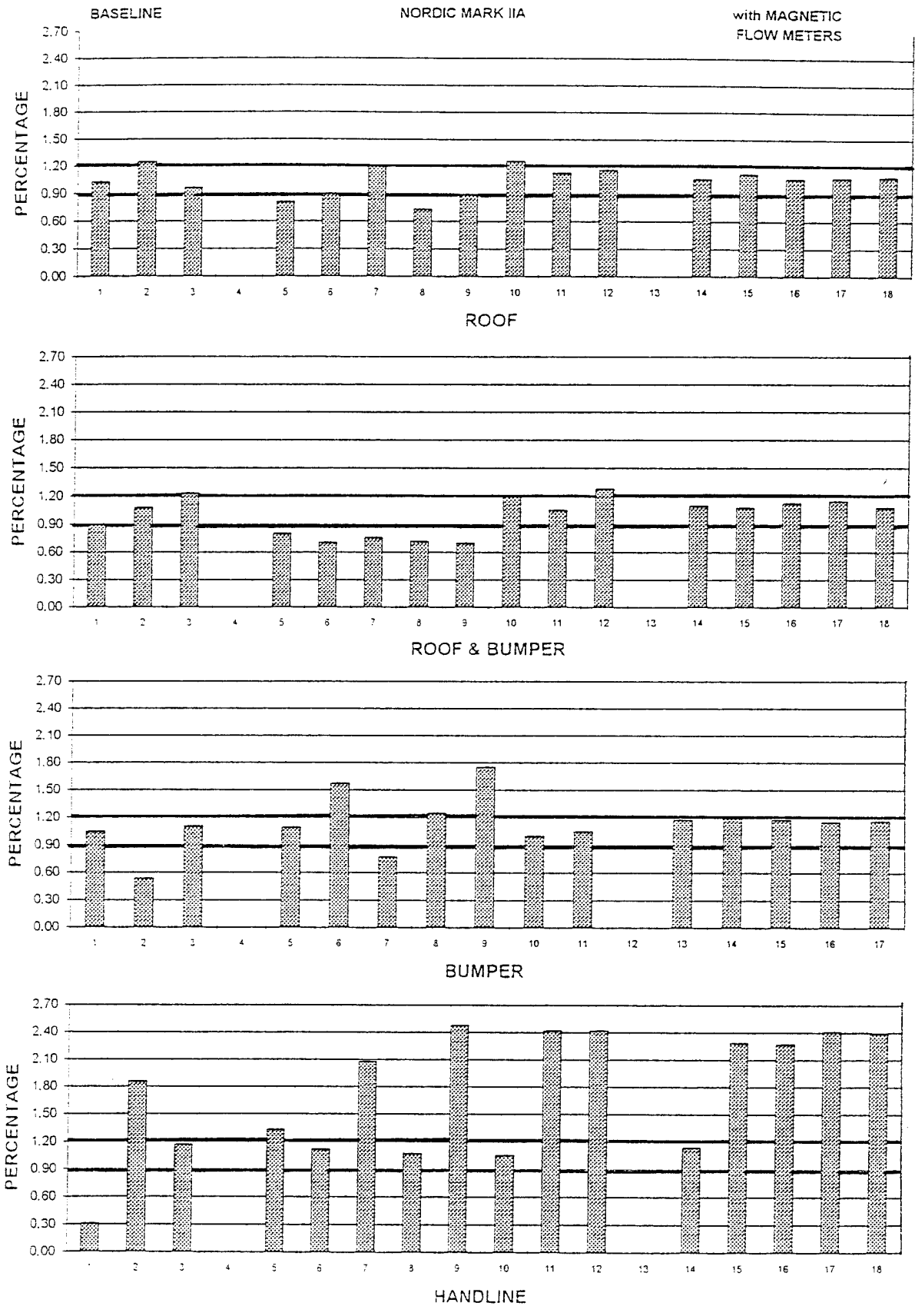
Figure 1 1% AFFF Performance Target Range 0.9 - 1.2%
