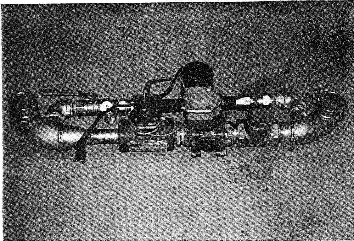
Photo 3 NORDIC Mark IIA Computerized Foam Proportioning System Valves and Plumbing
