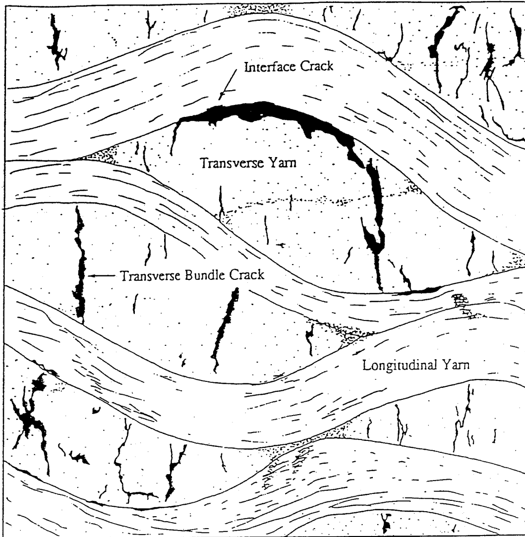
Figure 2. A schematic illustration of the typical damages found in an as-processed ORCC substrate material.
