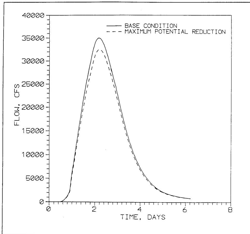
Figure 2. 100-year-event hydrographs for West Fork Cedar River
