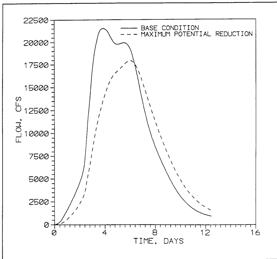
Figure 3. 100-year-event hydrographs for the Redwood River
