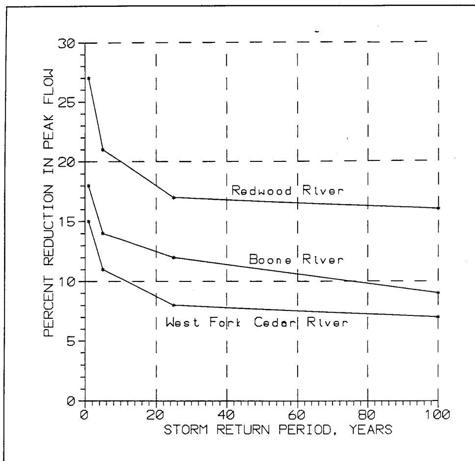
Figure 4. Percent peak flow reduction versus storm return period for maximum infiltration and storage alternatives
