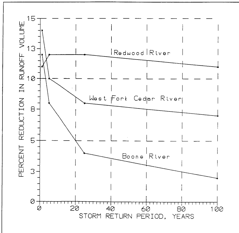
Figure 5. Percent runoff volume reduction versus storm return period for maximum infiltration and storage alternatives
