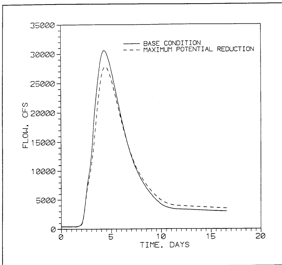
Figure 1. 100-year-event hydrographs for the Boone River
