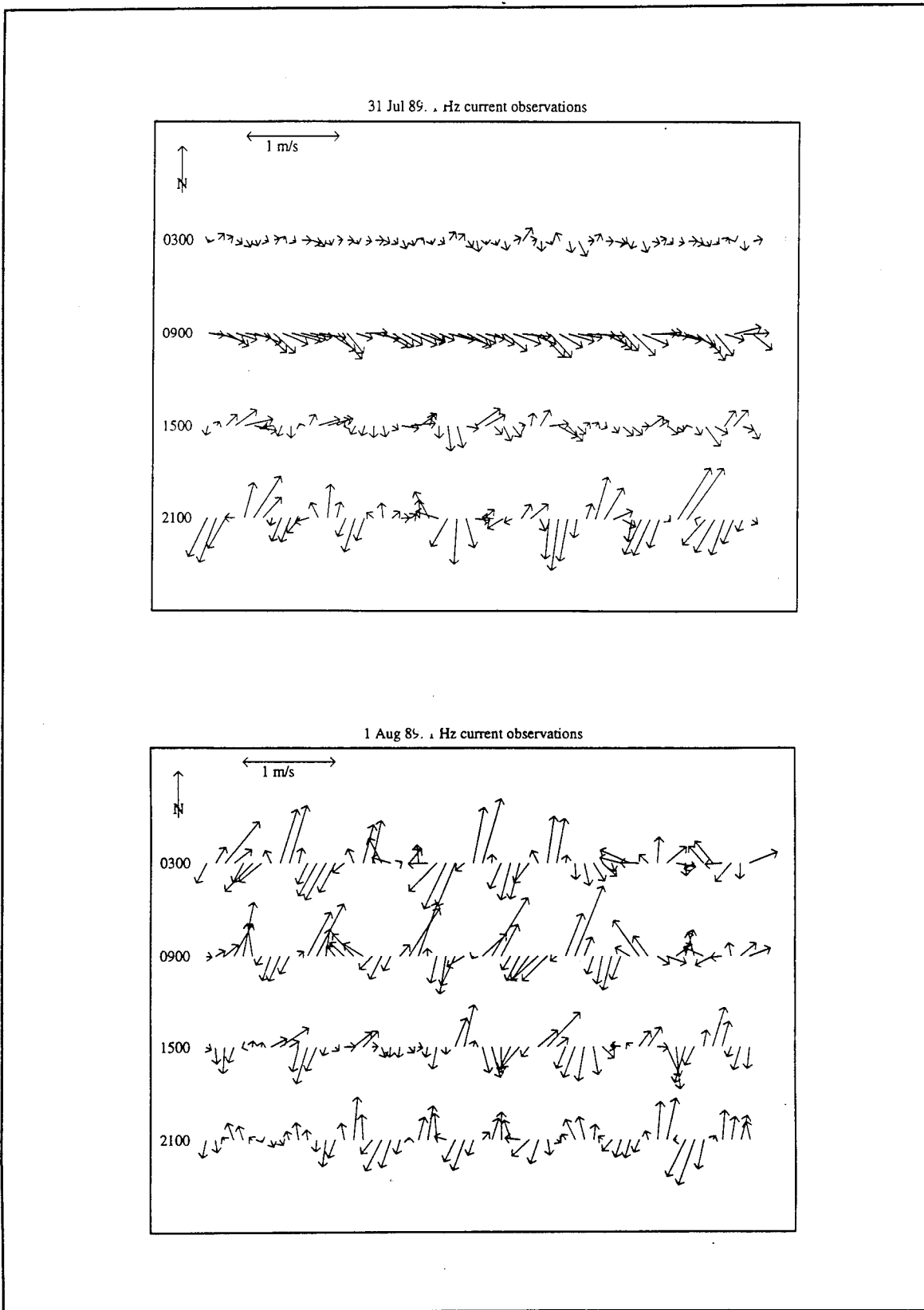
Figure 15. Instantaneous current vectors measured at 1 Hz during passage of Hurricane Chantal (Continued)
