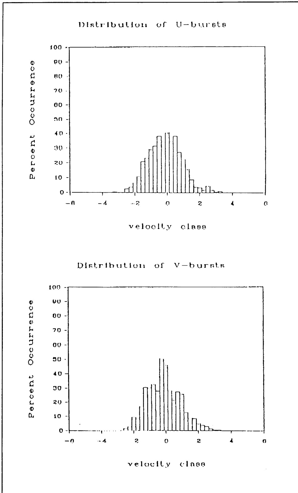
Figure 5. Distributions of standardized velocity components (dimensionless) during a typical "burst"
