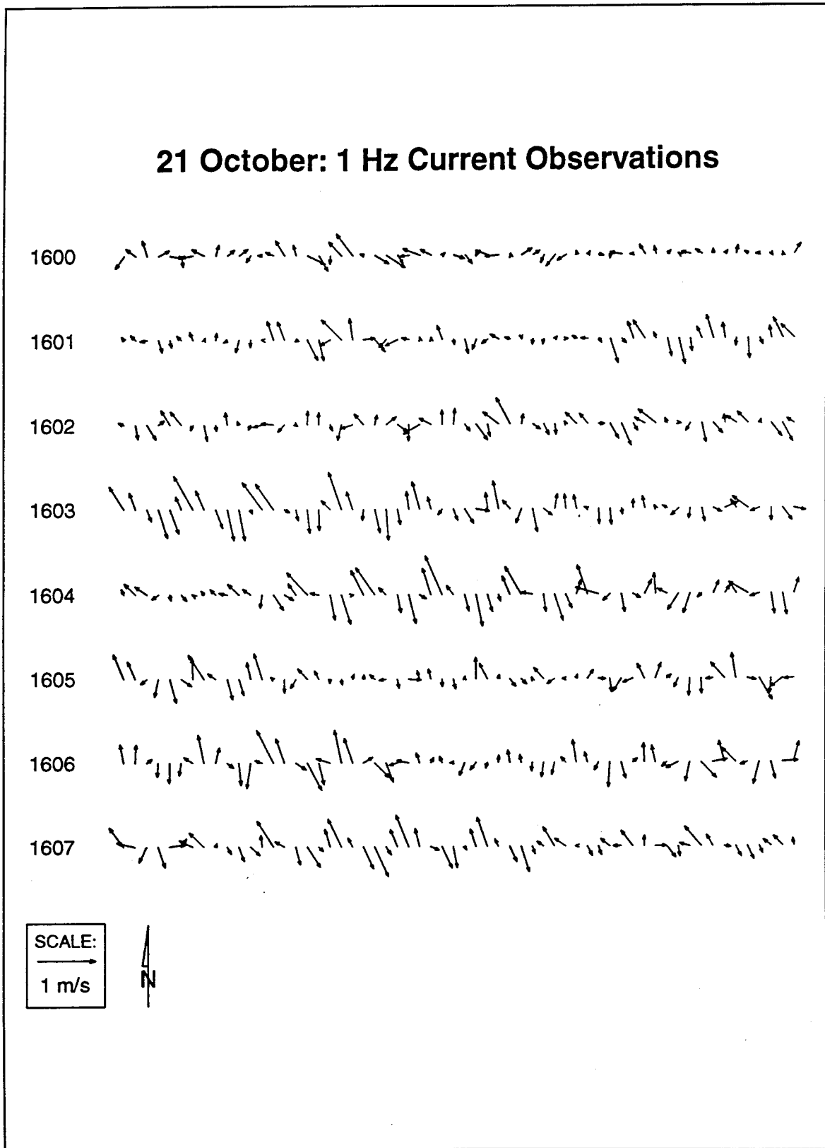
Figure 18. Instantaneous current vectors measured at 1 Hz at 1600-1607 on 21 October 1990 (southerly wind sea)
