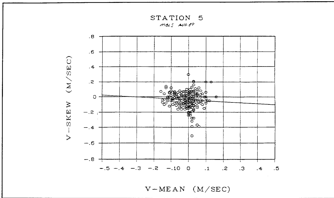
Figure 8. Joint distribution of mean v and \sigma_v at site PUVSI-5 (on-mound)
