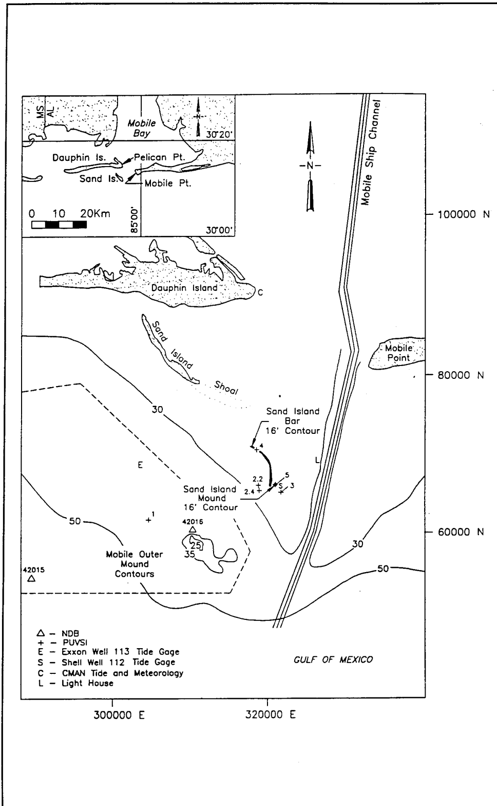
Figure 1. Location of constructed submerged features and gauges (from Hands and Allison (1991))
