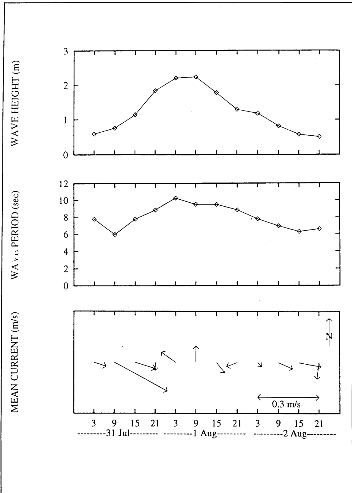
Figure 14. Wave and mean current conditions during passage of Hurricane Chantal
