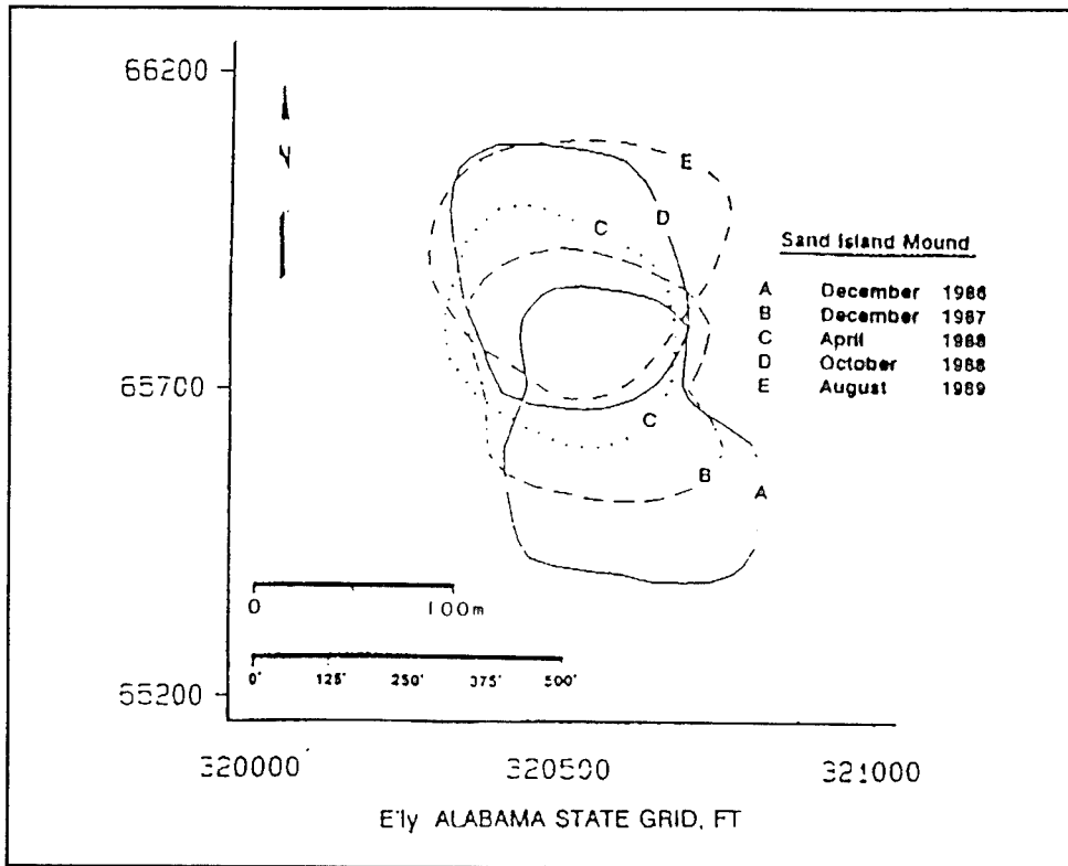
Figure 2. Migration of Sand Island Mound (from Hands and Allison (1991))
