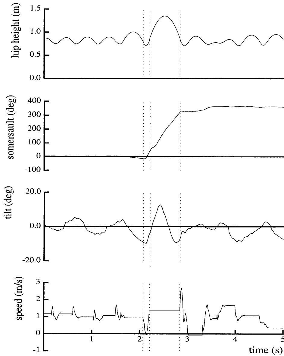
Figure 4-5: Hip height, somersault, and tilt angles, and forward speed of the 3D-Biped during a somersault. Vertical lines indicate initiation of flip, lift-off and landing. Data file B92.181.3
