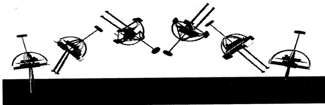
Figure 6-10: Sequence of images of the simulated 3D Biped somersault with twist.
